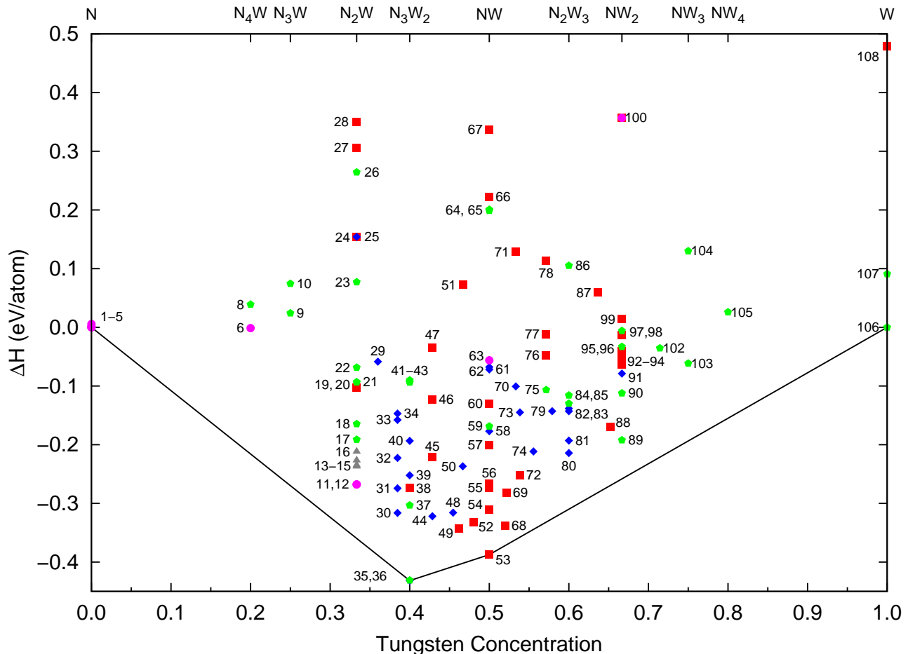
FIG. 2: (Color online) The relative enthalpy (1) of N_{1-x}W_x for the 108 structures listed in the supplementary material plotted versus increasing tungsten concentration. These points were calculated using the Perdew-Burke-Ernzerhof (PBE) functional with VASP. Note that the enthalpy of structure #7 is above the upper limit of the graph. The meaning of the symbols is described in the caption to Figure 1.
