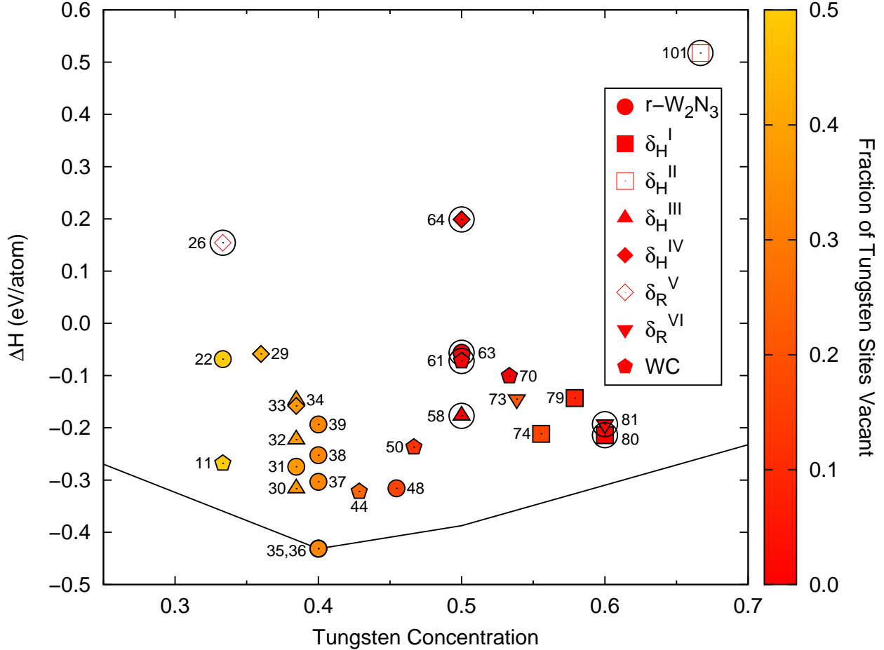
FIG. 9: (Color online) Enthalpy per atom for various crystal structures approximating the \delta -phases of Khitrova and Pinkser 18,19 and Wang, Yu, Lin al. (WYL+) 21 . All calculations were done using the PBE functional. The legend describes the six structures found by Khitrova and Pinksler, as well as the “ r - W_2N_3 ” structure of WYL+. We also include the tungsten carbide (WC) structure and some derivatives. 25,48 The actual structures are labeled according to the indexing in the supplementary material. The circled structures are the parent structures, which have fully occupied tungsten sites. For the other structures the tungsten vacancy concentration is indicated by the point shading. Red (dark) shaded structures have no or few defects, while orange-yellow (light) shading indicates a larger concentration of vacancies, up to 50%. Note that some tungsten planes have no vacancies, while other planes can have as many as 2/3 of the sites vacant. See Figure 10 for an example. The \delta_H^I and \delta_H^V structures have no vacancy sites, therefore the parent is the only structure we studied and its special status is shown by having no coloring to the data point.
