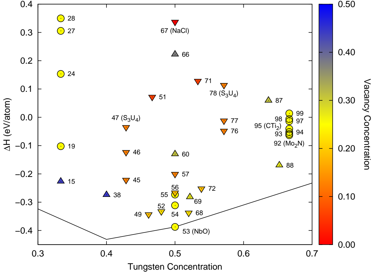
FIG. 8: (Color online) A section of Figure 2 showing only structures created by removing atoms from supercells of the NaCl structure. Yellow circles denote structures where 25% of the sites on the NaCl lattice are empty. Downward pointing triangles have fewer than 25% of the sites vacant, and the redder triangles have fewer vacancies, culminating in the NaCl structure (#67). Upward pointing triangles have more than 25% of the sites vacant, and are bluer as more sites become vacant. Known experimental structures are labeled by their prototype name.
