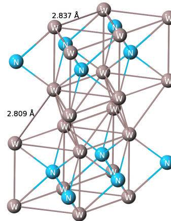
FIG. 16: (Color online) NW 2 in the hexagonal MoS 2 structure, 100 #89 in the supplementary materials. Unlike MoS 2 , the interplanar W-W distance is smaller than the in-plane W-W distance.
