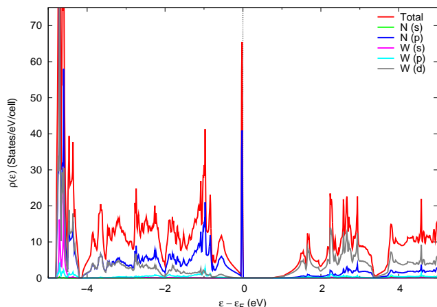
FIG. 15: (Color online) The electronic total, and angular momentum decomposed, density of states for N 2 W in the SiO 2 -like cI36 structure (#15), using the vdW-DF2 functional and the tetrahedron method within VASP. We truncated the plot at 75 states/eV/cell in order to show the behavior of the system near the top of the valence band. The density of states at the bottom of the valence band approaches 200 states/eV/cell.
