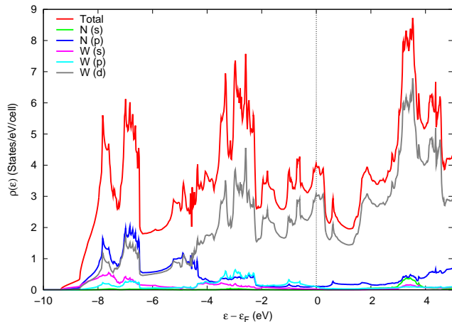
FIG. 18: (Color online) The electronic total, and angular momentum decomposed, density of states for NW_2 in the hexagonal MoS_2 structure 100,101 (#89 in the supplementary material), using the PBE functional.
