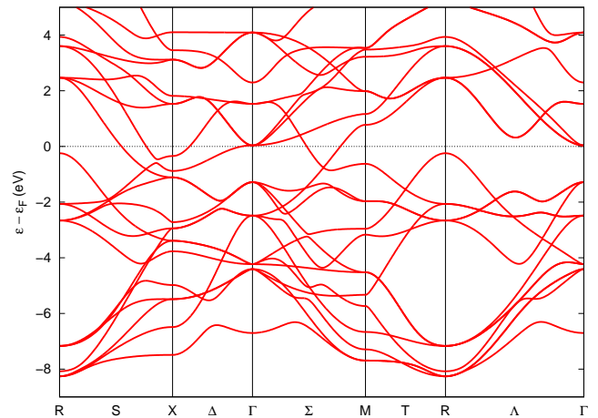
FIG. 6: The electronic band structure of tungsten nitride in the NbO structure (#53) at the PBE equilibrium ( a = 4.131\text{Å} ). The high symmetry points and lines are described in the supplementary material.
