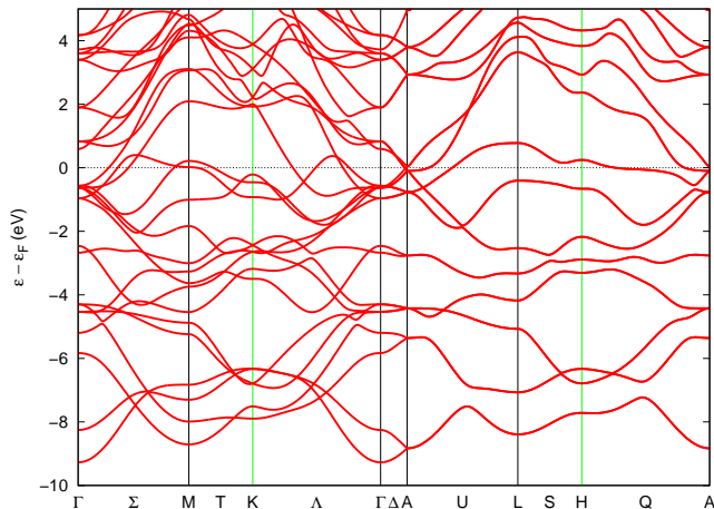
FIG. 17: (Color online) The electronic band structure for NW_2 in the hexagonal MoS_2 structure 100,101 (#89 in the supplementary material), using the PBE functional.
