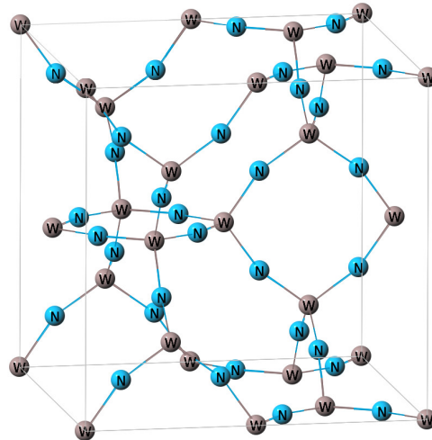
FIG. 13: (Color online) The \text{SiO}_2 -like cI36 structure (#15 in the supplementary material) predicted as the ground state of \text{N}_2\text{W} by the vdW-DF2 functional. The basic structure looks the same using LDA, PBE, and vdW-DF2 functionals. The exact dimensions are described in Table VI. Note that this is a body-centered cubic lattice, so the center of the cube and the cube corners are equivalent sites. The inversion sites are at the centers of the eight-atom rings, not on the tungsten atoms.
