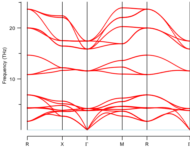
FIG. 5: (Color Online) Phonon frequencies along high-symmetry lines for the NbO structure (#53) of tungsten nitride, found with the MedeA ® package. 78 No imaginary phonon frequencies were found, indicating that this structure is stable against small amplitude vibrations. The high symmetry points and lines are described in the supplementary material.
