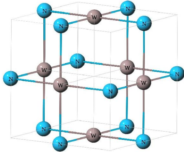
FIG. 4: (Color Online) Tungsten nitride in the NbO structure, 67 (#53 in the supplementary material) constructed by taking equally spaced vacancies from both sites of the NaCl structure. The PBE functional predicts the equilibrium lattice constant to be 4.131Å.
