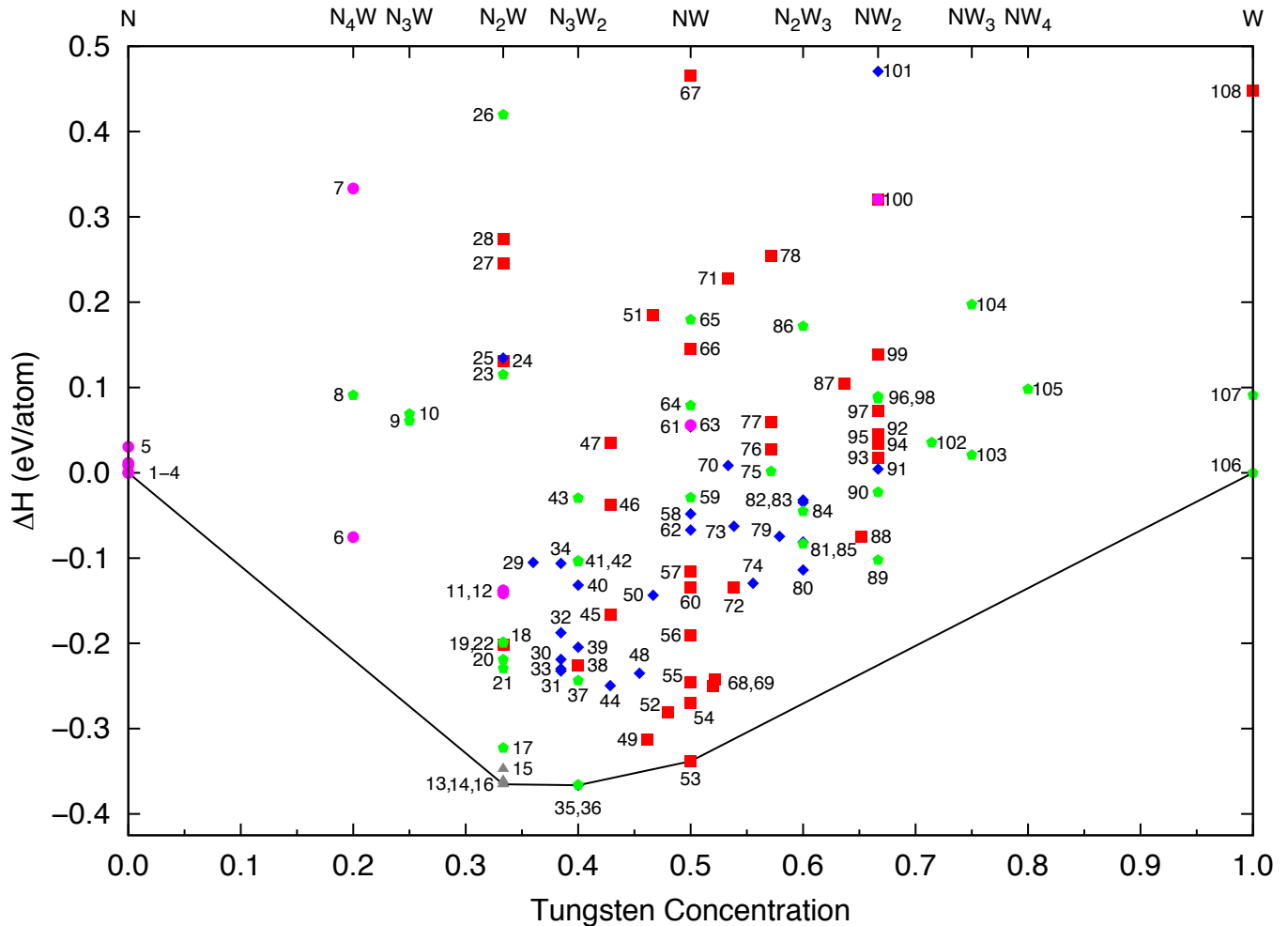
FIG. 3: The relative enthalpy (1) of N_{1-x}W_x for the 108 structures listed in the supplementary material plotted versus increasing tungsten concentration. These points were calculated using the van der Waals vdW-DF2 van der Waals functional with VASP. The meaning of the symbols is described in the caption to Figure 1.
