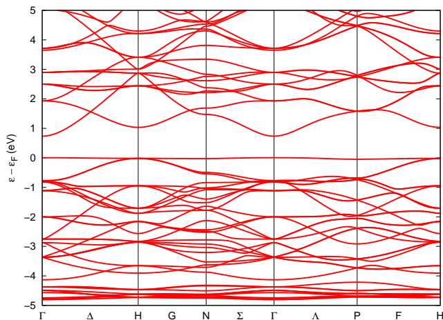
FIG. 14: The electronic band structure for the SiO 2 -like body-centered cubic cI36 structure (#15) of N 2 W described in the text. Calculations were done using the vdW-DF2 functional, including van der Waals forces, within VASP. The top valence band has a very small dispersion, dropping to -0.05 eV below the top of the valence band at P. The gap is 0.75 eV, and is direct at \Gamma . The LDA and PBE calculations produce similar band structures.
