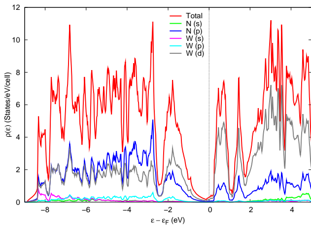
FIG. 12: (Color online) The electronic density of states for structure #35, one of our approximations to the “ r - W_2N_3 ” structure, 21 using the PBE functional and the tetrahedron method. Note that the angular momentum decomposed densities of states are summed over all atoms of the same type, even if they have different crystallographic positions.
