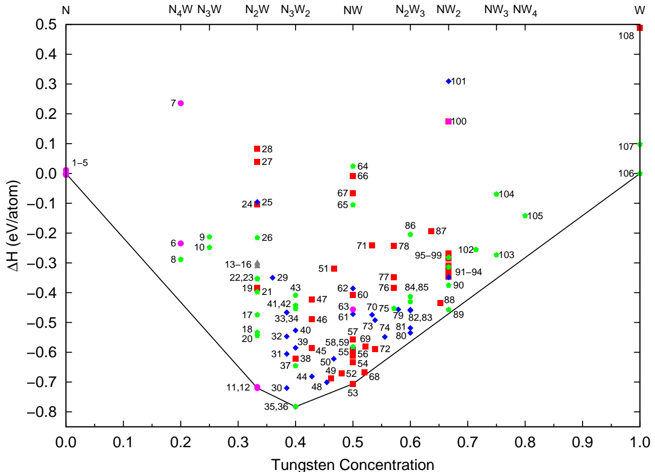
FIG. 1: (Color online) The relative enthalpy (1) of N_{1-x}W_x for the 108 structures listed in the supplementary material plotted versus increasing tungsten concentration. These points were calculated using the Local Density Approximation (LDA) with VASP. Red squares mark the \beta phase structures, dark blue diamonds the \delta phases, purple circles the N_2 (nitrogen dimer) phases, gray triangles the SiO_2 phases, and green pentagons the remaining miscellaneous phases. The labels correspond to the numbers of the structures in the supplementary material.
