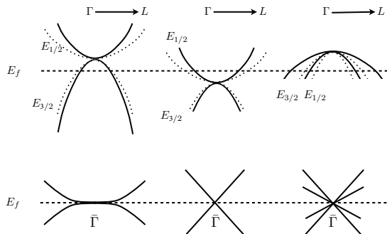
FIG. 2: Three possible scenarios for the Fermi level crossing the bulk \Gamma_8 -bands and the schematic dispersions of the surface states [from left to right: case-(ii), -(i) and -(iii)]. Solid and dotted lines mean that the corresponding band of has positive and negative pairing amplitude, respectively, in the nontrivial superconducting phase. See Ref.[41] for a discussion of the case of degenerate bands in the presence of inversion.
