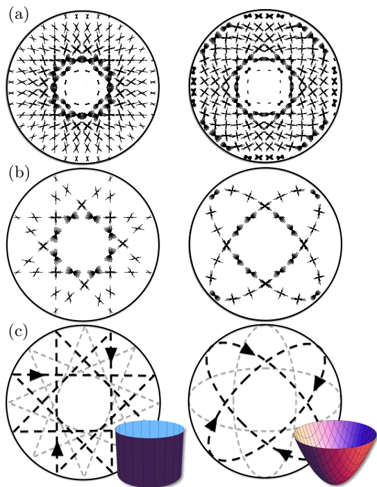
FIG. 14: Quantum-classical correspondence from Husimi maps by sampling along classical trajectories. In part (a), the Husimi map for the two eigenstates in Fig. 2c-d, where Husimi projections are sampled along a grid. In part (b), projections are instead sampled along classical paths that correspond to the wavefunction. Because of rotational symmetry, however, the wavefunction is actually created by the sum of many rotations of such paths, as indicated in part (c).
