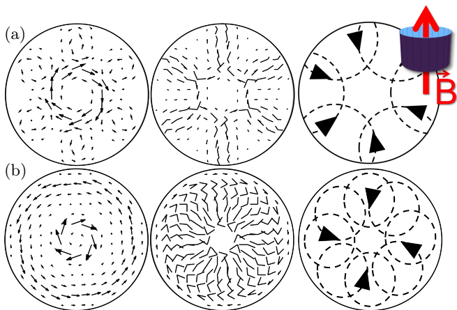
FIG. 4: Maps of the flow for the two states presented in Fig. 3(a-b). (left) the flux map, (center) the processed Husimi map, and (right) classical paths. The traditional flux correlates strongly with Husimi flux (Eq. 3) but fails to show the classical paths suggested by the wavefunction.
