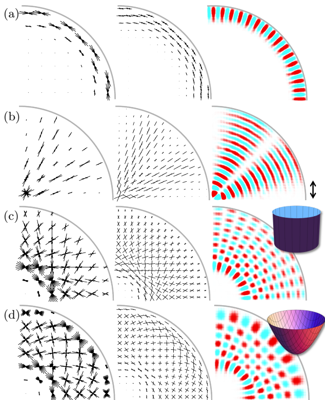
FIG. 2: Raw Husimi maps (left), processed Husimi Maps (middle), and the wavefunction (right) for eigenstates of the circular well (a-c) and the harmonic oscillator (d). Double-arrows at far right indicate the spread of the coherent state ( \Delta k/k = 10\% ). The states in (c) and (d) correspond to the classical paths in Figs. 14a and b respectively.
