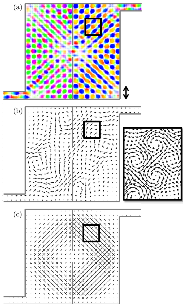
FIG. 10: A scattering wavefunction associated with full transmission through a partially obstructed square device. (a) Wavefunction of the system, (b) the Husimi flux, and (c) the processed Husimi map. The coherent state spread used is \Delta k/k = 10\% , indicated by the double arrows. The inset shows the traditional flux over the part of the system indicated by the black squares.
