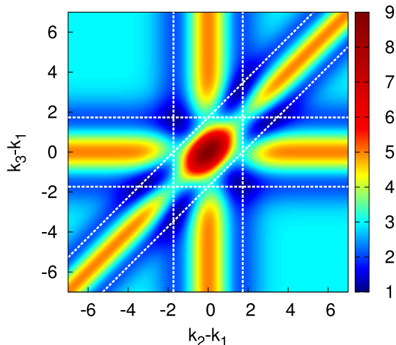
FIG. 13: Uncertainty obtained by summing three vectors of a Husimi projection, as written in Eq. A3. The uncertainty is bounded above by 9/4\sigma^2 and below by \sim 1.017/4\sigma^2 . The dashed white lines indicate local minima that result from spacing each pair of vectors by \sqrt{3}/\sigma , which would give a minimum uncertainty for two-vector addition (see Fig. 12).
