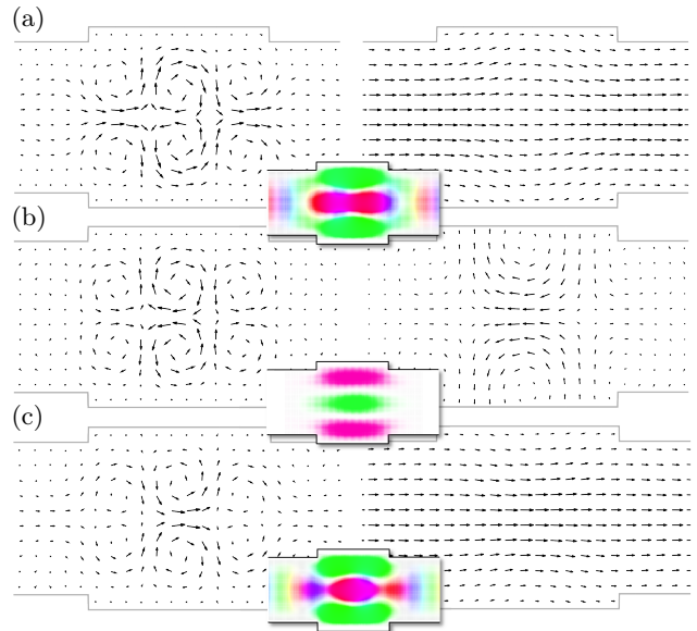
FIG. 9: The traditional flux (left column) and the Husimi flux (right column) for the resonance state in Fig. 6 slightly above resonance (a, E = E_{\text{res.}} + 0.00005 ), at resonance (b, E = E_{\text{res.}} ) and slightly below resonance (c, E = E_{\text{res.}} - 0.00005 ). The coherent state for the Husimi flux corresponds to \Delta k/k = 0.2 . The transmission function for this mode corresponds to (a) T = 0.99 , (b) 0.06, and (c) 0.99 for the respective energies. Even though the raw Husimi maps (not shown) at each energy are indistinguishable from Fig. 7, their vector additions (Husimi flux) vary substantially. Energies are in arbitrary units, scaled to Fig. 6.
