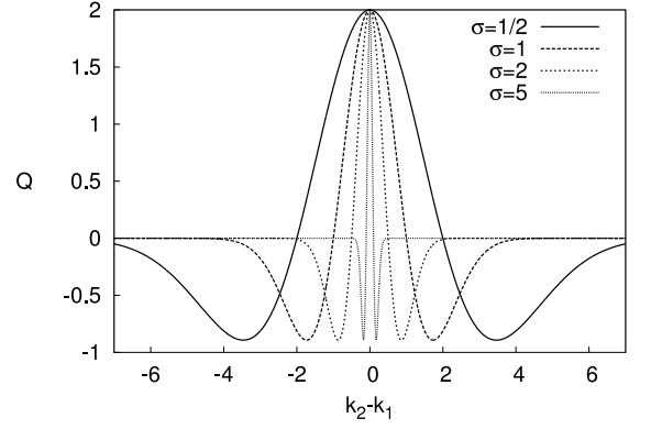
FIG. 12: The second term in Eq. A3 is plotted for the addition of two vectors in the Husimi projection. This term represents the covariance between the two vectors, and is bounded above by 2 and below by -\frac{4}{e^{3/2}} for all choices of \sigma .
