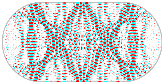
FIG. 1: A scarred eigenstate of the stadium billiard reveals the strong influence of periodic classical orbits. The traditional flux provides no information: it is uniformly zero inside the billiard.
