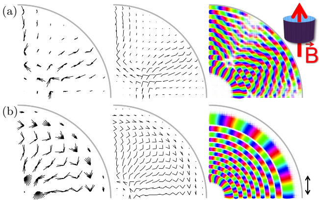
FIG. 3: Raw Husimi map (left), processed Husimi maps (middle), and wave function (right) for two eigenstates of the circular well with magnetic field coming out of the plane. The magnetic field strength is set so that the cyclotron radius is approximately 1/2 (a) and 1/3 (b) the radius of the system. Double-arrows at far right indicate the spread of the coherent state ( \Delta k/k = 10\% ). Both states correspond to the classical paths presented in Fig. 4.
