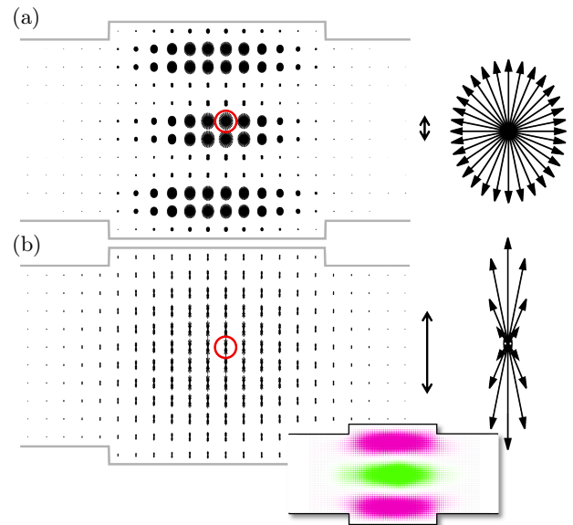
FIG. 7: The raw Husimi map for the resonant state (see inset) is plotted using (a) \Delta k/k = 100\% and (b) \Delta k/k = 20\% . The spread of the test wave packet is indicated by the respective double-arrows. A single Husimi projection (circled in red) for each map is magnified at right. The vector sums of each map are shown in Figs. 9b.
