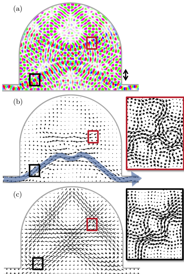
FIG. 11: A scattering wavefunction associated with full transmission through the half-stadium. (a) Wave function representation, (b) the Husimi flux, and (c) the processed Husimi map. The coherent state spread used is \Delta k/k = 10\% , indicated by the double arrows. Black and red squares highlight regions of particular interest (see text). The traditional flux from the respective highlighted regions of the system is shown magnified in the insets.
