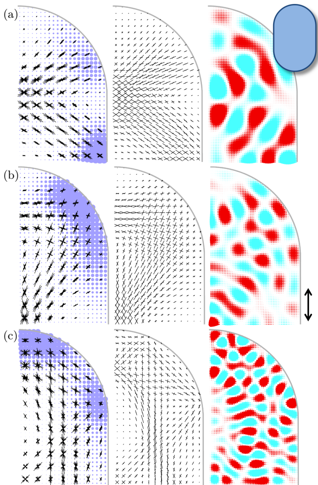
FIG. 5: Eigenstates of the stadium billiard system with Dirichlet boundary conditions at three increasing energies, with the raw Husimi map (left), processed Husimi map (middle) and wavefunction (right). Angular deflection is indicated in blue in the left column. Double arrows indicate the spread of the coherent state used in the calculations ( \Delta k/k = 20\% (a), 15\% (b) and 10\% (c)).
