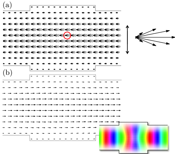
FIG. 8: (a) The raw Husimi map for the wave function of the lowest propagating mode (see inset) of the waveguide in Fig. 6. The energy of the state is well above resonance ( E = 0.02745 ). The uncertainty for this map is \Delta k/k = 20\% . A magnified view of the projection circled in red is presented at right. (b) The Husimi flux. This is the mode which hybridizes with the resonant state to produce Figs. 7 and 9.
