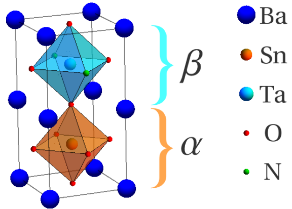
FIG. 1: Unit cell of the \alpha\beta structure. The cubic perovskite planes are stacked in the z -direction while x - and y -direction maintain the usual periodicity of a cubic perovskite. \alpha indicates the BaSnO 3 perovskite, and \beta the BaTaO 2 N.
