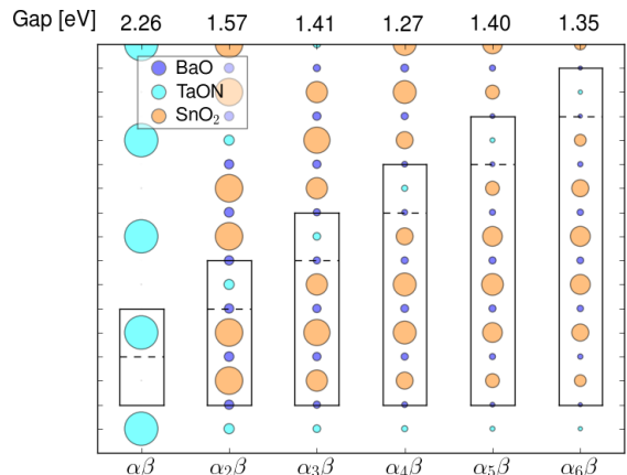
FIG. 7: Weight of the CBM-state in each xy -plane of the n_\beta = 1 structure. The character of the CBM-state changes drastically with n_\alpha : TaON is responsible for the CBM-state for the n_\alpha = 1 structure, while for n_\alpha > 1 it is SnO_2 (Figs. 4b and 4d). The tunneling across the TaON plane has an effect until n_\alpha = 4 .
