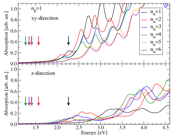
FIG. 9: Calculated optical absorption for the n_\beta = 1 systems. The direct band gaps are indicated with vertical arrows.
