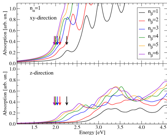
FIG. 8: Calculated optical absorption for the n_\alpha = 1 systems. The direct band gaps are indicated with vertical arrows.
