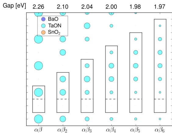
FIG. 5: The figure illustrates the weights of the CBM-state in real space. The vertical axes of the figure is along the stacking direction of the material and the areas of the circles indicate the weights of the CBM-state for a particular atomic xy -plane. The boxes show the extent of the supercell in the direction of the stacking ( z ), and the dashed lines mark the interfaces between the alpha and beta layers. Above the figure the calculated band gaps for the different stacking sequences are denoted. The CBM-state is mainly composed of Ta d -orbitals, as shown in Figure 4b.
