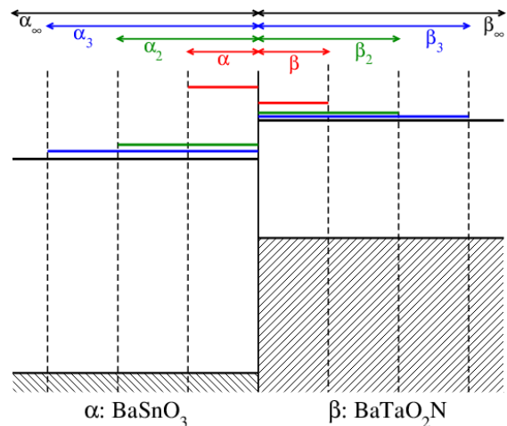
FIG. 3: Sketch of the electronic level positions at an interface between layers of BaSnO 3 and BaTaO 2 N. When the layer thickness is reduced the local position of the conduction band edge moves up due to confinement.
