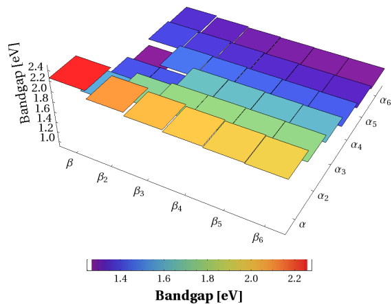
FIG. 2: Calculated band gaps as a function of the number of \alpha (BaSnO 3 ) and \beta (BaTaO 2 N) layers. Each rectangle in the plot represents a layered periodic structure with sequence \alpha_n\beta_m .
