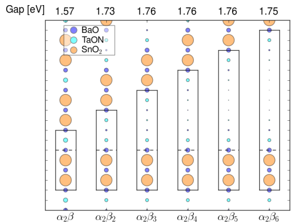
FIG. 6: Weight of the CBM-state in each xy -plane of the n_\alpha = 2 structure. The CBM-state is now composed of Sn s -states, with some tunneling through the TaON plane (Fig 4d). The tunneling progressively reduces with the increase of \beta -layers.
