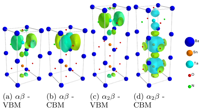
FIG. 4: Wave functions of states at the valence band maximum (VBM) and the conduction band minimum (CBM) for some combinations of \alpha and \beta layers.
