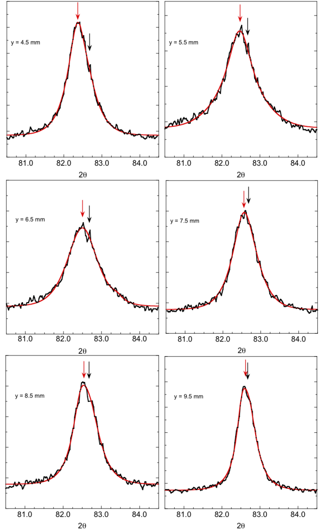
FIG. 12. (Color online) X-ray diffraction data for the \text{YBa}_2\text{Cu}_3\text{O}_{\nabla x} film. Fits to the \langle 00 10 \rangle peak for y = 4.5 mm - 9.5 mm. The red arrow indicates the maximum of the curve fit. The black arrow indicates a spurious substrate peak (which does not undergo change in 2\theta as the oxygen content of the \text{YBa}_2\text{Cu}_3\text{O}_{\nabla x} film does).
