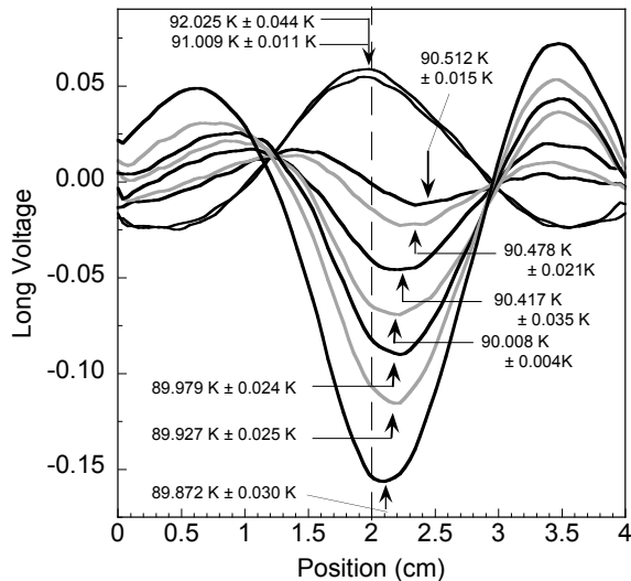
FIG. 2. Voltage signal response of the SQUID magnetometer for the longitudinal magnetic moment of the \text{YBa}_2\text{Cu}_3\text{O}_{\nabla x} sample at temperatures in the vicinity of the superconducting transition. The values of the temperature shown are the mean of the beginning and end temperature recorded by the MPMS for each scan. The error value indicates the range of the temperature during the scan. The arrows indicate the center position of the voltage response as determined by a curve fit. These positions are shown as open circle symbols in Fig. 3b.
