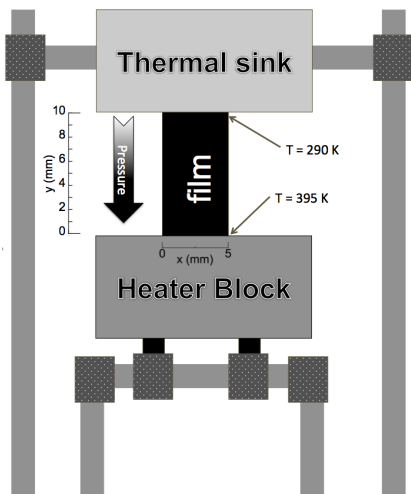
FIG. 1. Schematic of the apparatus used to produce the \text{YBa}_2\text{Cu}_3\text{O}_{\nabla x} film. The y(\text{mm}) scale shown corresponds to the sample orientation shown in Fig. 7b below.
