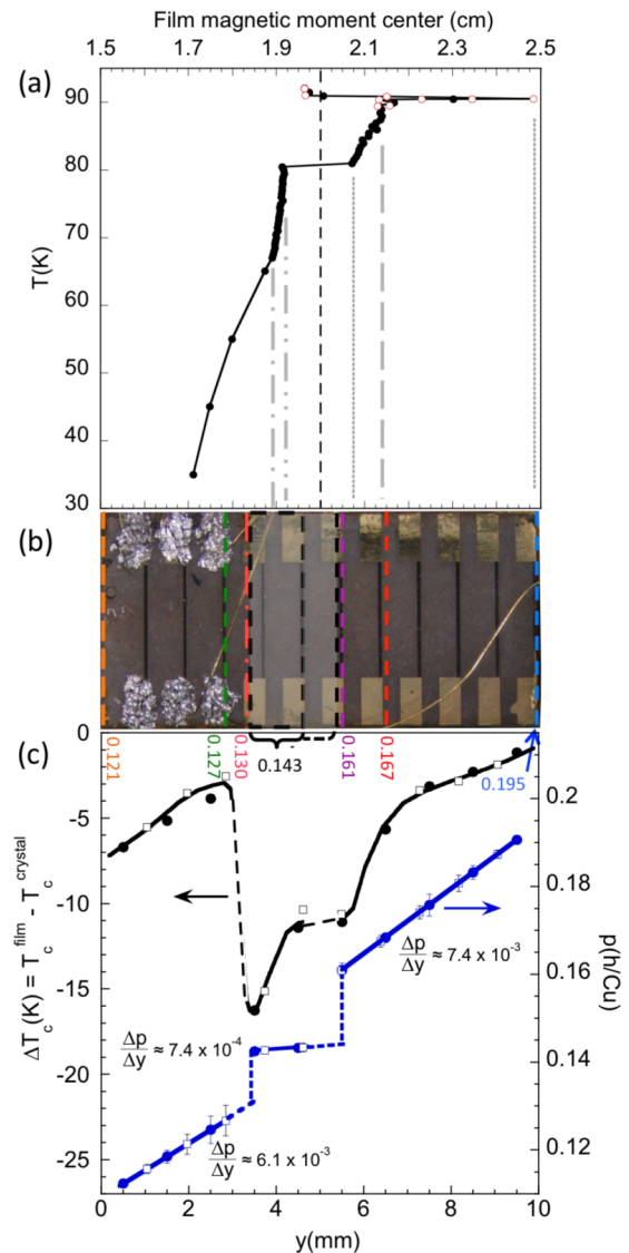
FIG. 7. (Color online) (a) Center of the longitudinal magnetic moment of the \text{YBa}_2\text{Cu}_3\text{O}_{\nabla x} sample with respect to the sample position y(\text{mm}) . The M(T) scan of sample was taken prior to lithographic etching. (b) \text{YBa}_2\text{Cu}_3\text{O}_{\nabla x} sample after it has been patterned for R(T) measurements. The colored regions indicate values of hole doping inferred from the x-ray data using the relationship the c-axis length and p established in Ref. [9] with the same coloring scheme used in Fig. 5. Note the grey shaded region in the interval 3.4 \text{ mm} \lesssim y \lesssim 5.6 \text{ mm} with p = 0.143 \approx 1/7 . The solid black bracket indicates the region determined from x-ray and R(T) measurements. The dashed extension of the bracket is inferred from M(T) data. The orange dashed line with p = 0.130 indicates the inferred doping by linearly extending the p(y) dependence of the highly underdoped region. (c) \Delta T_c vs. sample position y(\text{mm}) , and hole concentration vs. sample position p vs. y(\text{mm}) . The values of p shown as closed blue circles are determined from the linear fitted mean values of c(\text{nm}) shown in Fig. 5 (heavy dashed line). The values of p shown as open blue circles are inferred by correlating the position y of the resistance paths shown in Fig. 6 with an interpolation of closed blue circle p data points. See main text for further details
