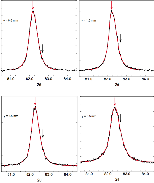
FIG. 11. (Color online) X-ray diffraction data for the \text{YBa}_2\text{Cu}_3\text{O}_{\nabla x} film. Fits to the \langle 00 10 \rangle peak for y = 0.5 mm - 3.5 mm. The red arrow indicates the maximum of the curve fit. The black arrow indicates a spurious substrate peak (which does not undergo change in 2\theta as the oxygen content of the \text{YBa}_2\text{Cu}_3\text{O}_{\nabla x} film does).
