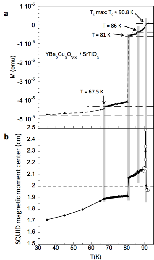
FIG. 3. Magnetization data for the \text{YBa}_2\text{Cu}_3\text{O}_{\nabla x} film. (a) Total magnetic moment vs. temperature, M(T) , of the \text{YBa}_2\text{Cu}_3\text{O}_{\nabla x} sample. (b) Magnetic moment signal center in the SQUID magnetometer vs temperature, M_{\text{center}}(T) . Open circles indicate data from voltage signal curves shown in Fig. 2. Filled circles are the average of four magnetization / center position measurements taken at each temperature. The values of 1.5 cm, 2.0 cm, and 2.5 cm of the signal position corresponds to the sample length positions of y = 0 mm, y = 5 mm, and y = 10 mm, respectively. (See also Fig. 7).
