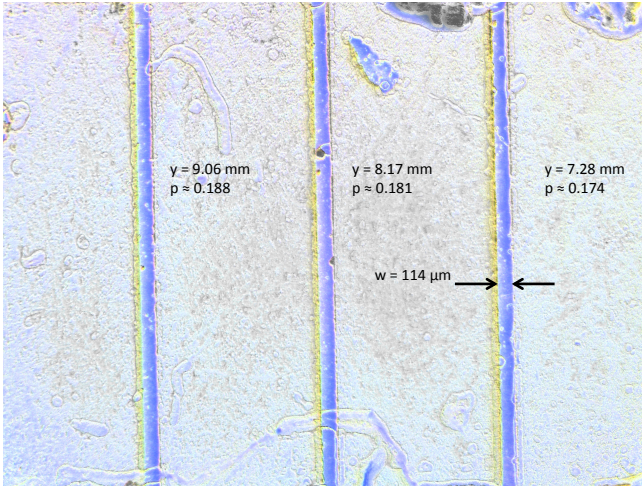
FIG. 9. (Color online) Polarized optical image of the resistivity bridges on the \text{YBa}_2\text{Cu}_3\text{O}_{\nabla x} film. The image shows segments of the film on the overdoped region of the film with p \approx 0.188 , 0.181 , and 0.174 . No twinning is observed at the micro-scale. Thermal grease can be seen remaining on the film and substrate surfaces. Remnant un-etched portions of the film can also be seen.
