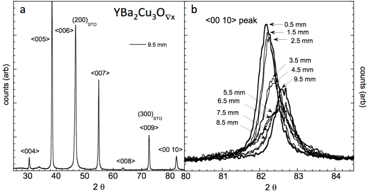
FIG. 4. Integrated x-ray diffraction data for the \text{YBa}_2\text{Cu}_3\text{O}_{\nabla x} film. (a), Full diffraction scan centered at position of (x, y) = (1.67 \text{ mm}, 9.5 \text{ mm}) . See Figs. (1) and (7) for corresponding axis configuration. (b) \langle 00 10 \rangle diffraction peak from a series of full diffraction scans at (x, y) = (1.67 \text{ mm}, [0.5, 1.5, \dots 9.5] \text{ mm}) . (See also Figs. 11 and 12 of Appendix B).
