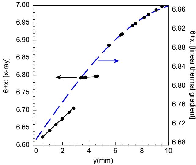
FIG. 8. (Color online) Oxygen content vs. sample position, 6+x vs. y(\text{mm}) , for the \text{YBa}_2\text{Cu}_3\text{O}_{\nabla x} film as determined from xray diffraction and resistivity data and calculated based upon an assumed linear temperature gradient. Solid black circles are calculated from a curve fit 37 to the data shown in Fig. 4a of Ref. [9] and from the p_{[avg]}(y) data given in Table 1 below. The blue dashed line is calculated by assuming a linear temperature profile along the sample (See Fig. 1) and from an empirical fit (via an extrapolation) to the data given in Table I of Ref. [10] with \log p_{\text{O}_2}^* = -4.0 to the expression 6+x = 5.9867 + 0.8845 \exp(-2.0319(1 - T/(275))^2) + 0.1 \cosh(1 - T/380) . The blue dashed line is then arrived at with T(y) = 395 - 105y[\text{cm}] , assuming an equilibrium linear thermal profile. 39 Note that the scales on the left and right y-axes are different, and thus there is a small discrepancy between the ranges of oxygen concentration in the film calculated by the two methods. Also, our sample was annealed in an oxygen atmosphere with P = 120 mtorr, corresponding to \log p_{\text{O}_2}^* = -3.8 , hence a small underestimation of the oxygen content can be expected. However, qualitatively, the two calculations of the oxygen distribution are in good agreement above y = 5.5 mm prior to the p \approx 1/7 ( O \approx 6.8 ) discontinuity. Interestingly, the (scaled) blue dashed line intercepts the edge of the p = 1/7 plateau and the tail of the p \lesssim 1/8 region at the edge of the sample.
