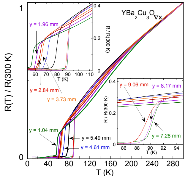
FIG. 6. (Color online) Normalized resistance vs. temperature, R(T)/R(T = 300\text{K}) , as a function of sample position.
