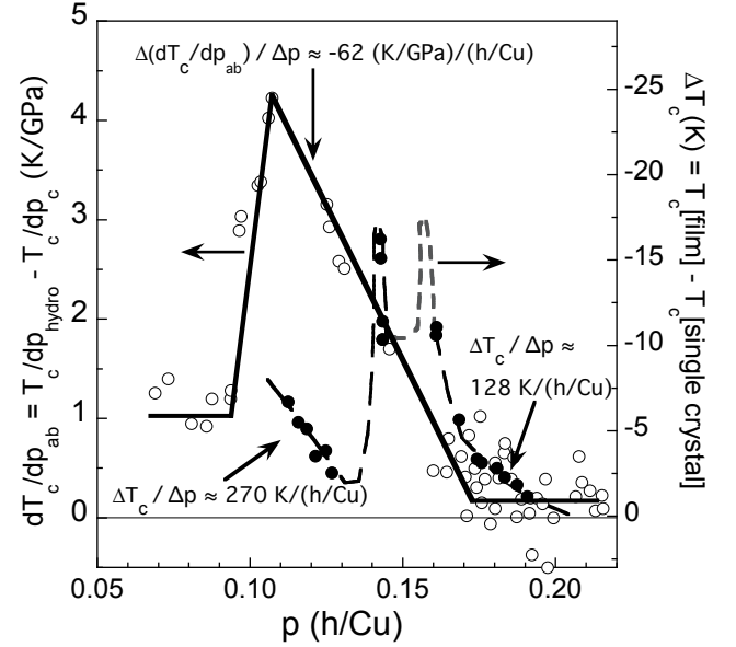
FIG. 10. Comparison of the charge doping dependence of the change of T_c for single crystals due to in-plane pressure to the difference between the values of T_c of the \text{YBa}_2\text{Cu}_3\text{O}_{\nabla x} film and unstrained single crystals. The dT_c/dp_{ab} vs p data (open circles) are deduced values for compressive in-plane (a-b) pressure applied to single crystals of \text{YBa}_2\text{Cu}_3\text{O}_x . The single crystal data, along with the linear guide lines, are reproduced from Ref. [14]. Values of \Delta T_c vs. p (closed circles) for the strained \text{YBa}_2\text{Cu}_3\text{O}_{\nabla x} film are determined from Fig. 13 in Appendix C. The short dashed line is speculative as to the strain effects at the boundary between the p \approx 1/7 and p \approx 1/6 regions. Note the sign reversal used for the (right) \Delta T_c axis. A negative impact on T_c is consistent with compressive/expansive strain along the a/b -axis direction.
