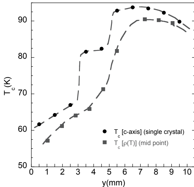
FIG. 13. Superconducting critical temperature vs. sample position, T_c vs. y(\text{mm}) . Values of T_c were determined by the mid point of the resistive transition (squares), and calculated from the c-axis lattice length extracted from x-ray diffraction data (circles) via the T_c - c(\text{nm}) relationship shown in Fig. (1b) of Ref. 9 . Note that the maximum value of T_c for our sample is \approx 3 K lower than that of their single crystals.
