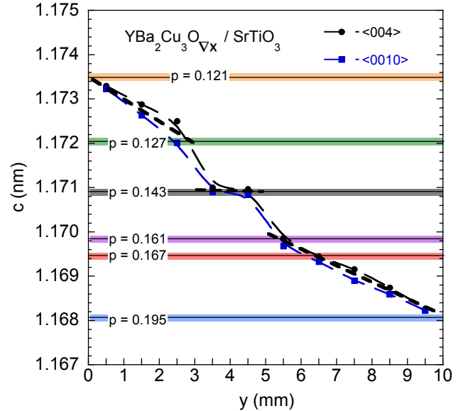
FIG. 5. (Color online) \text{YBa}_2\text{Cu}_3\text{O}_x film c -axis lattice parameter vs position, c(\text{nm}) vs y(\text{mm}) along the direction of the thermal gradient. Values of c(\text{nm}) are calculated from the series of the \langle 004 \rangle and the \langle 00 10 \rangle peaks. Linear fits to the average of the c -axis length determined from the two sets of peaks are shown for three distinct regions. In the regions from y \approx 0.5 \text{ mm} - 3.0 \text{ mm} and y \approx 5.0 \text{ mm} - 10 \text{ mm} the change in hole concentration per sample length is \Delta p / \Delta y \approx 6.1 \times 10^{-3} (holes/Cu)/mm and 7.4 \times 10^{-3} (holes/Cu)/mm, respectively. The intermediate region, in the p \approx 1/7 plateau, \Delta p / \Delta y \approx 7.4 \times 10^{-4} (holes/Cu)/mm.
