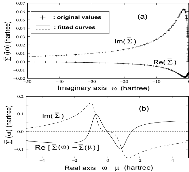
FIG. 4. The expectation value \bar{\Sigma}(i\omega) = \langle \psi'_i(0) | \Sigma(i\omega) | \psi'_i(0) \rangle for i = 6 on the imaginary axis (a). The crosses are the directly calculated values, and the continued lines are the analytical fitting curve; the analytically extended \bar{\Sigma}(\omega) on real \omega axis (b).
