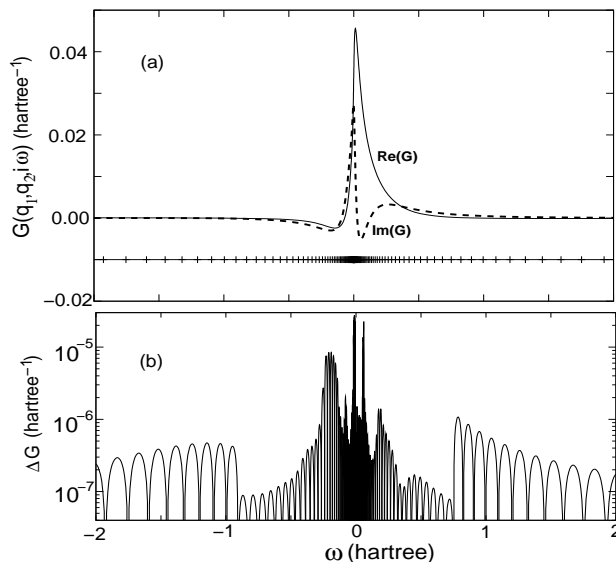
FIG. 1. The G_0(q_1, q_2, i\omega) for an typical off diagonal (q_1, q_2) element (a); and its fitting error within each interval [\omega_k, \omega_{k+1}] using the analytical formula with coefficients obtained from Eqs.(8)-(10). The horizontal line with ticks in (a) indicates the \omega_k positions.
