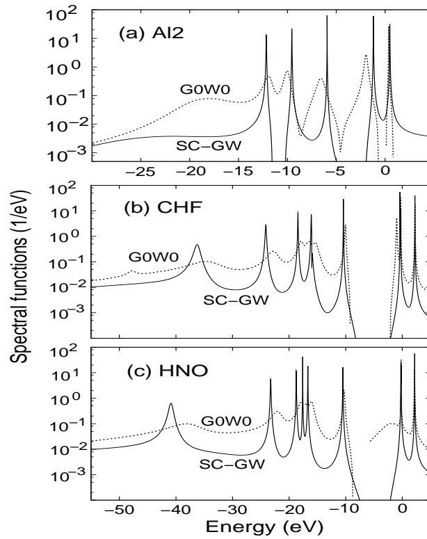
FIG. 6. The spectral functions as calculated from Eq.(19). The dotted lines are for G0W0 results starting with LDA input wave functions and eigen energies, and the solid lines are for sc-GW results. The Fermi energy \mu for Al2, CHF, and HNO are around -3,-5, -5 eV respectively.
