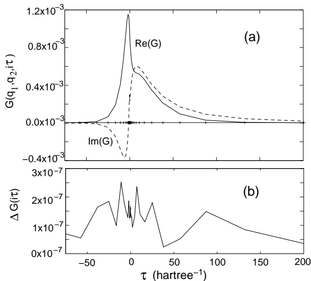
FIG. 2. The numerically integrated G_0(q_1, q_2, i\tau) from the G_0(q_1, q_2, i\omega) in Fig.1 (a); the error of the numerically integrated G_0(q_1, q_2, i\tau) when compared with the analytical expression of Eq.(16)(b). The ticks on the horizontal axis in (a) indicate the \tau_k positions.
