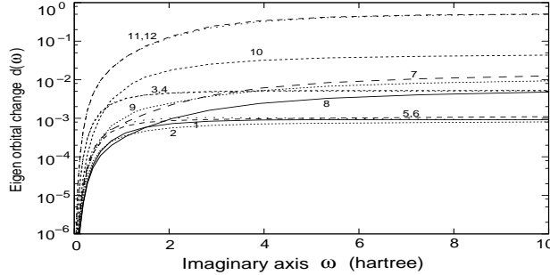
FIG. 5. The spread of the eigen vectors along the imaginary i\omega axis. The d_i(i\omega) is defined in the text. The numbers are the state index i 's.
