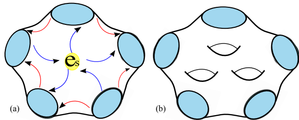
FIG. 1. Topologically ordered states on a 2D manifold with 1D boundaries: (a) Illustration of fusion rules and total neutrality , where anyons are transported from one boundary to another (red arrows), or when they fuse into physical excitations (blue arrows), on a manifold with five boundaries. (b) A higher genus compact surface with boundaries (thus with punctures): a genus-3 manifold with five boundaries.
