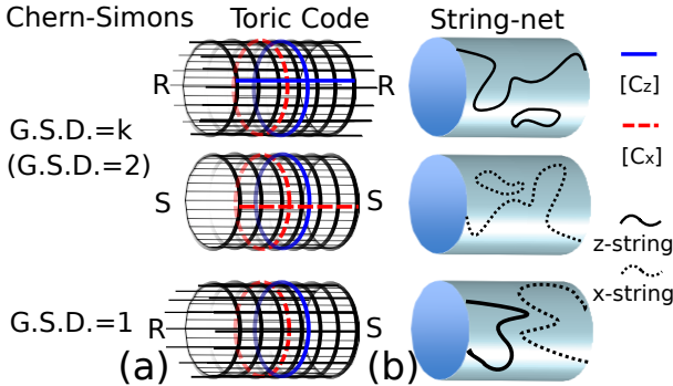
FIG. 2. (a) The same boundary conditions on two ends of a cylinder allow a pair of cycles [c_x], [c_z] of a qubit, thus \text{GSD} = 2 . Different boundary conditions do not, thus \text{GSD} = 1 . (b) The same boundary conditions allow z - or x -strings connect two boundaries. Different boundary conditions do not.
