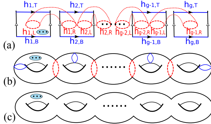
FIG. 4. Glue the punctured cylinders to form a genus g Riemann surface with \eta' punctures. Start from (a), firstly identify left and right \triangleright arrows of each square to form a number g of punctured cylinders. Then glue h_{j,L} and h_{j,R} (red dotted circles) together for 1 \leq j \leq g-1 , and glue h_{i,T} and h_{i,B} (blue arrows) together for 1 \leq i \leq g , which yields (b), equivalently as a genus g Riemann surface (c). The extra \eta' punctures are indicated here as a shaded blue puncture in the left most handle.
