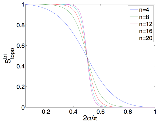
FIG. 10. S_{\text{topo}}^{\text{tri}} for the transverse Ising model. The horizontal axis is the angle 2\alpha/\pi for the Hamiltonian H(\alpha) as given in Eq. (16). A similar result is presented in Ref 39 , from a different viewpoint.
