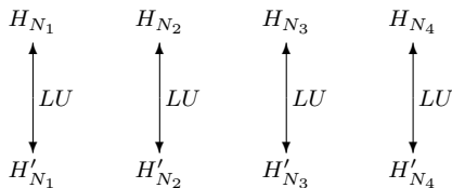
FIG. 2. The two rows of Hamiltonians describe two gapped quantum systems. The two rows connected by LU transformations represent the equivalence relation between the two gapped quantum systems, whose equivalence classes are gapped quantum phases. We may view H_N as a projector that defines its ground-state subspace. The ground-state subspaces of two equivalent systems are connected by the LU transformations.
