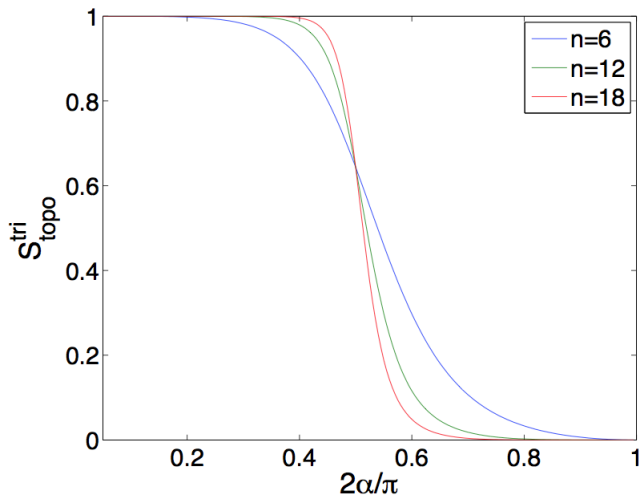
FIG. 11. S_{\text{topo}}^{\text{tri}} for the transverse Ising model. The ratio r = 2 : 1 , and the system sizes are n = 6, 12, 18 qubits.
