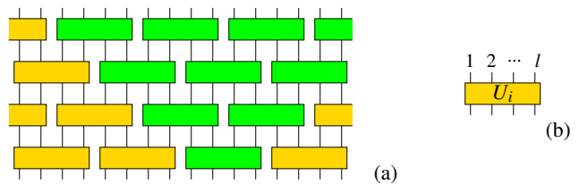
FIG. 1. (Color online) (a) A graphic representation of a quantum circuit, which is form by (b) unitary operations on blocks of finite size l . The green shading represents a causal structure.
