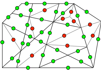
FIG. 5. Toric code as a gapped quantum liquid: toric code of N_k qubits on an arbitrary 2D lattice, where the green dots represent qubits sitting on the link of the lattice (given by solid lines). By adding N_{k+1} - N_k qubits (red dots), the gLU transformation H_{N_k} \rightarrow H_{N_{k+1}} ‘dissolves’ the red qubits in the new lattice (with both the solid lines and dashed lines).
