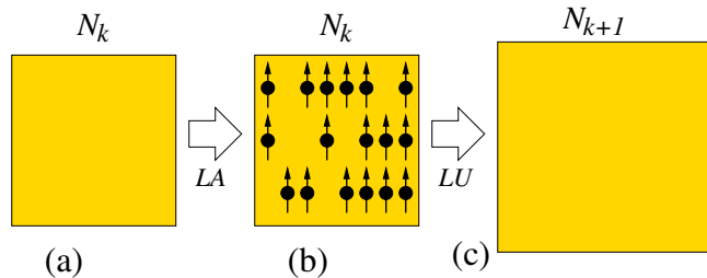
FIG. 4. (Color online) Two systems (a) and (c), with size N_k and N_{k+1} , are described by H_{N_k} and H_{N_{k+1}} respectively. (a) \rightarrow (b) is an LA transformation where we add N_{k+1} - N_k qubits to the system H_{N_k} to obtain the Hamiltonian H_{N_k} + \sum_i Z_i for the combined system (b). Under the LA transformation, the ground states of H_{N_k} is tensored with a product state to obtain the ground states of H_{N_k} + \sum_i Z_i . In (b) \rightarrow (c), we transform the ground-state subspace of H_{N_k} + \sum_i Z_i to the ground-state subspace of H_{N_{k+1}} via an LU transformation.
