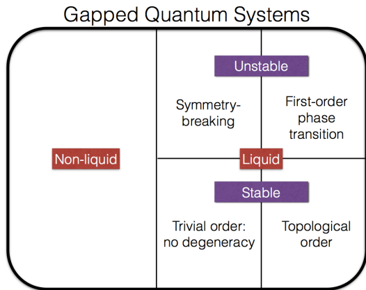
FIG. 6. Summary of gapped quantum systems: gapped quantum systems include gapped quantum liquid systems, and systems that are not liquid (nonliquid). For gapped quantum liquids, there are stable systems (including the trivial systems given by e.g. the Hamiltonian H_{N_k}^{\text{non-liquid}} and the topologically ordered systems) and unstable systems (including symmetry-breaking systems and first-order phase transitions).
