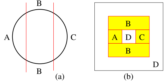
FIG. 8. (a) Cutting a ring into three parts A, B, C . (b) Cutting a 2D system into four parts A, B, C, D .
