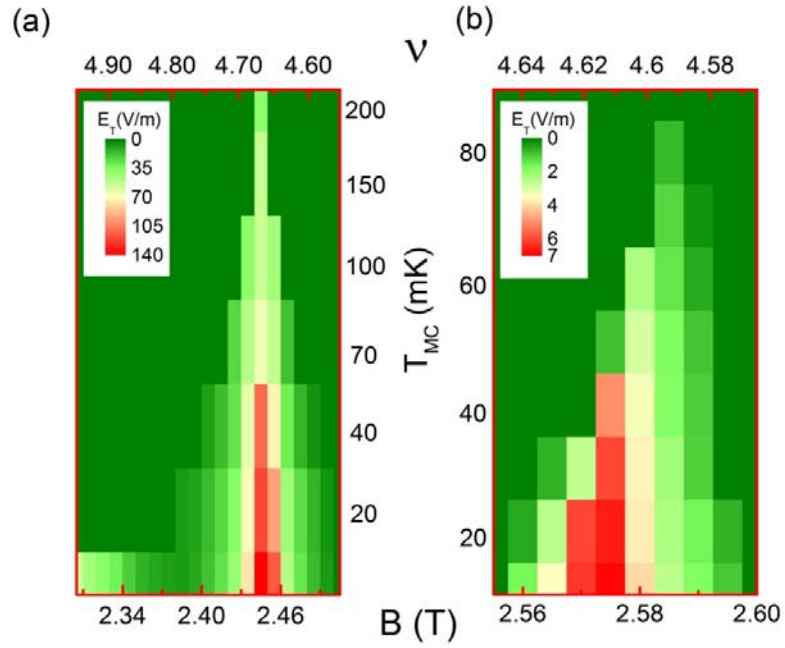
FIG. 3. (a) B-T phase diagram of RIQHE=5 for Sample B, different colors represent different values of threshold electric fields. (b) B-T phase diagram of RIQHE=4 for Sample B, different colors represent different values of threshold electric fields.
