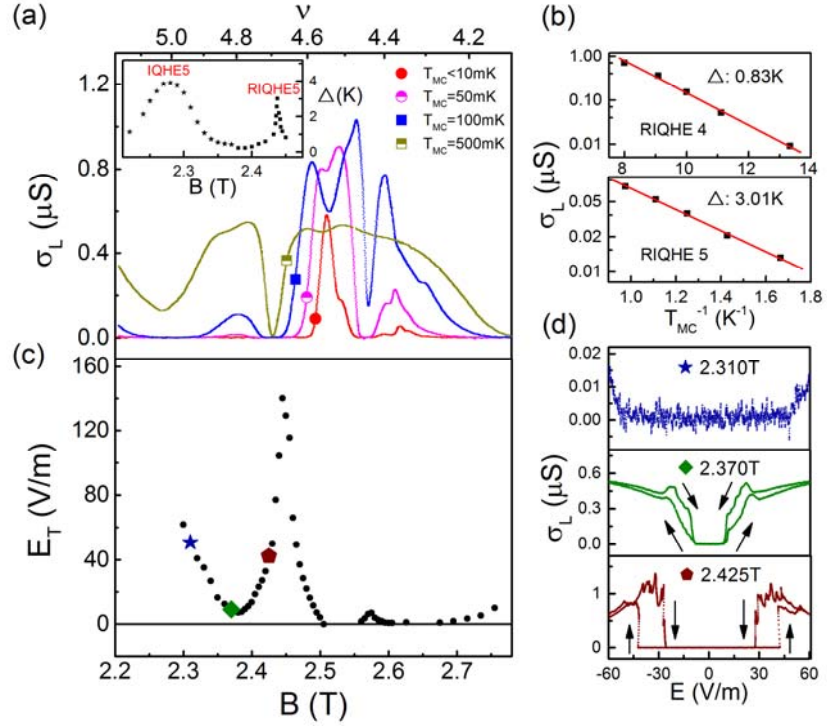
FIG. 2. (a) Differential conductivity of Corbino Sample B as a function of the magnetic field at different temperatures. Inset is the energy gap \Delta as a function of magnetic field, showing a transition from IQHE to RIQHE. Below 2.375 T (symbol star), the energy gap is fitted by the equation \sigma_L \propto \exp(-\Delta/2k_B T) . Above 2.375 T (symbol square), the energy gap is fitted by the equation \sigma_L \propto \exp(-\Delta/k_B T) . (b) Examples of energy gap of reentrant states, fitted by the equation \sigma_L \propto \exp(-\Delta/k_B T) . (c) Threshold electric field E_T as a function of magnetic field at the lowest temperature. (d) From top to bottom, they are examples for IQHE breakdown, crossover behavior from IQHE=5 to RIQHE=5, and RIQHE de-pinning, respectively. The examples at three filling factors are labeled differently in (c).
