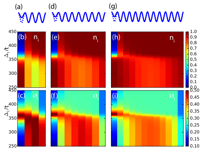
FIG. 4: (Color online) Exact diagonalization results of the density n_i and its variance \sigma_i as functions of \Delta_1 for Case-1 with OBC. Site 2 to N are uniform and U = 10t . (a)-(c) show the results for a 4-site array with 3 photons. In (a) the dashed line and solid line on the first site correspond to the two schemes shown in Fig. 3. (d)-(f) correspond to the case of 8 sites with 7 photons. (g)-(i) correspond to 12 sites with 11 photons.
