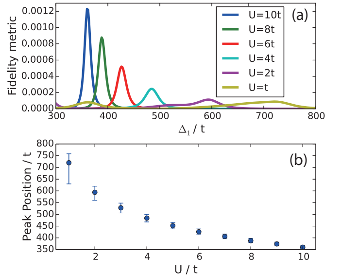
FIG. 7: (Color online) (a) Fidelity metric as a function of \Delta_1 for different values of U for N = 8 and 7 photons. (b) Peak position of Fidelity metric as a function of U/t . The full width at half maximum (FWHM) is shown as the bar spanning across each point.
