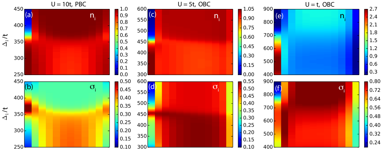
FIG. 5: (Color online) Photon density profiles and its variance for selected values of U and boundary conditions. (a) and (b): U/t = 10 and PBC. In this case, the photons in site 2 and N can both tunnel to site 1. Hence the photon density on site 2 and N are different from the bulk value due to boundary effects. (c) and (d): U/t = 5 and OBC. (e) and (f): U/t = 1 and OBC. The non-uniform density and its significant variance of the last case indicate that there is no Mott insulator in this setting. Here N = 12 with 11 photons.
