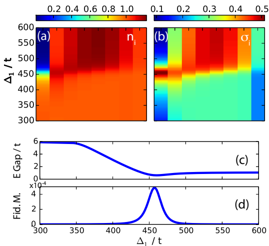
FIG. 8: (Color online) Exact diagonalization results for Case 2 with N = 8 and 8 photons. Here U = 10t . (a) and (b) show the density profile in the array and the density variance. The energy gap (E Gap) and fidelity metric (Fid. M.) in (c) and (d) clearly exhibit signatures of the MI-SF transition.
