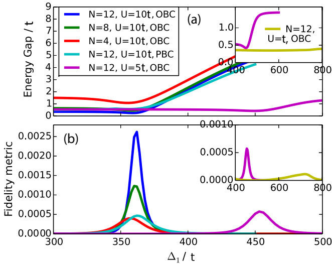
FIG. 6: (Color online) (a) Energy gap for different values of U and N . The inset shows a regime when U = t , in yellow, for N = 12 with OBC compared to U = 5t from the main figure. (b) The peaks of the fidelity metric indicate the critical points. When N varies, the location of the critical point remains intact. However, varying the on-site interaction U changes the location of the critical point, which is consistent with the analysis in Sec. III. Note that PBC gives the same critical point as OBC.
