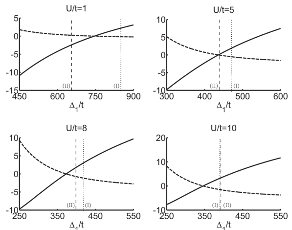
FIG. 2: \delta (solid lines) and \eta (dashed lines) as functions of \Delta_1 for U/t = 1, 5, 8, 10 and g_q = 120\text{MHz} \times 2\pi . As Eq. (16) shows, \delta and \eta are the displacements of the on-site energy and on-site interaction of the first site. The vertical lines (I) and (II) indicate the mean-field critical values of the two cases discussed in Sec. III.
