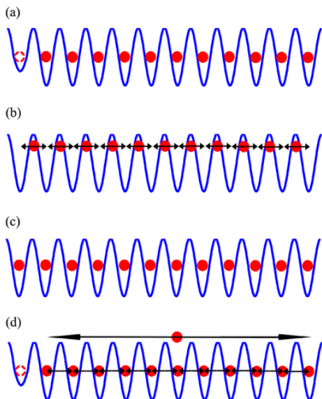
FIG. 3: (Color online) Illustration of single-site manipulations of the Mott insulator to superfluid transition for N - 1 bosons with strong repulsion in N sites ((a) and (b)) and for N bosons with strong repulsion in N sites ((c) and (d)). (a) The on-site energy of site-1 is increased and the system is pushed into a localized Mott insulator. The dashed circle implies that the first site is virtually empty. (b) The system becomes a delocalized superfluid as the on-site energy is lowered. (c) The system is a localized Mott insulator when the onsite energy of site 1 is small. (d) By increasing the on-site energy of site 1, photons are pushed into the bulk and form a delocalized superfluid.
