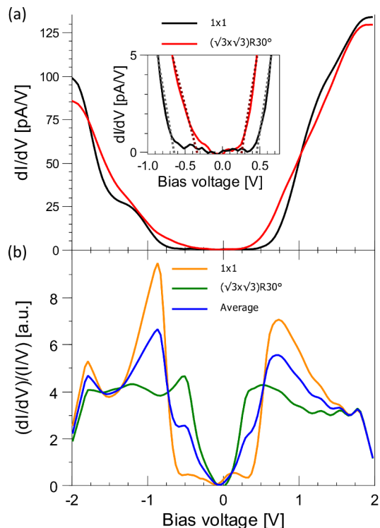
FIG. 3. (Color online) (a) Differential conductivity spectra of the 1 \times 1 and (\sqrt{3} \times \sqrt{3})\text{R}30^\circ surface. The inset shows a zoom into the onset region of conduction and valence bands. The gap is estimated by linear extrapolation of the band edges to zero conductance, indicated as dashed lines [13]: For the 1 \times 1 surface we observe the gap to be E_g \approx 1.2 eV, while the (\sqrt{3} \times \sqrt{3})\text{R}30^\circ surface shows a smaller gap of E_g \approx 0.6 eV. (b) Normalized differential conductivity graphs of the two surfaces and their average. Spectral features are visible at V_{\text{bias}} \simeq \pm 1 V. The averaged spectrum, assuming equal surface coverages, allows a comparison to ARPES and optical conductivity measurements. Note: The signal inside the gap is below the setup resolution limit and apparent features are computational noise [13].
