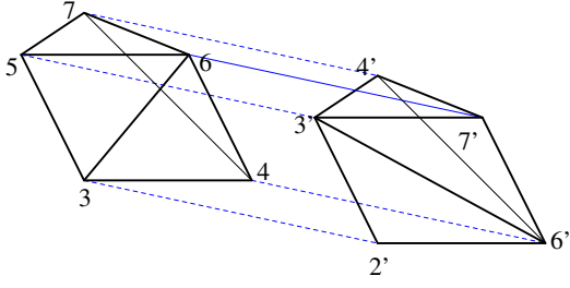
FIG. 14. The complex M_2 .
