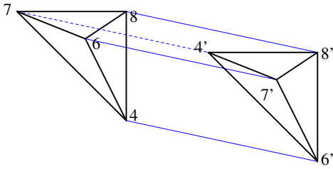
FIG. 16. The complex M_4 .
