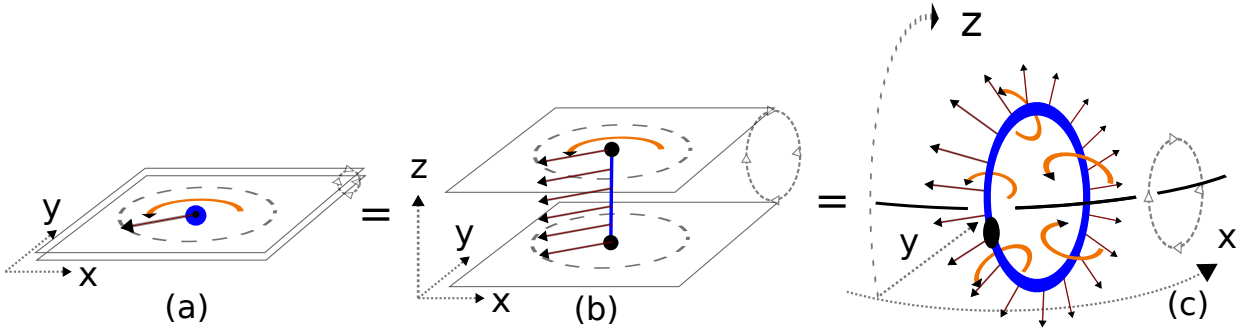
FIG. 6. Topological spin of (a) a particle by 2\pi -self rotation in 2D, (b) a framed closed-string by 2\pi -self rotation in 3D with a compact z , (c) a closed-string (blue) by 2\pi -self flipping, threaded by a background (black) string creating monodromy b flux (along the arrow - - \rightarrow ), under a single Hopf link 2_1^2 configuration. All above equivalent pictures describe the physics of topological spin in terms of \mathbb{T}_b^{xy} . For Abelian topological orders, the spin of an excitation (say A ) in Fig.6(a) yields an Abelian phase e^{i\Theta(A)} = \mathbb{T}_{(A)(A)}^{xy} proportional to the diagonal of 2D's \mathbb{T}^{xy} matrix. The dimensional-extended equivalent picture Fig.6(c) implies that the loop-flipping yields a phase e^{i\Theta(A), b} = \mathbb{T}_{b(A)(A)}^{xy} of Eq.(31) (up to a choice of canonical basis), where b is the flux of the black string.
