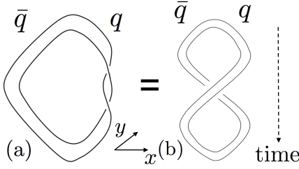
FIG. 5. Both process (a) and (b) starts from creating a pair of particle q and anti-particle \bar{q} , but the worldlines evolve along time to the bottom differently. The process (a) produces a phase e^{i2\pi s} due to 2\pi rotation of q , with spin s . The process (b) produces a phase e^{i\Theta} due to the exchange statistics. The homotopic equivalence by deformation implies e^{i2\pi s} = e^{i\Theta} .
