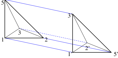
FIG. 15. The complex M_3 .
