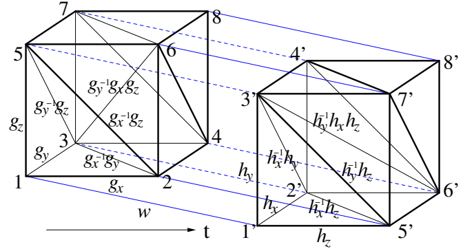
FIG. 12. The space-time complex \mathbb{T}^3 \times I , where I = [0, 1] is the time direction. The figure shows \mathbb{T}^3 \times \{0\} and \mathbb{T}^3 \times \{1\} . The blue lines illustrate how the two \mathbb{T}^3 are connected for t \in (0, 1) . Note that the two \mathbb{T}^3 's differ by a rotation S^{xyz} . In other words, when time forms a loop, the two \mathbb{T}^3 are glued together by 1 \rightarrow 1' , 2 \rightarrow 2' , 3 \rightarrow 3' , 4 \rightarrow 4' , 5 \rightarrow 5' , 6 \rightarrow 6' , 7 \rightarrow 7' , and 8 \rightarrow 8' .
