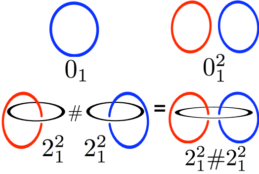
FIG. 10. Under Alexander-Briggs notation, an unknot is 0_1 , two unknots can form an unlink 0_1^2 . A Hopf link is 2_1^2 , a connected sum of two Hopf links is 2_1^2 \# 2_1^2 .
