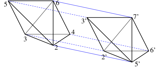
FIG. 17. The complex M_1' .
