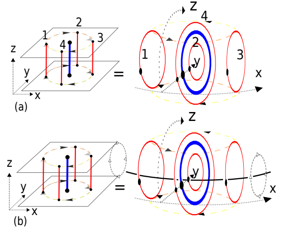
FIG. 9. For 3+1D Type IV \omega_{4,IV} twisted gauge theory \mathcal{C}_{G, \omega_{4,IV}}^{3D} : (a) Two-string statistics in unlink 0_1^2 configuration is Abelian. (The b = 0 sector as \mathcal{C}_G^{2D} .) (b) Three-string statistics in two Hopf links 2_1^2 \# 2_1^2 configuration is non-Abelian. (The b \neq 0 sector in \mathcal{C}_b^{2D} = \mathcal{C}_{G, \omega_{3,III}}^{2D} .) The b \neq 0 flux sector creates a monodromy effectively acting as the third (black) string threading the two (red, blue) strings.
