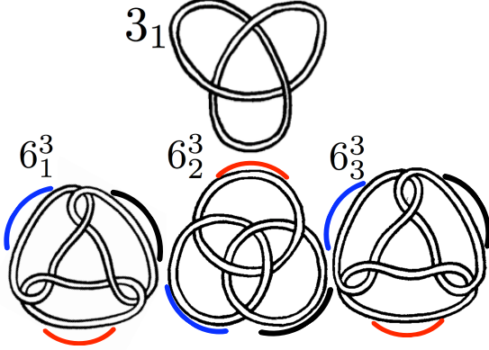
FIG. 11. The trefoil knot is 3_1 . Some other simplest 3-string links (beyond Hopf links 2_1^2 \# 2_1^2 ) are given: 6_1^3 , 6_2^3 (Borromean rings), 6_3^3 . From the spin-statistics relation of a closed string discussed in Sec.III C, where the topological spin of certain knot/link configurations ( 0_1 for the monodromy flux b = 0 and 2_1^2 for b \neq 0 ) is equivalent to the exchange statistics of certain knot/link configurations ( 0_1^2 for b = 0 and 2_1^2 \# 2_1^2 for b \neq 0 ) under Eq.(35). Therefore, we may further conjecture that the topological spin of a trefoil knot 3_1 may relate to the braiding statistics of 6_1^3 , 6_2^3 , 6_3^3 .
