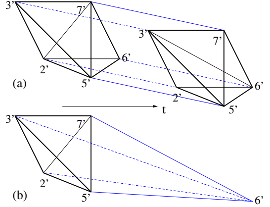
FIG. 17. The complex M_1' .
