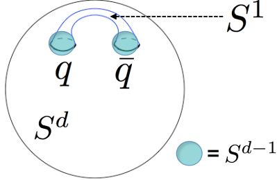
FIG. 8. The number of particle types = GSD on S^{d-1} \times S^1
