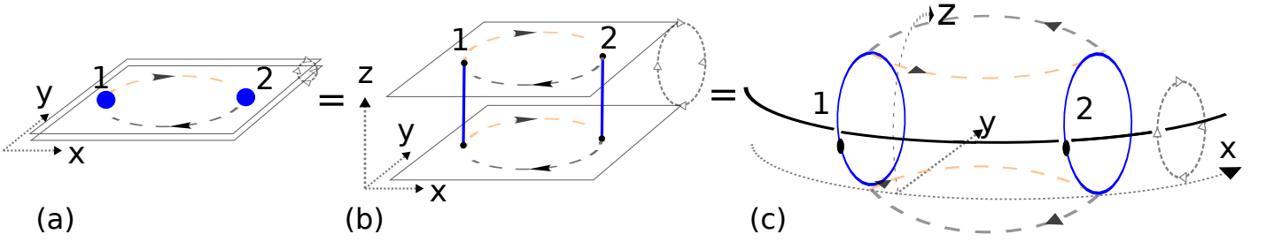
FIG. 7. Exchange statistics of (a) two identical particles at positions 1 and 2 by a \pi winding (half-winding), (b) two identical strings by a \pi winding in 3D with a compact z , (c) two identical closed-strings (blue) with a \pi -winding around, both threaded by a background (black) string creating monodromy b flux, under the Hopf links 2_1^2 \# 2_1^2 configuration. Here figures (a)(b)(c) describe the equivalent physics in 3D with a compact z direction. The physics of exchange statistics of a closed string turns out to be related to the topological spin of Fig.6, discussed in Sec.III C 3.
