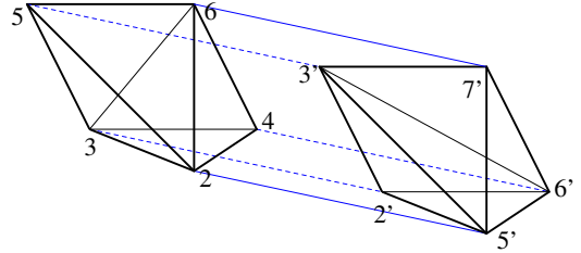
FIG. 13. The complex M_1 .
