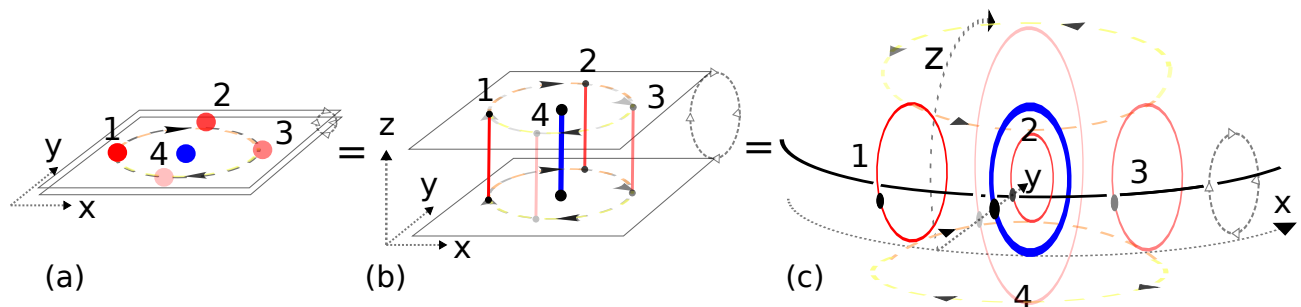
FIG. 2. Mutual braiding statistics following the path 1 \rightarrow 2 \rightarrow 3 \rightarrow 4 along the time evolution (see Sec.III C 2): (a) From a 2D viewpoint of dimensional reduced C_b^{2D} , the 2\pi braiding of two particles is shown. (b) The compact z direction extends two particles to two closed (red, blue) strings. (c) An equivalent 3D view, the b flux (along the arrow - - \triangleright ) is regarded as the monodromy caused by a third (black) string. We identify the coordinates x, y and a compact z to see that a full-braiding process is the one (red) string going inside to the loop of another (blue) string, and then going back from the outside . For Abelian topological orders, the mutual braiding process between two excitations (A and B) in Fig.2(a) yields a statistical Abelian phase e^{i\theta^{(A)(B)}} \propto S_{(A)(B)}^{xy} proportional to the 2D's S^{xy} matrix. The dimensional-extended equivalent picture Fig.2(c) implies that the loop-braiding yields a phase e^{i\theta^{(A)(B),b}} \propto S_{b(A)(B)}^{xy} of Eq.(34) (up to a choice of canonical basis), where b is the flux of the black string. We clarify that in both (b) and (c) our strings may carry both flux and charge. If a string carries only a pure charge, then it is effectively a point particle in 3D. If a string carries a pure flux, then it is effectively a loop of a pure string in 3D. If a string carries both charge and flux (as a dyon in 2D), then it is a loop with string fluxes attached with some charged particles in 3D. Therefore our Fig.2(c)'s string-string braiding actually represents several braiding processes: the particle-particle, particle-loop and loop-loop braidings, all processes are threaded with a background (black) string.
