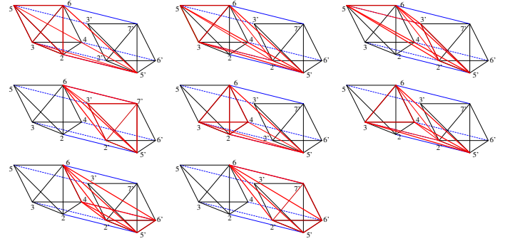
FIG. 19. The complex M_1' is formed by eight 4-simplices.
