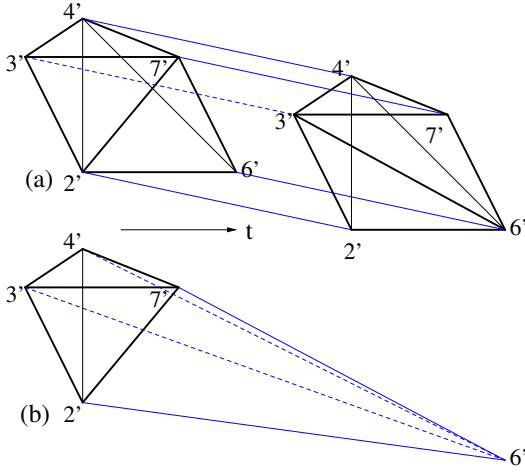
FIG. 21. The complex M''_2 , which is formed by one 4-simplex. Note that all the vertices in (a) are on the same time slice but the (curved) edge (2'7') is on an earlier time slice and the (curved) edge (3'6') is on a later time slice. To realize this using straight edges, we put the vertex 6' on a later time slice, and this gives us a 4-simplex in (b).
