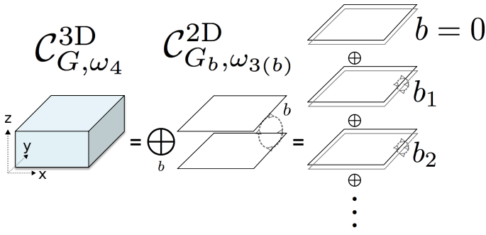
FIG. 4. Combine the reasoning in Eq.(18) and Fig.1, we obtain the physical meaning of dimensional reduction from a 3+1D twisted gauge theory as a 3D topological order to several sectors of 2D topological orders: \mathcal{C}_{G, \omega_4}^{3D} = \bigoplus_b \mathcal{C}_{G_b, \omega_3(b)}^{2D} . Here b stands for the gauge flux (Wilson line operator) of gauge group G . Here \omega_3 are dimensionally reduced 3-cocycles from 4-cocycles \omega_4 . Notice there is a zero flux b = 0 sector with \mathcal{C}_{G, (\text{untwist})}^{2D} = \mathcal{C}_G^{2D} .
