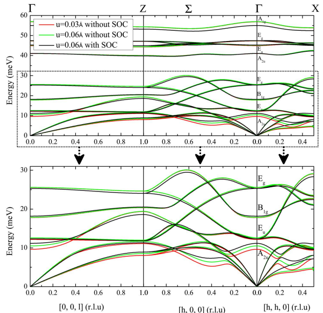
FIG. 14. (Color online) Ab initio calculation of the phonon dispersion curves along \Gamma Z , \Gamma\Sigma Z and \Gamma X at 0 K. The parameter u sets for the displacements of the atoms. Increasing u from 0.03 \text{ \AA} (red line) to 0.06 \text{ \AA} (green line) is used to probe the effects of anharmonicity. Black line shows the calculation with spin-orbit coupling (SOC). The black line is the closest to the experimental results and is the one reported in Figure 13
