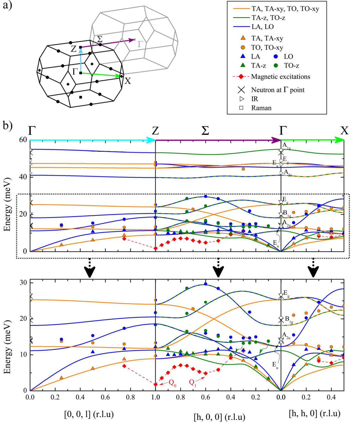
FIG. 13. (Color online) (a) Brillouin zone of the body centered tetragonal crystal structure of \text{URu}_2\text{Si}_2 in the paramagnetic state. The arrows indicate the direction of the dispersion for the Inelastic Neutron Scattering (INS) measurements, as reported below. (b) Phonons and magnetic excitations (full red diamonds) dispersion along the \Gamma Z ( [0,0,1] ), Z\Sigma\Gamma ( [1,0,0] ) and \Gamma X ( [1,1,0] ) directions. Full circles and full upward triangles are INS data for the optical and acoustic branches, respectively. Each reported energy is the energy average of all measured temperature for each phonon mode (See text). Empty symbols are data obtained in the zone center at \Gamma , with cross, open triangles and squares for INS, IR and Raman measurements, respectively. Dashed lines are guides to the eyes for the magnetic excitations dispersion. Solid lines corresponds to the ab initio GGA calculation with spin-orbit coupling and u=0.06 \text{ \AA} (See section VI). When the dispersion curve has a mixed character (for instance from LO (in \Gamma ) to TO-z (in Z ) along [1,0,0] ), the solid lines are bicolored. The black arrow points to the E_u(1) phonon mode measured by IR at \Gamma point. The green arrows indicate the calculated branch which corresponds to the measured points (green full circles). Q_0 and Q_1 correspond to the minima in magnetic excitation dispersion, known as commensurate and incommensurate excitations, respectively.
