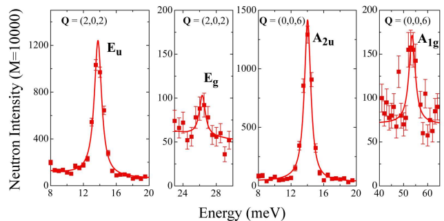
FIG. 11. (Color online) Inelastic Neutron Scattering phonon spectra at \Gamma point measured for \mathbf{Q}=(2, 0, 2) and \mathbf{Q}=(0, 0, 6) at T = 300 K. The E_u and E_g phonon modes have been observed for \mathbf{Q}=(2, 0, 2) and A_{2u} and A_{1g} phonon modes for \mathbf{Q}=(0, 0, 6) . The neutron intensity is given for a normalized incident flux (M) which corresponds to a counting time of approximately 80s for E_u , E_g , A_{2u} and 110s for A_{1g} . Lines are fits of the data with an harmonic oscillator lineshape.
