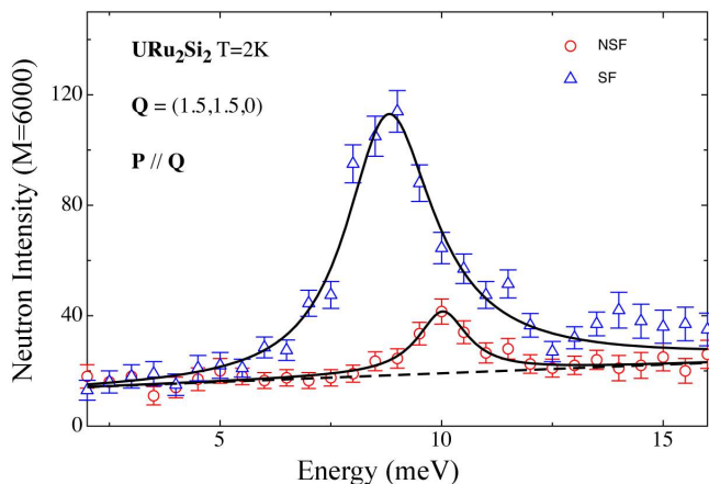
FIG. 12. (Color online) Polarized Inelastic Neutron Scattering spectra measured for \mathbf{Q}=(1.5, 1.5, 0) in the Non Spin Flip (NSF) and Spin Flip (SF) channels for T = 2 K. Full lines are fits of the data with functions described in the text. The dashed line indicates the background. The neutron intensity is given for a normalized incident flux which corresponds to a counting time ( M ) of approximately 25min.
