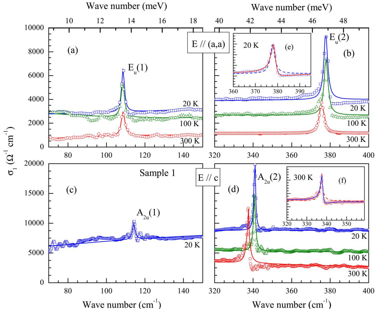
FIG. 6. (Color online) Optical conductivity centered around each phonon of \text{URu}_2\text{Si}_2 at selected temperatures. Panels (a) and (b) are for light polarized on the (a,a) plane and panels (c) and (d) are for measurements along the c -direction. Symbols are the data and the lines are Drude-Lorentz fits as described in the text. Inset (e) shows the highest frequency E_u(2) mode at 20 K described by either a Lorentz oscillator (dashed line) or a Fano mode (solid line). Panel (f) is the equivalent to panel (e) for the highest frequency A_{2u}(2) mode at 300 K.
