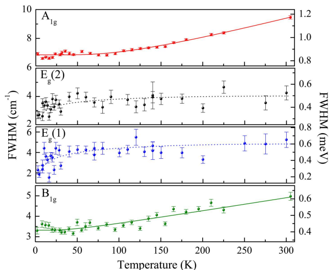
FIG. 5. (Color online) Temperature dependence of the FWHM of A_{1g} , E_g(1) , E_g(2) and B_{1g} phonon modes. Lines are fits with a single anharmonic model 37,38 . Dot lines are guides to the eyes.
