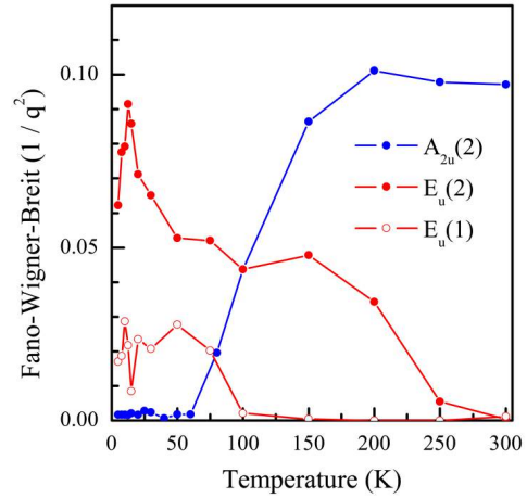
FIG. 9. (color online) Temperature dependence of Fano-Wigner-Breit q^{-2} parameter for both E_u and the highest frequency A_{2u} phonons. When an electron-phonon coupling occurs, the Fano-Wigner-Breit q^{-2} parameter becomes different from zero.
