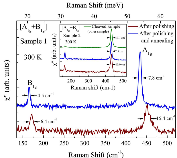
FIG. 2. (Color online) Raman spectra of \text{URu}_2\text{Si}_2 for sample 1 after polishing along the (a,c) plane and annealing. Inset: Raman spectra for sample 2 after polishing along the (a,a) plane, annealing and for another sample cleaved along the (a,a) plane.
