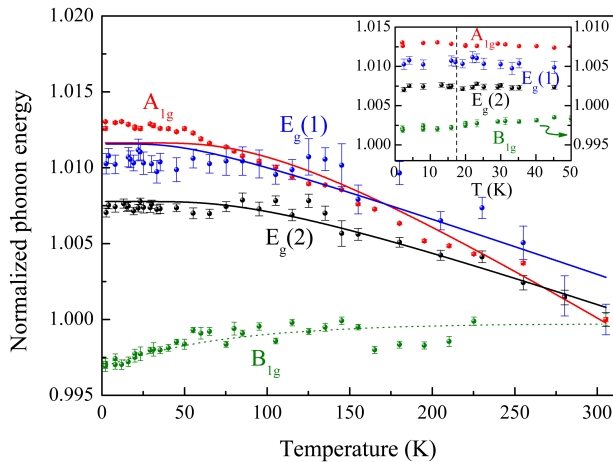
FIG. 4. (Color online) Temperature dependence of the position of the A_{1g} , E_g(1) , E_g(2) and B_{1g} phonon modes normalized to their value at 300 K. B_{1g} phonon exhibits an unusual softening when cooling down below 100 K. Error bars have been extracted from the Lorentzian fits. Lines are fits with a single anharmonic model 37,38 . The green dot line is a guide to the eyes. Inset : zoom of the data at low temperature (hidden order transition is marked by the vertical black dashed line). No particular anomaly is measured at T_0 .
