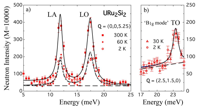
FIG. 10. (Color online) Inelastic Neutron Scattering phonon spectra measured for (a): \mathbf{Q}=(0, 0, 5.25) at T = 2, 60 and 300 K performed on IN8 and (b): \mathbf{Q}=(2.5, 1.5, 0) at T = 2 and 30 K performed on IN22. L and T, A and O stand for longitudinal and transverse, acoustic and optic, respectively. The TO mode belongs to the branch that corresponds to the B_{1g} mode at \mathbf{Q}=0 . Lines are fits of the data with an harmonic oscillator lineshape and sloppy background. The neutron intensity is given for a normalized incident flux (M) which corresponds to a counting time of approximately 80s.
