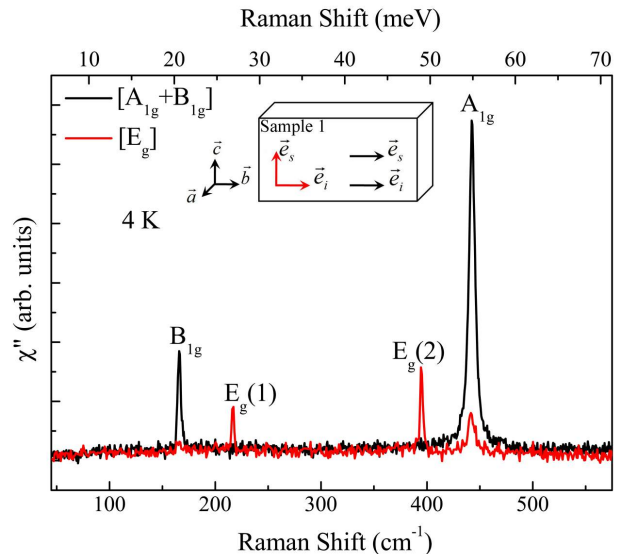
FIG. 3. (Color online) Typical Raman spectra measured at 4 K in cross and parallel polarization of the light. A scheme of sample 1 with the orientation of the polarizations of the incident \vec{e}_i and scattering \vec{e}_s light is shown.
