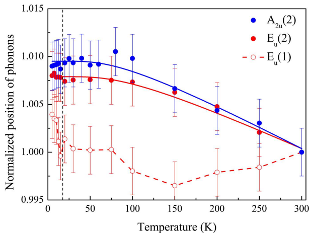
FIG. 8. (Color online) Temperature dependence of the frequency of A_{2u}(2) , E_u(1) and E_u(2) phonon modes normalized to their value at 300 K. Lines are fits with a single anharmonic model (See Section III C). The vertical black dashed line marks the transition into the hidden order.
