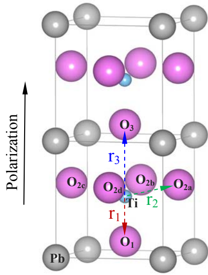
Figure 3. Schematic atomic structure of ferroelectric \text{PbTiO}_3 with two unit cells.
