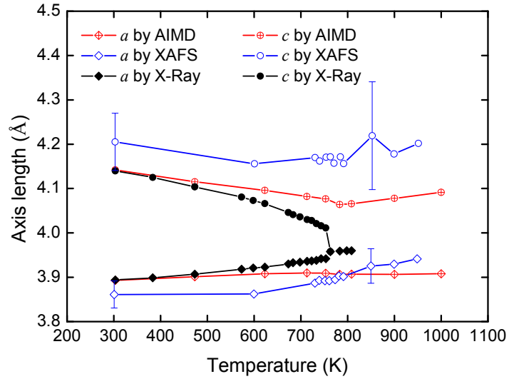
Figure 1. Temperature dependence of the lattice parameters a , c of \text{PbTiO}_3 unit cell. The data in crossed symbols are derived from current AIMD simulations, the open symbols are from the EXAFS measurements by Sicron et al. 12, 14 and the closed symbols are from the X-Ray diffraction by Shirane et al. 1 .
