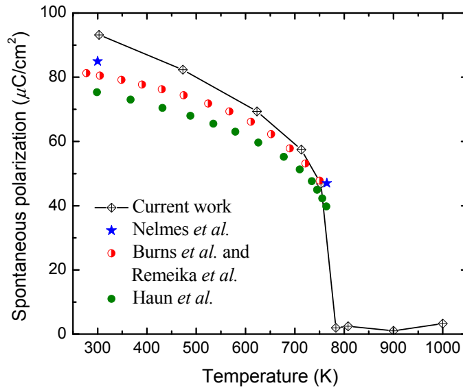
Figure 8. Variation of the polarization as a function of temperature, in comparison with available experimental data. The blue stars are from Ref. 32 and the green closed circles are from Ref. 33 . The red half-closed circles are quoted based on Refs. 10,39 , and the polarization data were derived as P_S = P_0 + \Delta P , where the P_0 = 42 \mu\text{C}/\text{cm}^2 at the Curie temperature 10 and \Delta P were from Ref. 39 .
