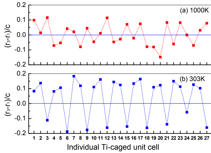
Figure 6. Distribution of the nominal polarizations of individual Ti-caged unit cell in the simulation supercell at (a) 1000 K and (b) 303 K at the instant of t = 18 ps. The positive and negative values of (r_3-r_1)/c indicate the opposite directions of local spontaneous polarization. The dashed lines are drawn for guiding eyes.
