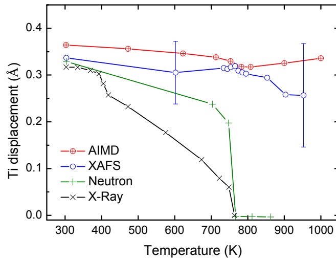
Figure 2. The displacement of Ti from the midpoint between the O_1 and O_3 atoms as shown in Figure 3. The crossed circles are from current work, the open circles are from the XAFS measurements 12-14 , the “+” and “×” are the results from neutron 36 and X-Ray 37,38 diffractions respectively.
