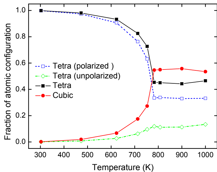
Figure 5. Fractions of the cubic (closed circles) and tetragonal (closed squares) configurations as a function of temperature, obtained from the AIMD simulations. Among the tetragonal configurations, the fractions of the polarized and unpolarized ones in the \langle 001 \rangle direction are shown in the open squares and open diamonds, respectively.
