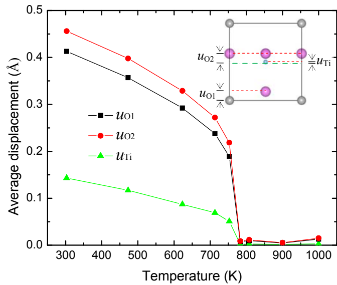
Figure 7. The displacements of O and Ti ions along \langle 001 \rangle direction as a function of temperature. The inset illustrates the definition of displacements with respect to the centrosymmetric cubic configuration.
