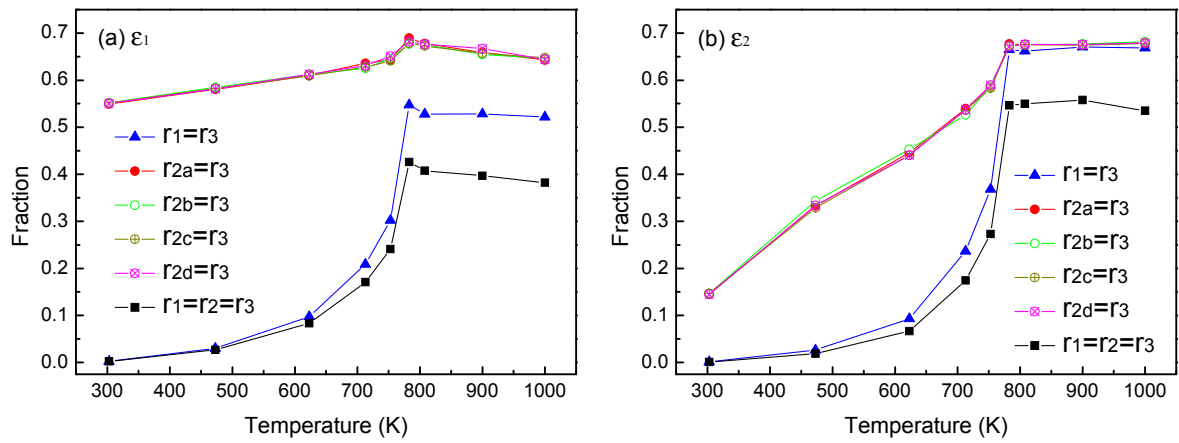
Figure 4. Fractions of atomic environments represented with the relevance of Ti-O bond lengths as a function of temperature based on the two considered uncertainty parameters: (a) \epsilon_1 and (b) \epsilon_2 .
