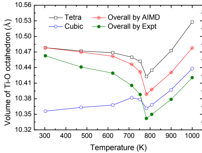
Figure 9. Temperature dependence of the volume of Ti-O octahedral clusters, showing the negative and positive thermal expansion. The volumes of Ti-O octahedra in the tetragonal and cubic configurations are shown in the open squares and open circles, respectively. The volumes of the overall Ti-O octahedra from current AIMD simulation and the experiment measurement by Shirane et al. 1 are shown in the crossed and closed circles, respectively.
