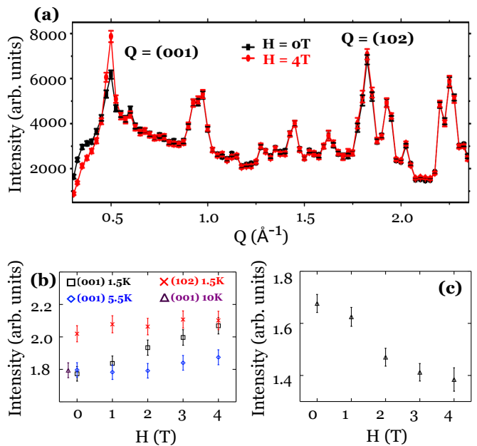
FIG. 5. (color online) (a) Elastic neutron scattering intensities at different fields at T = 1.5 K from the CNCS measurements. The data were integrated between -0.5 meV and 0.5 meV energy transfer. (b) The field dependence of the summed intensity of the Q = (001) Bragg peak at T = 1.5 K and T = 5.5 K and Q = (102) peak at T = 1.5 K. The Q = (001) intensity at T = 10 K at zero field is shown to demonstrate that Q = (001) intensity is purely nuclear at zero field. This intensity is displaced slightly along the negative x-axis direction for visualization. (c) The field dependence of the quasi-elastic scattering intensity at low Q around [0.3, 0.46] \text{ \AA}^{-1} summed over E = [0.1, 0.4] \text{ meV} measured at T = 1.5 K.
