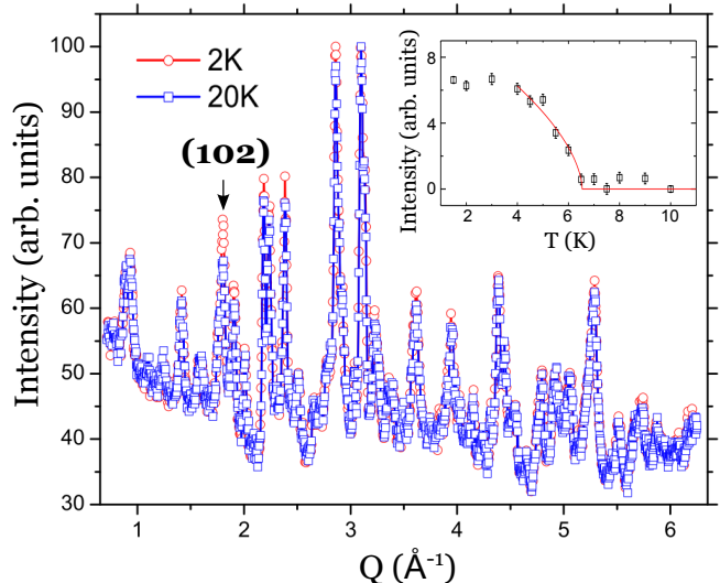
FIG. 3. (color online) The neutron powder diffraction data of \text{CeO}_{0.3}\text{F}_{0.7}\text{BiS}_2 below and above the magnetic phase transition temperature, T_M . Red circles represent 2K data and blue squares represents 20K data. Inset shows the summed intensity of the Q = (102) Bragg peak as a function of temperature. Red line represent the power law fit down to 4K.
