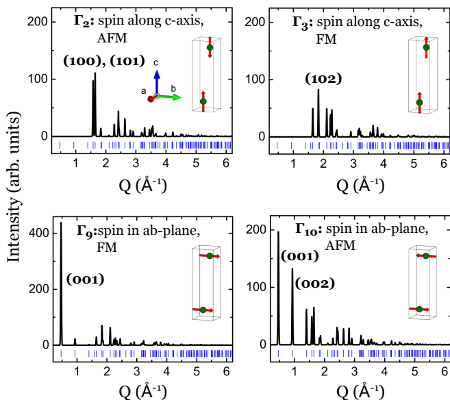
FIG. 4. (color online) Group theoretical analysis on the possible magnetic structures and their simulated neutron scattering intensities. Most prominent Bragg peaks are indicated in each panel. Group analysis was done using the program SARAh 62 and the number of IRs follows Kovalev's notation. Insets illustrate the corresponding magnetic order of the Ce moments for each IR.
