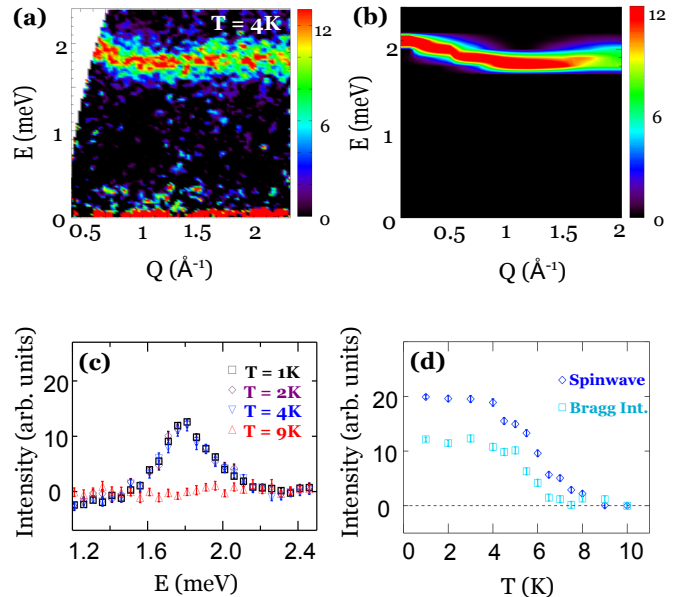
FIG. 6. (color online) (a) The contour map of measured inelastic neutron scattering intensity in reciprocal wave vector ( Q ) and energy transfer ( E ) space. (b) Simulated spin excitation spectrum in Q - E space. (c) Inelastic neutron scattering intensities along energy transfer at different temperatures. Intensities shown are summed over 0.5 \text{ \AA}^{-1} \leq Q \leq 1 \text{ \AA}^{-1} . (d) Temperature dependence of integrated intensities around magnetic excitation and magnetic Bragg peak Q = (102) . The T -dependence of the magnetic excitation was obtained by integrating the intensity over Q from 0.5 to 2.0 \text{\AA}^{-1} and over energy transfer from 1.5 to 2.5 meV. All figures shown here are background subtracted by the data obtained at T = 10 \text{ K} .
