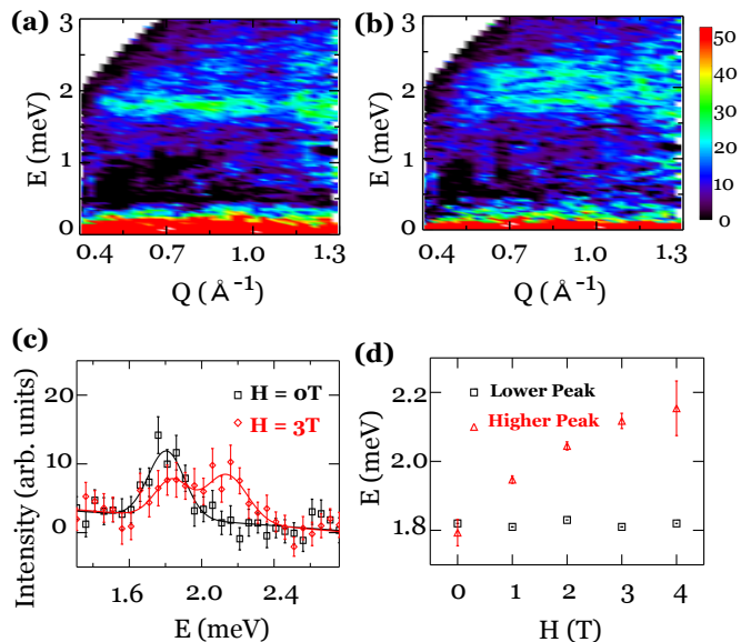
FIG. 7. (color online) The change of inelastic neutron scattering with external magnetic field is shown. (a) Spin excitation spectrum at H = 0 \text{ T} . (b) Spin excitation spectrum at H = 3 \text{ T} . (c) Inelastic neutron scattering intensities along energy transfer at different field of 0 \text{ T} and 3 \text{ T} . Scattering intensities are integrated over 0.5 \text{ \AA}^{-1} \leq Q \leq 1 \text{ \AA}^{-1} . (d) Gaussian fitted peak positions at different magnetic fields.
