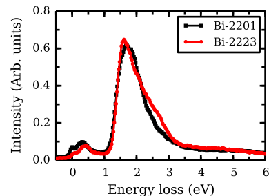
FIG. 1. (Color online) RIXS Spectra for Bi-2201 and Bi-2223 taken at \mathbf{Q} = (0.39, 0) . Magnetic, orbital and charge-transfer excitations are seen in energy ranges around 0 – 400 meV, 1 – 3 eV and 2 – 8 eV respectively (high energy scales > 6 eV are not shown).
