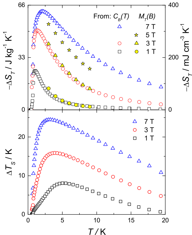
Figure 5: (Color online) Top: Isothermal entropy increment \Delta S_T for magnetic field increment, from zero to a given value, as labelled, computed from isothermal magnetization measurements and from heat capacity. Vertical axis reports units in \text{J kg}^{-1} \text{K}^{-1} (left) and volumetric \text{mJ/cm}^3 \text{K}^{-1} (right). Details about the absolute entropy in the text. Bottom: Adiabatic temperature increments, from zero field to a given value, as labelled, computed from heat capacity data. The abscissa is the initial temperature.
