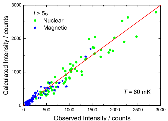
Figure 2: (Color online) Plot of the observed vs. calculated intensities for the ( I > 5\sigma ) magnetic and nuclear reflections.
