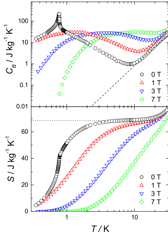
Figure 4: (Color online) Top: Heat capacity at applied magnetic field, C_B(T) . Dashed line: calculation of the phonon contribution. Bottom: Entropy S(T, B) deduced from heat capacity. Details in the text. Dotted line: infinite temperature limit for the molar magnetic entropy S_m/R(\infty) = \ln(2s + 1) for s = 7/2 .
