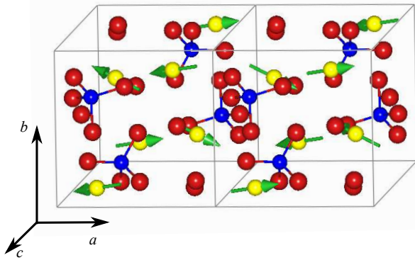
Figure 3: (Color online) Nuclear and magnetic structure at T = 60 mK. Red: O, blue: P, yellow: Gd. Green arrows: moments of Gd
