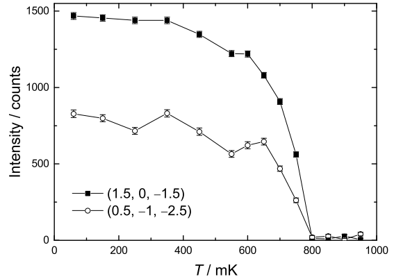
Figure 1: Variation of the intensity of the strong magnetic reflections (1.5, 0, -1.5) and (0.5, -1, -2.5) with temperature. Lines are guide to the eye.
