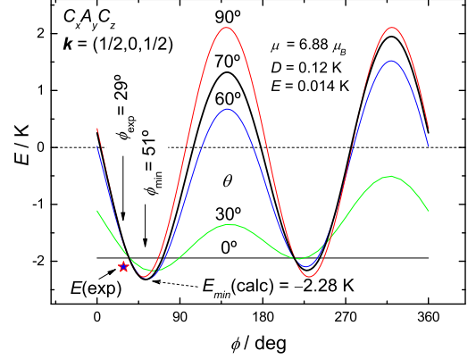
Figure 6: (Color online) Free energy per particle considering anisotropy and dipolar interactions for the C_x A_y C_z magnetic mode as a function of the azimuthal angle \phi for different \theta values defining the orientation of the moment at Gd1. The experimentally found magnetic energy is indicated.
