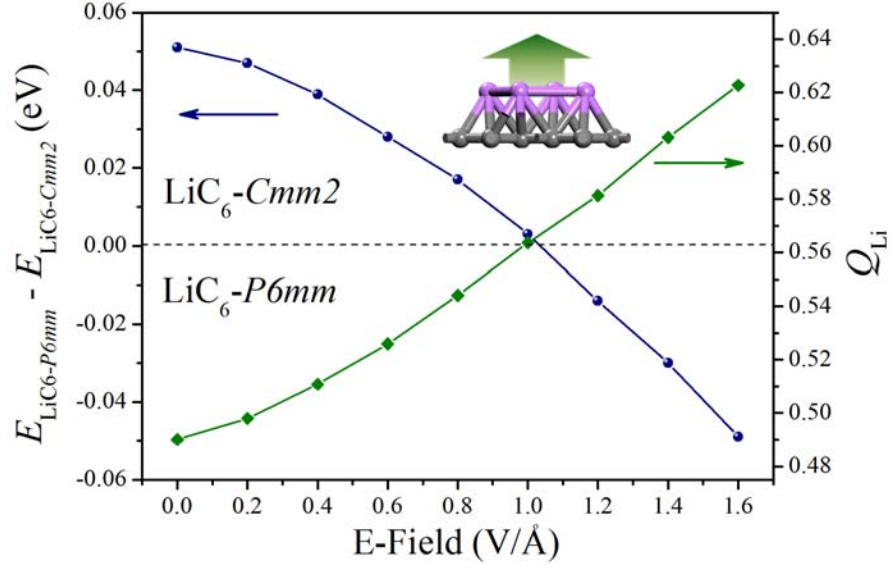
FIG. 6 Relative energies between the \text{LiC}_6\text{-}P6mm and \text{LiC}_6\text{-}Cmm2 per f.u. and average charges on each Li with respect to magnitude of the E-field. The inset arrow shows the direction of the E-field.
