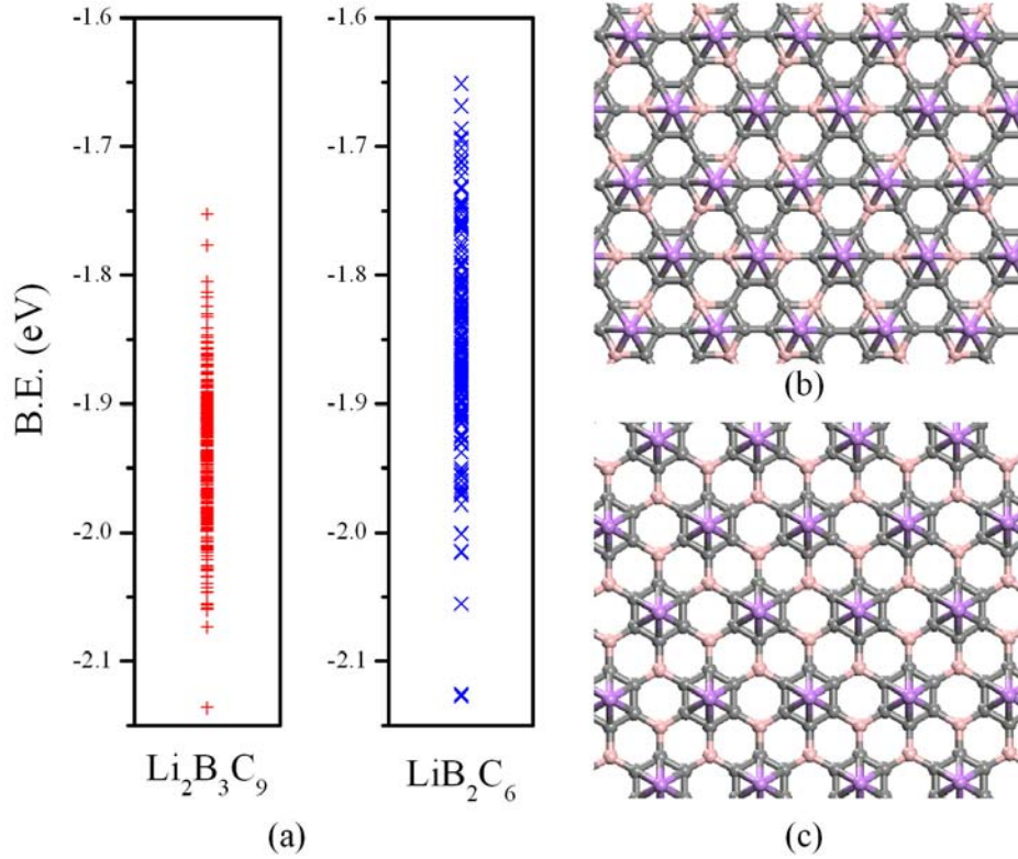
FIG. 7 (a) The calculated binding energy (B.E.) per Li atom of \text{Li}_2\text{B}_3\text{C}_9 and \text{LiB}_2\text{C}_6 obtained during the PPSO search. The ground state geometry of (b) \text{Li}_2\text{B}_3\text{C}_9 and (c) \text{LiB}_2\text{C}_6 .
