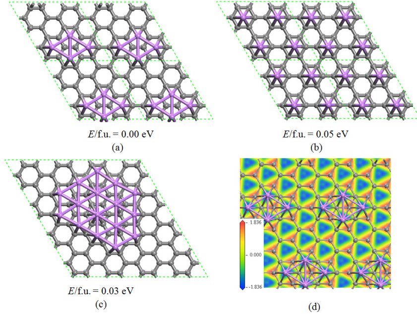
FIG. 2 Structures and relative energies of \text{LiC}_6 with Li atoms forming (a) a \text{Li}_4 cluster ( \text{LiC}_6 - Cmm2 ), (b) uniformly distributed Li ( \text{LiC}_6 - P6mm ), and (c) a \text{Li}_{16} cluster. In (d) we show the redistribution of electron density function in 2D slice form (in \text{e}/\text{\AA}^3 ). Grey and magenta spheres represent C and Li atoms, respectively. Green dashed lines outline simulated supercell.
