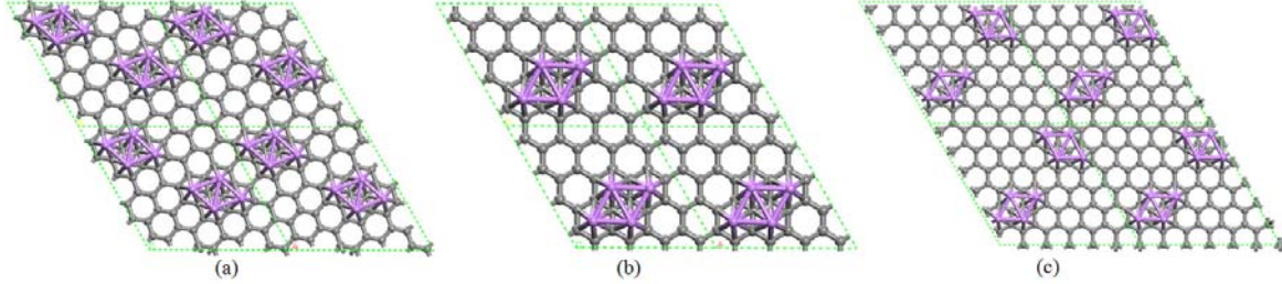
FIG. 3 Geometric structure of optimal (a) \text{LiC}_7 , (b) \text{LiC}_8 , and (c) \text{LiC}_9 .
