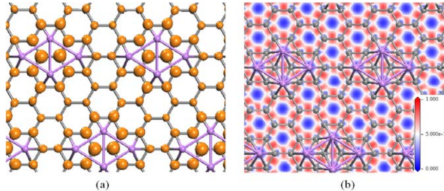
FIG. 5 (a) Charge density isosurface ( 0.01 \text{ e}/\text{\AA}^3 ) of the partially occupied bands and (b) 2D slice of ELF of \text{LiC}_6 .
