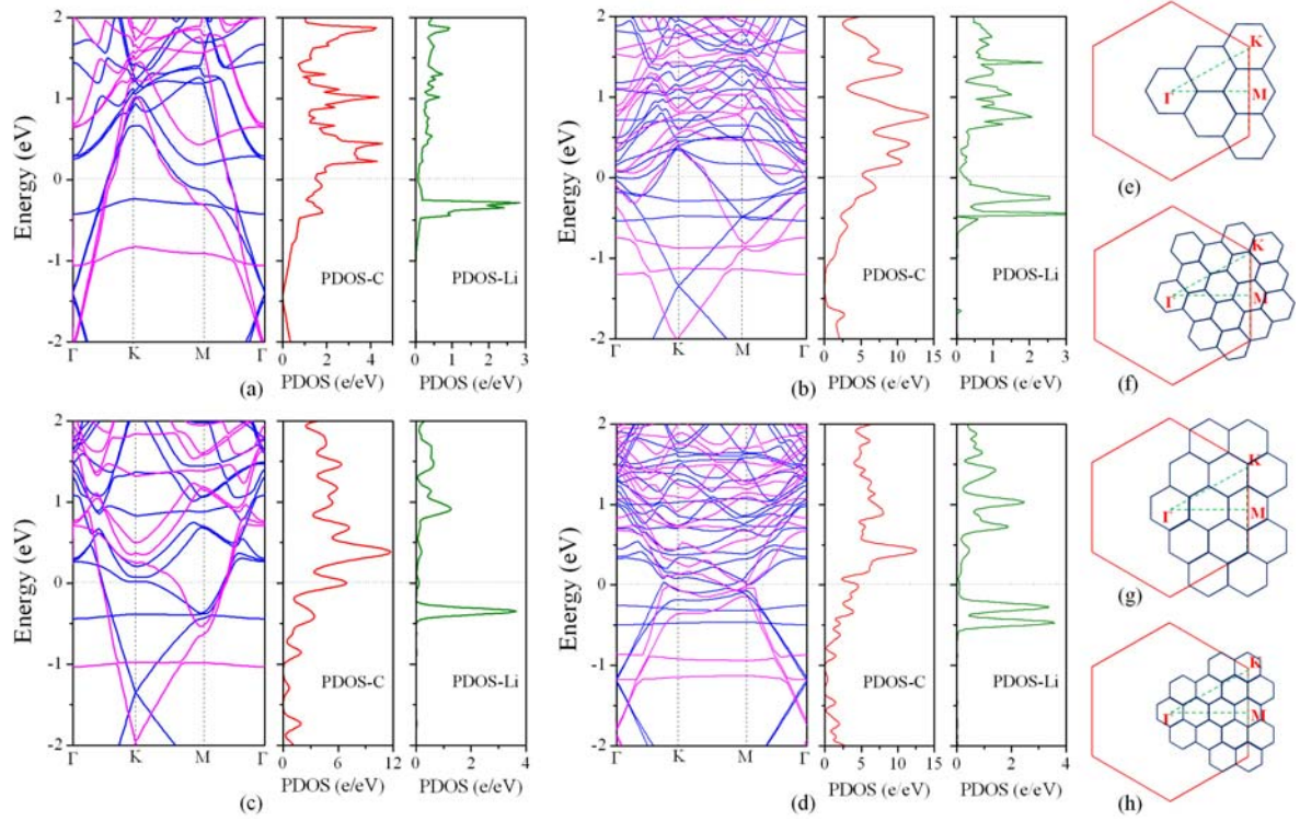
FIG. 4 Band structure and PDOS of (a) \text{LiC}_6 , (b) \text{LiC}_7 , (c) \text{LiC}_8 , and (d) \text{LiC}_9 . Blue and magenta curves in the band structure plots represent results obtained from GGA-PBE and hybrid functional HSE06, respectively. The PDOS curves are computed using the GGA-PBE functional. Momentum space folding of the simulating supercells for (e) \text{LiC}_6 , (f) \text{LiC}_7 , (g) \text{LiC}_8 , and (h) \text{LiC}_9 are also shown. Red hexagon represents the first Brillouin zone of the graphene unit cell, while dark blue hexagons are the first Brillouin zone of the simulated supercell.
