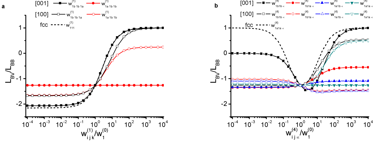
FIG. 3. (color online) Drag ratio L_{BV}/L_{BB} of a model alloy under an elementary strain \varepsilon_{33} as a function of (a) the different frequencies corresponding to w_{111}^{(1)} in the fcc structure, (b) the different frequencies corresponding to w_{11\infty}^{(4)} in the fcc structure. Filled symbols correspond to fluxes along the [001] direction, empty symbols to fluxes along the [100] or [010] direction. The corresponding ratio in the fcc structure is indicated by a dashed line.
