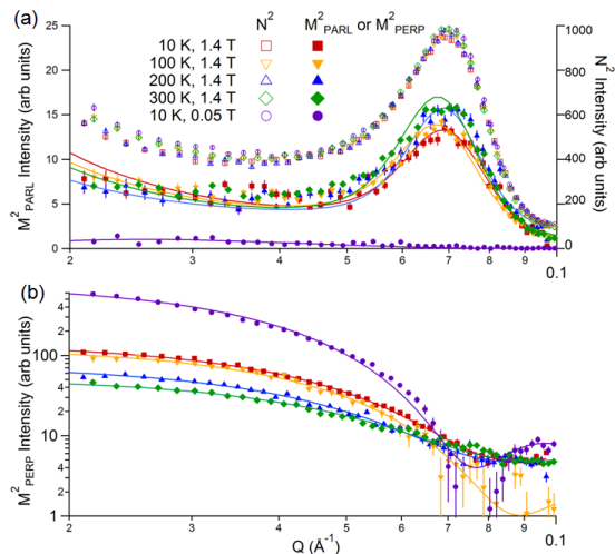
FIG. 3. (Color online.) (a) Data for N^2 and M_{PARL}^2 vs Q and (b) M_{PERP}^2 vs Q for a variety of temperatures in 1.4 T, scaled to a N^2 Bragg peak height of 1000. Data for 10 K in a remanent field of \approx 0.05 T are also shown. Solid lines in (a) are for a close-packed array of FCC magnetic spheres with \approx 13\% standard deviation in spacing distance whereas for (b) are for simple spheres of diameter 10.5 \text{ nm} \pm 0.4 \text{ nm} . Error bars in the plot denote standard uncertainties.
