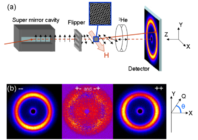
FIG. 2. (Color online.) (a) Experimental setup includes a polarizing supermirror and RF or conventional flipper to select the incident spin state and a ^3\text{He} cell with in-situ NMR flipper to select the scattered spin state. The scattering pattern is collected on a 2D detector. (b) Corrected 2D SANS images for 200 K, 1.4 T.
