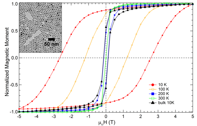
FIG. 1. (Color online.) Hysteresis loops for \text{CoFe}_2\text{O}_4 nanoparticle assemblies at 10, 100, 200, and 300 K. The 10 K hysteresis loop for bulk \text{CoFe}_2\text{O}_4 is shown for comparison. Inset shows TEM image of as-grown particles.
