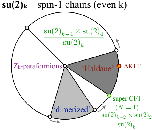
FIG. 9: (color online) Phase diagram of the even- k anyonic su(2)_k spin-1 chain in a projector representation (9) where J_1 = -\sin(\theta_{2,1}) and J_2 = \cos(\theta_{2,1}) . The locations of the phase boundaries correspond to the case k = 6 . Some of the phase boundaries move with increasing (even) k ; the arrows indicate the direction of the change.
