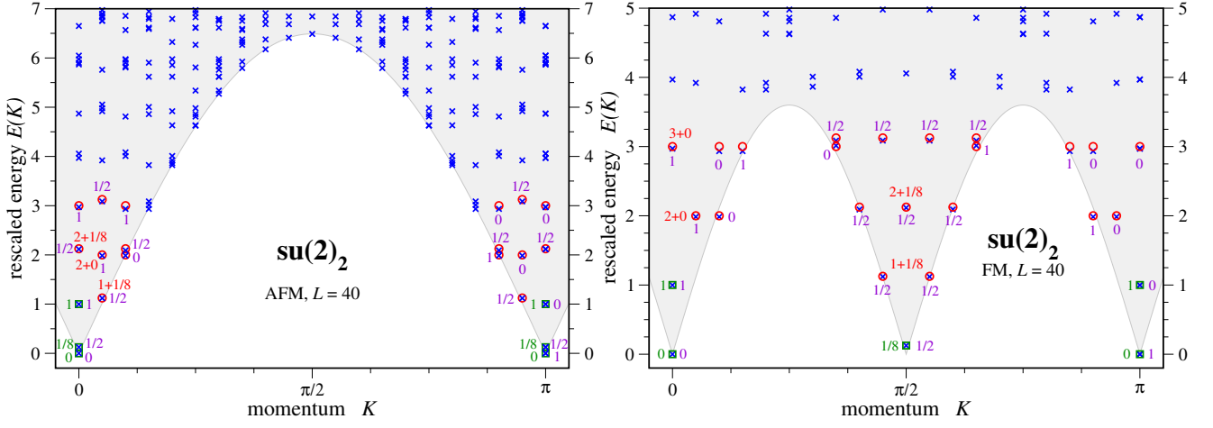
FIG. 17: (color online) The su(2)_2 spin-1/2 chain: Energy spectra have been rescaled to match the conformal field theory prediction given in Eq. (22). Green squares indicate the location of the primary fields, red circles specify the descendant fields. The topological symmetry sector is indicated by the violet index. Data shown is for system size L = 40 .
