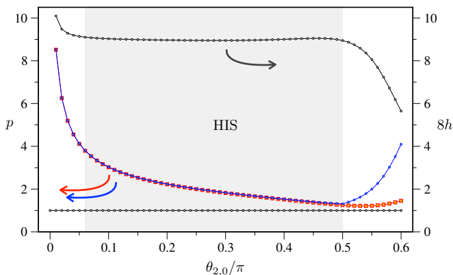
FIG. 16: Numerical estimate (system size L = 20 ) of parameter p from the eigenenergies that are associated with operators with scaling dimensions 1/2p (red squares) and 4/2p (blue dots) in the HIS gapless phase. The black dots correspond to the scaling dimension of the fields with dimensions h = 1/8 and h = 9/8 multiplied by eight, as obtained from exact diagonalization. The shaded region indicates the range of \theta_{2,0} for which the latter dimension lies between 8.9 < 8h < 9.1 .
