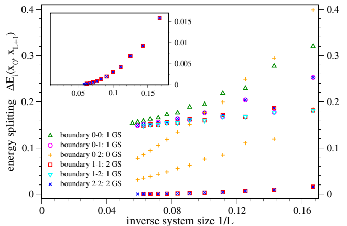
FIG. 8: The eigenenergies \Delta E_i(x_0, x_{L+1}) := E_i(x_0, x_{L+1}) - E_0(x_0, x_{L+1}) ( i \geq 1 ) of the \text{su}(2)_5 anyonic spin-1 chain with fixed boundaries x_0 and x_{L+1} as a function of 1/L at \theta_{2,1} = -0.01\pi . The legend at the lower left side indicates the values of x_0 and x_{L+1} . The energy E_0(x_0, x_{L+1}) is the lowest energy and not necessarily a ‘ground state energy’. For x_0 = x_{L+1} = 1 , and for x_0 = x_{L+1} = 2 , there are two almost degenerate zero-energy states, and \Delta E_1(x_0, x_{L+1}) corresponds to the finite-size splitting of the two ground states that decays exponentially with system size (see the inset).
