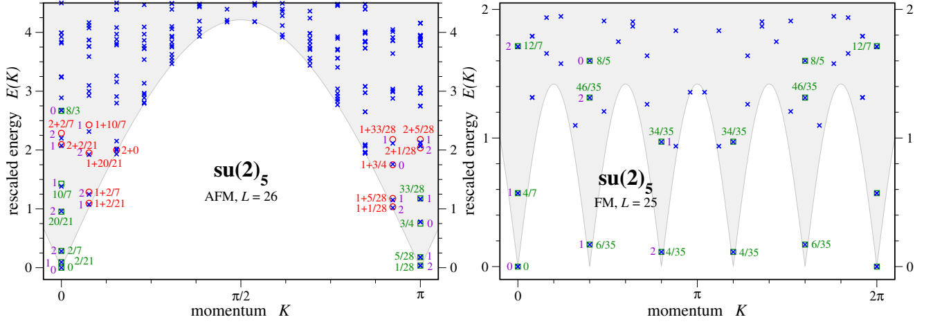
FIG. 19: (color online) The su(2)_5 spin-1/2 chain: Energy spectra have been rescaled to match the conformal field theory prediction given in Eq. (22). Green squares indicate the location of the primary fields, red circles the descendant fields. The topological symmetry sector is indicated by the violet index. Data shown is for system size L = 26 and L = 25 , respectively.
