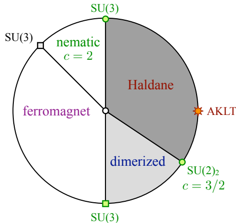
FIG. 3: (color online) Phase diagrams of the ordinary SU(2) spin-1 chain in a projector representation (9) with J_1 = -\sin(\theta_{2,1}) and J_2 = \cos(\theta_{2,1}) .
