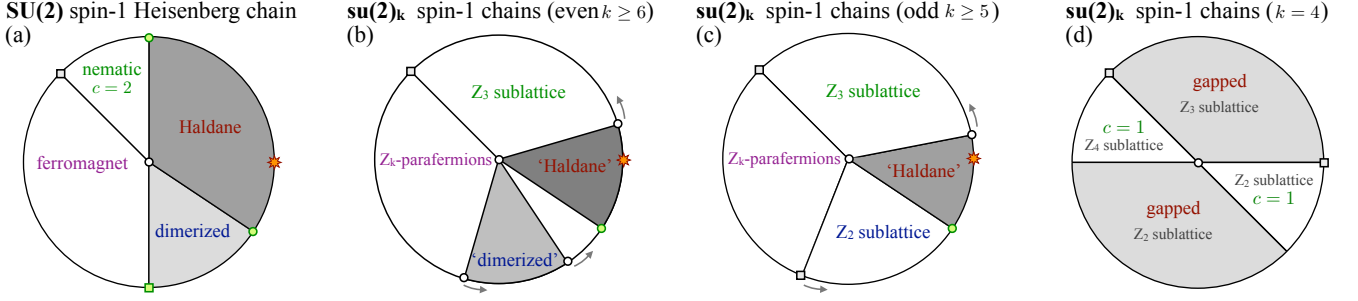
FIG. 20: Phase diagrams of the various spin-1 models considered in the paper: (a) the bilinear-biquadratic spin-1 Heisenberg chain, (b) the generic even k \geq 6 anyonic spin-1 chain, (c) the generic odd k \geq 5 anyonic spin-1 chain, (d) the special case k = 4 .
