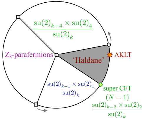
FIG. 4: (color online) Phase diagrams of the anyonic \text{su}(2)_k spin-1 chain with odd k in a projector representation (9) where J_1 = -\sin(\theta_{2,1}) and J_2 = \cos(\theta_{2,1}) . With increasing (odd) index k \geq 5 the phase boundaries move as indicated by the arrows.
