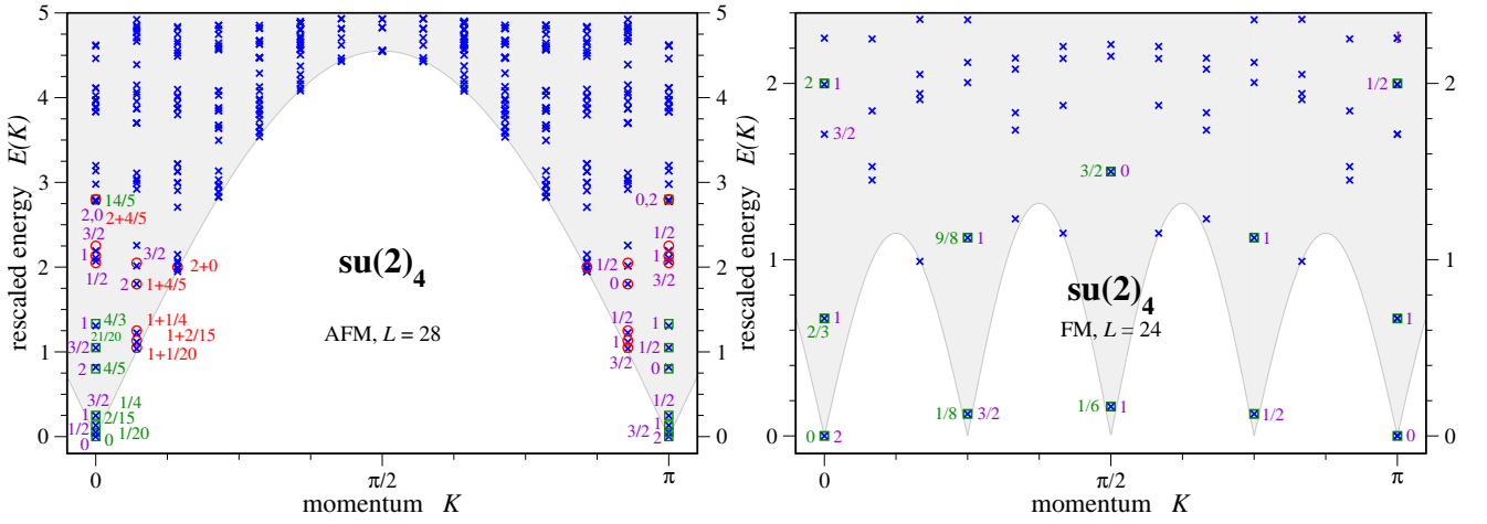
FIG. 18: (color online) The su(2)_4 spin-1/2 chain: Energy spectra have been rescaled to match the conformal field theory prediction given in Eq. (22). Green squares indicate the location of the primary fields, red circles specify the descendant fields. The topological symmetry sector is indicated by the violet index. Data shown is for system size L = 28 and L = 24 .
