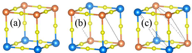
FIG. 1. (Color online) The three stacking configurations of perovskite SLs (period n = 1 ) studied here: (a) (001); (b) (011); (c) (111). Blue and brown balls are the transition metals, such as Ni and Mn, while the yellow balls are the oxygens. The A-site cation, e.g. La, is not shown.
