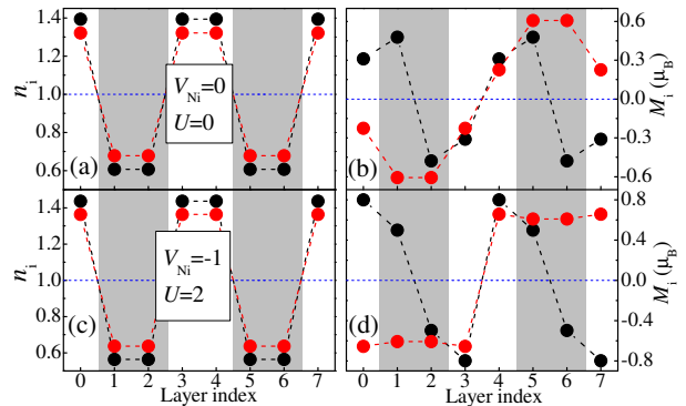
FIG. 7. (Color online) The profiles of e_g density (left) and e_g magnetization (right) for the n = 2 (111)-stacking superlattices with antiferromagnetically coupled \text{LaMnO}_3 layers. Black: \text{Mn}\uparrow\text{-Mn}\downarrow\text{-Ni-Ni-Mn}\uparrow\text{-Mn}\downarrow configuration; Red: \text{Mn}\downarrow\text{-Mn}\downarrow\text{-Ni-Ni-Mn}\uparrow\text{-Mn}\uparrow configuration. Gray region: LMO; White region: LNO. (a-b) V_{\text{Ni}} = 0 and U = 0 ; (c-d) V_{\text{Ni}} = -1 and U = 2 .
