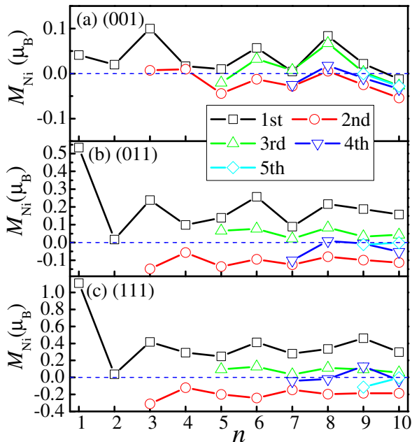
FIG. 6. (Color online) Magnetization profiles vs. distances from the interfaces. V_{\text{Ni}} = -1 , U = 2 are used. All notations are the same as in Fig. 4.
