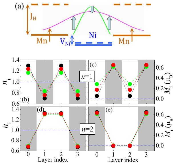
FIG. 2. (Color online) (a) Sketch of spin-filtered quantum confinement. Solid and broken lines denote the spin-up and spin-down levels, which are degenerate for Ni but split by J_H for Mn. V_{Ni} < 0 implies lower Ni levels. Pink and green curves are the sketch of spin-up and spin-down e_g electron densities. (b-e) The e_g -density profiles (left) and e_g magnetization (right) of SLs at V_{Ni} = U = 0 . Black: (001)-; Red: (011)-; Green: (111)-stacking SLs. Gray: LMO; White: LNO.
