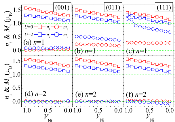
FIG. 5. (Color online) The Ni e_g electron densities (squares) and magnetization (circles) versus V_{\text{Ni}} for U = 0 (red) and U = 2 (blue). Top: n = 1 ; bottom: n = 2 . Left/middle/right: (001)/(011)/(111)-stacking.
