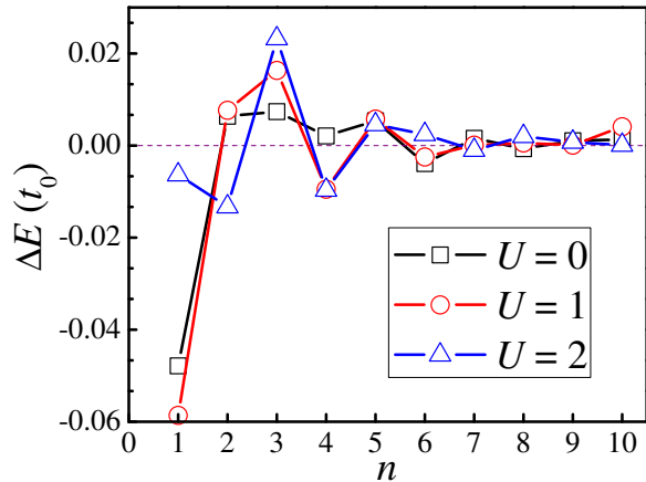
FIG. 8. (Color online) The energy differences per site between ferromagnetically coupled and antiferromagnetically coupled LMO layers ( E_{\text{AFM}} - E_{\text{FM}} ) in the (111)-stacking superlattices. V_{\text{Ni}} = -1 is used and U changes from 0 to 2.
