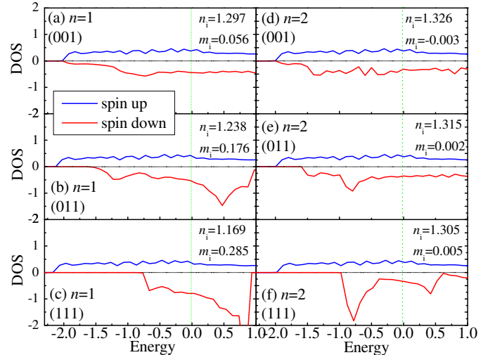
FIG. 3. (Color online) (a-f) Spin-resolved density of states of Ni. The Fermi level is at 0. Here U = 0 and V_{Ni} = 0 . Left: n = 1 ; Right: n = 2 . Upper: (001)-stacking; Middle: (011)-stacking; Lower: (111)-stacking. The e_g electron densities and magnetism are also shown.
