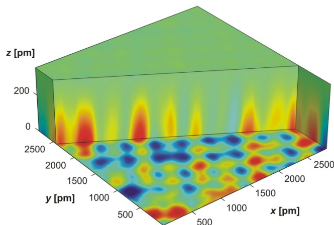
FIG. 3. (Color online) Three-dimensional representation of chemical interaction forces over an area of 2.89 \text{ nm} \times 2.89 \text{ nm} . The color scale ranges from -12 \text{ pN} (dark blue, least attractive) to +10 \text{ pN} (dark red, most attractive), with the average force at each height subtracted. 18,19 Note that the z -axis has been arbitrarily set to z = 0 \text{ pm} at the distance of closest approach, i.e., the displayed values do not coincide with the definition of the distance d in the simulations.
