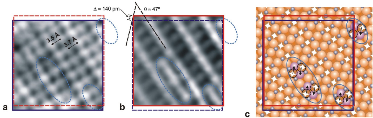
FIG. 4. (Color online) Simultaneous 3D-AFM and tunneling current measurements on Cu(100)-O ( 2.89 \text{ nm} \times 2.89 \text{ nm} ). (a) Horizontal force map cut from the data set shown in Figure 3 at the distance of closest approach. Circular maxima reveal the oxygen atoms' alternating spacing of 3.5 \text{ \AA}/3.7 \text{ \AA} . Total force contrast is 23 \text{ pN} ; dashed lines circle the locations of defects identified from the current map in Fig. 2b. (b) Tunneling current data displaying a ladder -type contrast as well as defects in the form of apparent nonmissing rows . The greyscale covers the range of 0\text{-}7 \text{ pA} (dark to bright). (c) Structural model of the imaged area, where defects formed through lateral movement of Cu2 atoms are highlighted. Comparing (a) and (b) reveals that the current and force images are offset by \approx 140 \text{ pm} .
