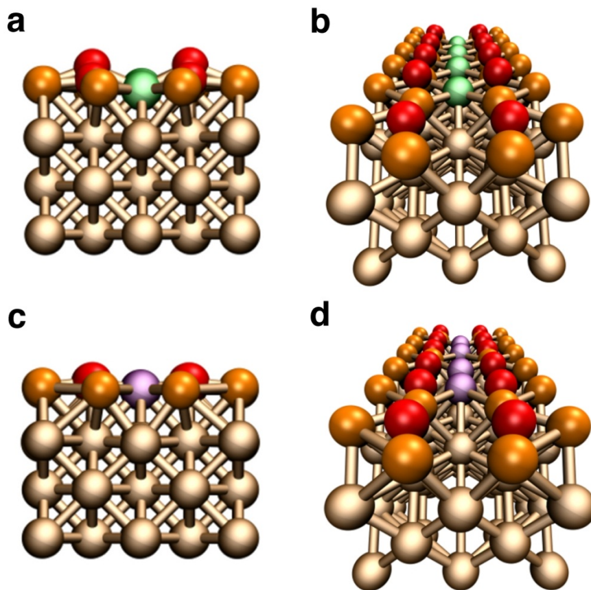
FIG. 8. (Color online) The 2\times 6 unit cell segment of the optimized Cu(100)-O surface oxide structure containing defect atoms in the missing row, with Cu atoms shown in gold, O atoms in red and sub-surface Cu slabs in dimmed gray. “Filled-row” and “displacement” Cu defects are colored green and purple respectively. (a) and (c) The vertical displacement of surface atoms around the defect-filled missing row seen in the x - z plane (side view), demonstrating the additional displacement of O atoms around the “filled-row” defects in comparison to the case of “displacement” defects. (b) and (d) The difference in O and Cu 2 atom lateral displacements towards the defect-filled missing row, perspective view.
