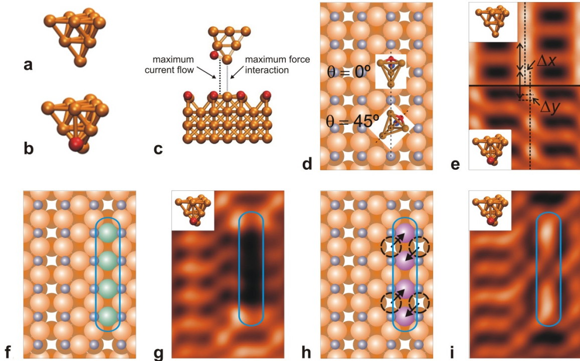
FIG. 7. (Color online) Tip and defect identification. (a) Clean Cu-terminated tip (side view). (b) Cu-terminated tip stabilized by an oxygen atom located at the side (“CuO tip”; side view). (c) Origin of the offset between force and current channels for the CuO tip: The oxygen atom close to the apex causes the current maximum to shift towards the direction of the oxygen, while the strongest force interaction remains with the apex atom. (d) Structural model for the defect-free surface; insets of tip models define the notation used to describe tip orientation. (e) Corresponding simulated STM signature, revealing a ladder-type contrast. The upper panel has been computed for a symmetric Cu tip, the bottom panel for a CuO tip with \theta = 45^\circ . The offsets resulting from tip asymmetry are highlighted. (f-g) Model and computed STM signature for a missing row partially filled with four Cu atoms (“filled-row defect”, represented by green spheres in blue enclosure). Simulations for a CuO tip with \theta = 45^\circ predict a dark row along the defect, in strong contrast to experimental results. (h) Energetically favorable defect model created by lateral displacement of Cu 2 atoms (purple spheres, highlighted by blue enclosure). For this “displacement defect”, distortions in the positions of the O atoms are minimal both in lateral and vertical directions. (i) Corresponding STM image calculated for a CuO tip with \theta = 45^\circ . The appearance of an apparent nonmissing row is clearly observed along the length of the defect. All current maps are calculated at a constant height of 450 pm and at a bias voltage of -0.4 V.
