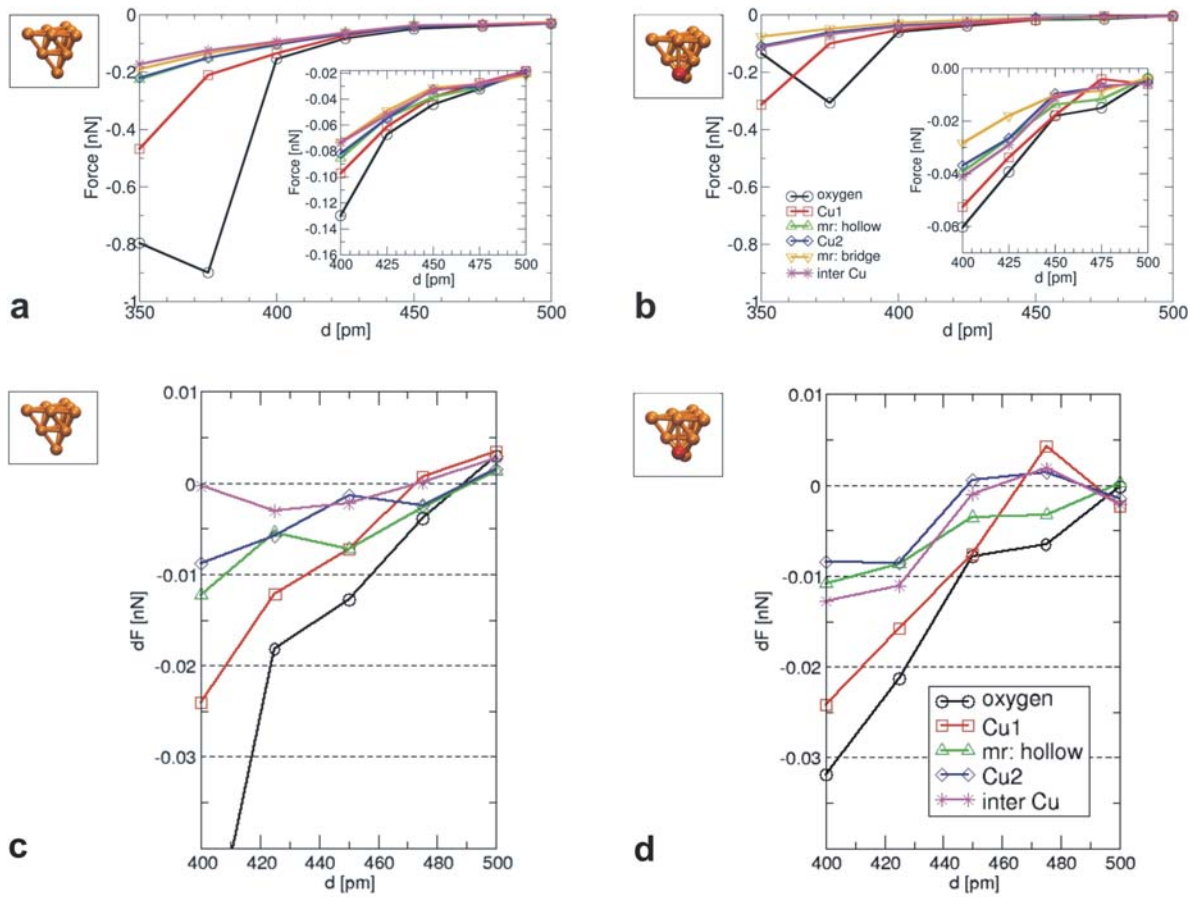
FIG. 6. (Color online) Force-distance curves computed for Cu (a) and CuO (b) tips (Insets: Zoom of the forces in the 400-500 pm distance range). (c) and (d) display, for Cu and CuO tips, the force difference (dF) between individual lattice sites and the missing row bridge site (mr:bridge) located between two Cu atoms on both sides of a missing row. A comparison with experimental force contrast reveals that the closest tip-sample distance during the experiments is 425-450 pm.
