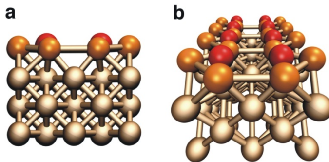
FIG. 2. (Color online) The 2 \times 4 unit cell segment of the optimized Cu(100)-O surface oxide structure, with Cu atoms shown in gold, O atoms in red, and sub-surface Cu slabs in dimmed gray. (a) The vertical displacement of surface atoms around the missing row feature seen in the x - z plane (side view). (b) The difference in O and Cu2 atom lateral displacements towards the missing row, perspective view.
