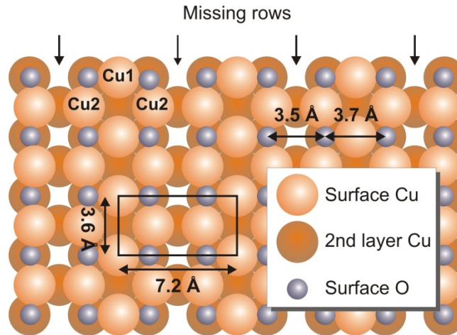
FIG. 1. (Color online) Missing-row model of the surface oxide layer on the Cu(100) surface. A rectangular unit cell, the positions of Cu1 and Cu2 atoms and the missing rows, as well as the alternating separation of O atoms are highlighted.
