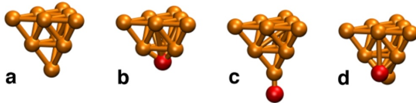
FIG. 5. (Color online) Probe tips considered in the calculations (perspective views with copper atoms in gold and oxygen atoms in red). (a) Cu-terminated tip; (b) O-terminated tip; (c) Dangling bond O tip; (d) O-adatom tip (“CuO tip”).
