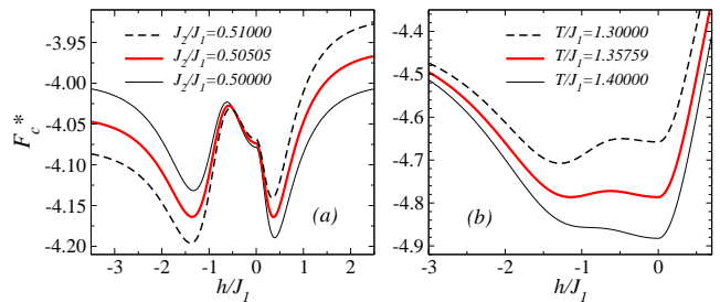
FIG. 6. (Color online) Free energy versus the external field parameter h in the 2 \times 2 cluster mean-field theory at and close to first-order transitions. Positive and negative h correspond to ferromagnetic and striped field patterns, respectively. (a) shows results for different coupling ratios at and close to the ferromagnetic–striped transition at fixed T/J_1 = 1 , and (b) shows the behavior for temperatures at and close to the stripe–paramagnetic transition at g = 0.55 .
