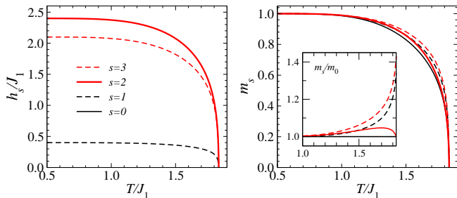
FIG. 5. (Color online) Self-consistent variational field parameters (left) and the corresponding induced stripe magnetizations (right) versus temperature obtained using a 4 \times 4 cluster at J_2/J_1 = 0.7 . The inset of the right panel shows the ratio of the shell magnetizations for shells s > 0 to the one with s = 0 (center of the cluster). The shell index s follows the convention illustrated in Fig. 3.
