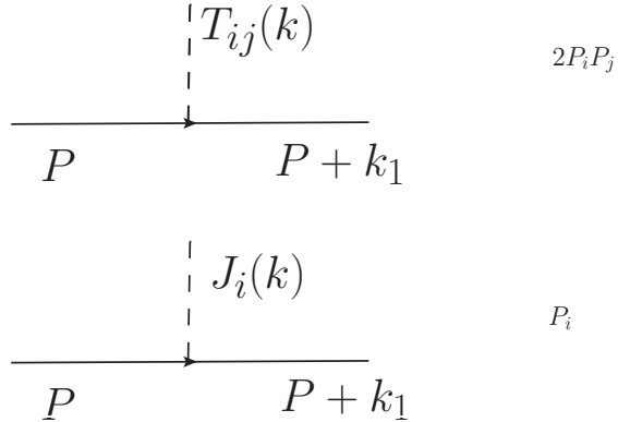
Figure 4. Momentum structure of the stress tensor (top) and current vertex (bottom) after contracting with transverse and traceless polarization tensors.
