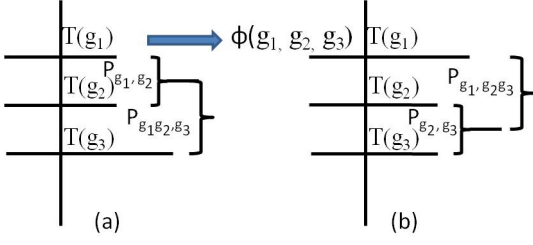
FIG. 3. Different ways to reduce combination of T(g_3) , T(g_2) and T(g_1) into T(g_1g_2g_3) . Only the right projection operators are shown. Their combined actions differ by a phase factor \phi(g_1, g_2, g_3) .
