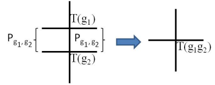
FIG. 2. Reduce combination of T(g_2) and T(g_1) into T(g_1 g_2) .
