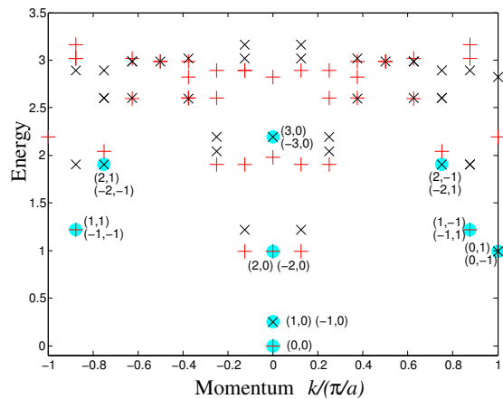
FIG. 1. Low energy states of XY model H'_2 (Eqn. (3)). x -axis is lattice momentum k/(\pi/a) , where a is the lattice spacing. y -axis is energy with ground state energy set to 0 and first excited state energy normalized to 1/4. + represents positive \mathbb{Z}_2 quantum number and \times represents negative \mathbb{Z}_2 quantum number. The total angular momentum l and winding number m are labeled as (l, m) for each primary field, represented by the shaded + or \times . States in the same conformal tower have the same l and m .
