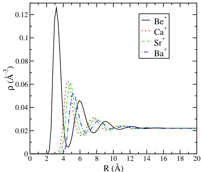
FIG. 4: (Color online) Calculated ground state liquid densities as obtained from DFT calculations for \text{Be}^+ , \text{Ca}^+ , \text{Sr}^+ and \text{Ba}^+ are shown.
