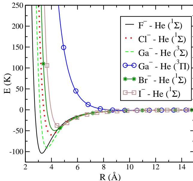
FIG. 1: (Color online) Calculated pair potentials for halogen anions interacting with a ground state helium atom are shown. Note that \text{Ga}^- is non-spherical as two possible electronic states ( \Sigma and \Pi ) arise from the outmost atomic s and p orbitals on He and Ga, respectively.
