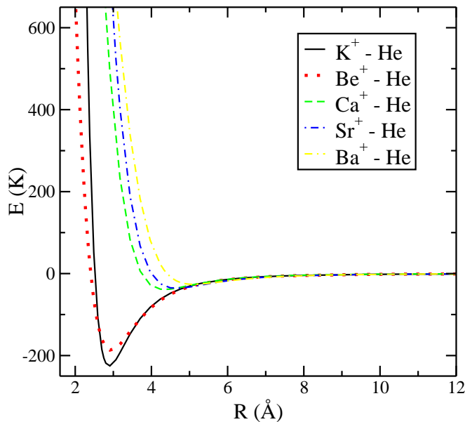
FIG. 2: (Color online) Calculated pair potentials for the cations K^+ , Be^+ , Ca^+ , Sr^+ and Ba^+ interacting with a ground state helium atom are shown.
