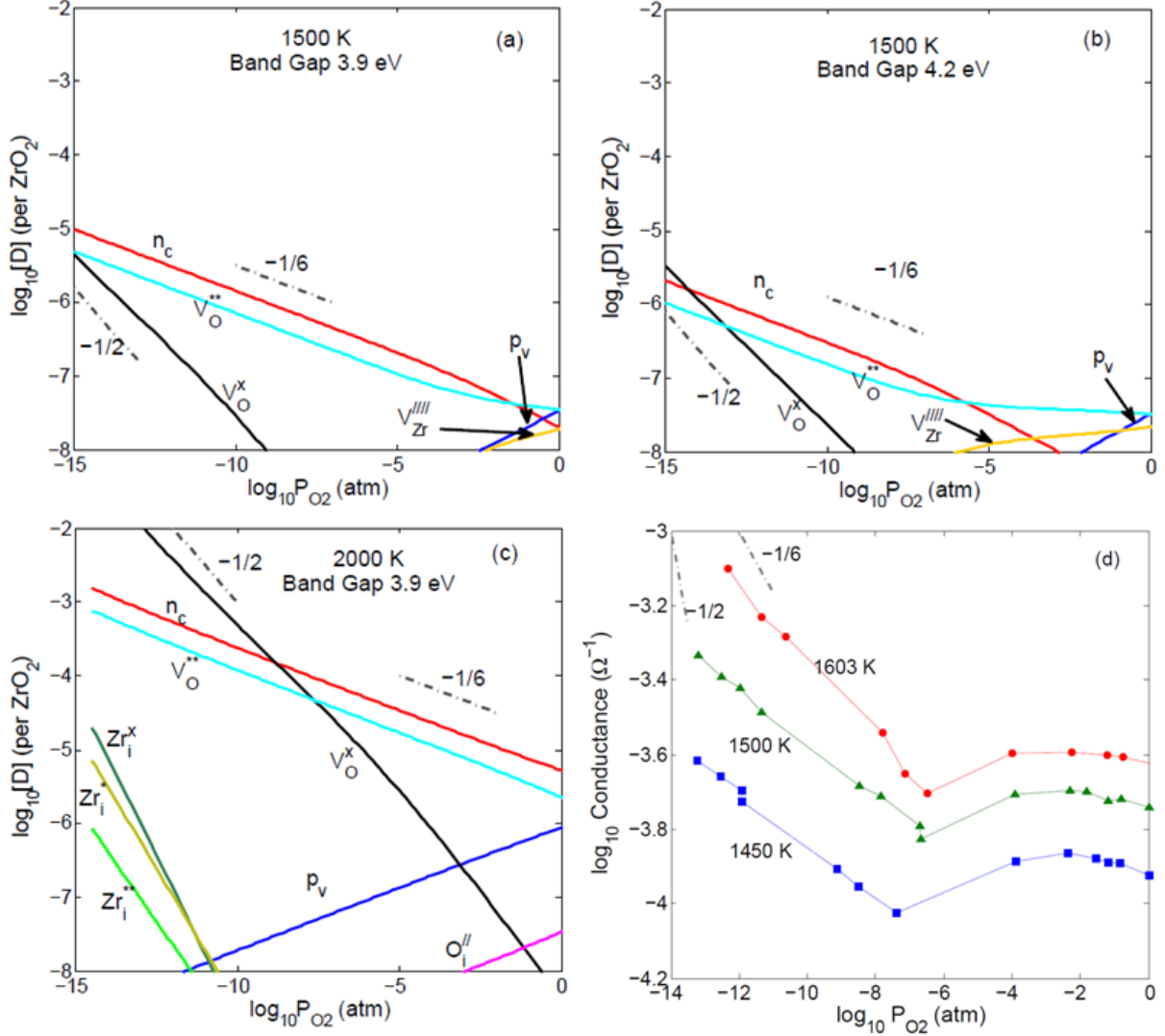
FIG. 4. (Color online) Calculated Kröger-Vink diagram for tetragonal ZrO 2 at (a) 1500 K using the DFT predicted band gap of 3.9 eV, (b) 1500 K using the experimental band gap of 4.2 eV, (c) 2000 K using the DFT predicted band gap. (d) Conductivity measurements on tetragonal zirconia by Kofstad and Ruzicka. 23 In a,b,c only the defects that have concentrations greater than 10 -8 are shown. The dash-dot lines in a,b,c,d are guide for the eye showing the (-1/2) and (-1/6) slopes.
