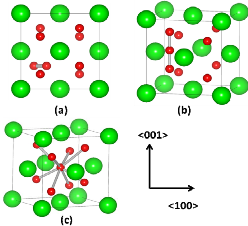
FIG. 2. (Color online) Examples of the oxygen interstitial structures considered. (a) \langle 110 \rangle dumbbell, (b) \langle 001 \rangle crowdion, (c) the octahedral site. Green (large) and red (small) balls represent zirconium and oxygen, respectively. The sticks are guide for the eye and have no particular physical meaning. This figure was generated using the visualization software VESTA. 56
