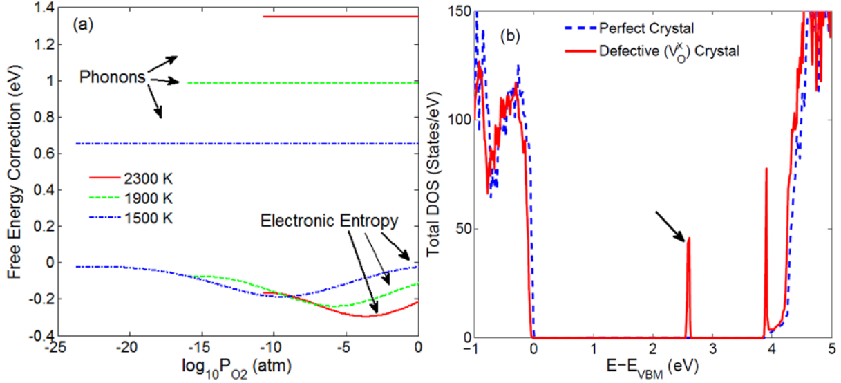
FIG. 1. (Color online) (a) Corrections to the free energy of formation of the neutral oxygen vacancy due to the change in the phonon vibrations and the electronic entropy in the solid. (b) The total electronic density of states (DOS) for tetragonal ZrO_2 in a perfect supercell and in a supercell with a neutral oxygen vacancy. The arrow in (b) indicates the electronic state in the gap due to the neutral oxygen vacancy that enhances the electronic entropy of the defect. The position and magnitude of the resonance (in (a)) between \mu_F and the defect state (in (b)) depends on temperature and oxygen partial pressure.
