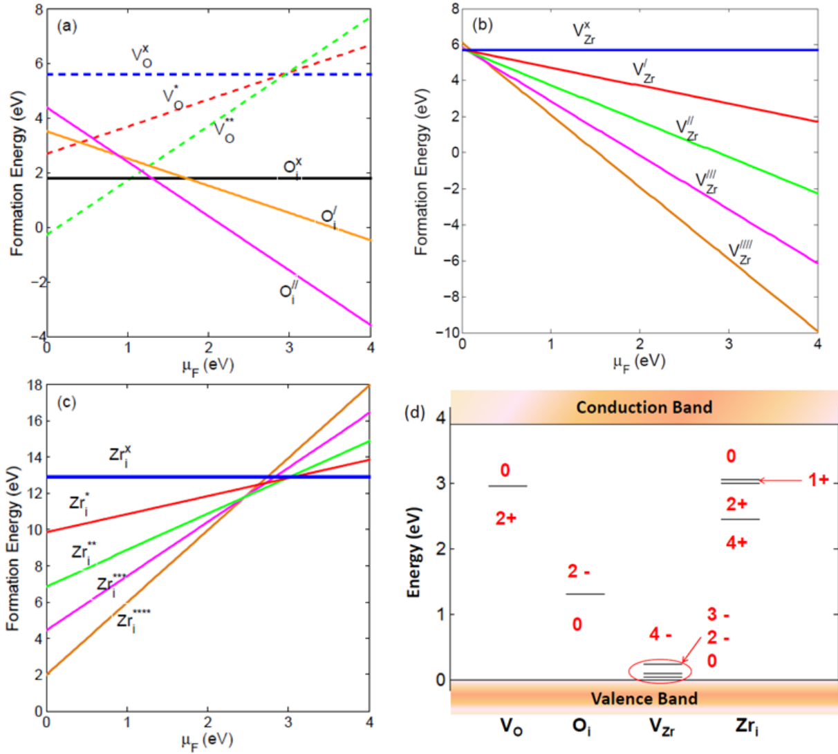
FIG. 3. (Color online) Defect formation energies as a function of the electron chemical potential. (a) Oxygen defects. (b) Zirconium vacancies. (c) Zirconium interstitials. (d) The thermodynamic transition levels for the native defects determined from (a,b,c).
