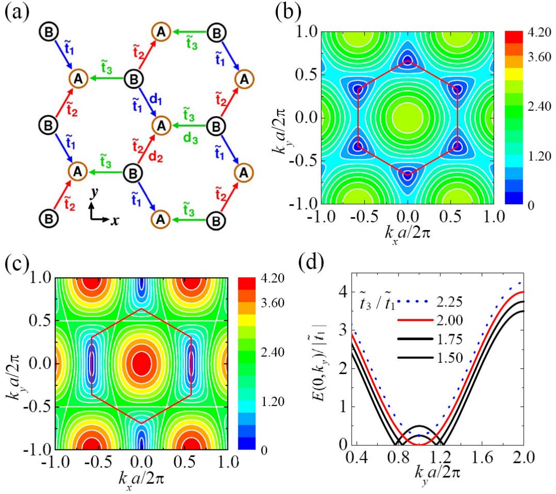
Figure 4. (color online) (a) Honeycomb lattice geometry with three nearest-neighbor hopping matrix elements ( \tilde{t}_1 , \tilde{t}_2 , \tilde{t}_3 ) and three nearest-neighbor relative positions ( \vec{d}_1 , \vec{d}_2 , \vec{d}_3 ). A and B denote two sublattices. (b) 2D plots of the energy dispersion, E(k_x, k_y)/|\tilde{t}_1| with three equivalent hoppings ( \tilde{t}_1 = \tilde{t}_2 = \tilde{t}_3 ). (c) 2D plots of the energy dispersion E(k_x, k_y)/|\tilde{t}_1| with \tilde{t}_1 = \tilde{t}_2 and \tilde{t}_3 = 2.1 \times \tilde{t}_1 . (d) The dispersion E(0, k_y)/|\tilde{t}_1| for various values of \tilde{t}_3/\tilde{t}_1 . In (d), the energy-gap opening can be clearly seen when \tilde{t}_3/\tilde{t}_1 > 2 . In (b)-(d), the lattice constant a is \sqrt{3} times the C-C bond length.
