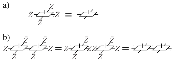
FIG. 5. \mathbb{Z}_2 -invariant tensor network. a) A tensor is called \mathbb{Z}_2 -invariant if it is invariant under some \bar{Z} applied to all virtual indices, where \{1, \bar{Z}\} forms a representation of \mathbb{Z}_2 . b) \mathbb{Z}_2 -invariance is stable under concatenation of tensors.
