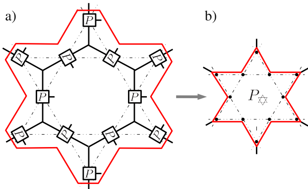
FIG. 8. Definition of the tensor P_{\star} . a) P_{\star} is obtained by blocking 12 tensors P with 6 triangular “bond tensors” E ; it maps 6 virtual qutrits to 12 physical qubits. b) Effective depiction of the tensor P_{\star} .
