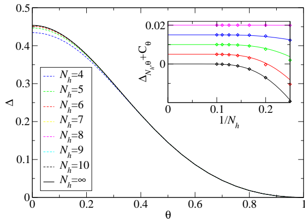
FIG. 12. Gap of the transfer operator \Delta as a function of \theta along the RVB-dimer interpolation for N_h = 4, \dots, 10 and PBC. As the transfer operator is parity preserving (changing) for N_h even (odd), it has two (almost) degenerate largest eigenvalues corresponding to different parity sectors (for N_h even, there is an exponentially small splitting in N_h ); the gap \Delta shown is the ratio of the third eigenvalue and the average of the two maximal eigenvalues. The data for N_h = \infty has been obtained by fitting the data for N_h = 6, \dots, 10 with a + b \exp(-cN_h) . The inset shows the fit for \theta = 0, 0.1, 0.2, 0.3, 0.5 (from bottom to top, the curves have been shifted vertically in the plot); note that the two right-most data points have not been used for the fit.
