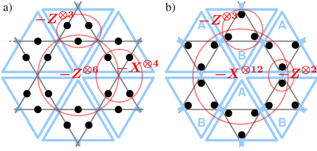
FIG. 19. a) Tensor network and Hamiltonian for the toric code on the kagome lattice. Two types of terms ensure the parity constraints over the triangular and hexagonal plaquettes, while the vertex term enforces an equal weight superposition of all even parity configurations. Note that the -Z^{\otimes 3} acting on the triangles can be understood as enforcing each individual tensor to be in the correct subspace. b) Hamiltonian terms obtained by transforming each tensor unitarily into a projector onto the symmetric subspace. Z^{\otimes 3} still enforces that the tensor is in the correct subspace; further, there is a Z^{\otimes 2} at each vertex enforcing equality of the adjacent qubits—translated to the dimer state, this will enforce that there is exactly one singlet adjacent to each vertex. Finally, the X^{\otimes 12} term around the hexagon makes sure that all such configurations appear with equal weight—it will make the dimer configurations resonate in the orthogonal RVB state. (Note that this model can also be understood as a toric code model on a “decorated” hexagonal lattice with two sites per edge and a vertex between, and X stabilizers around plaquettes and Z stabilizers across vertices.)
