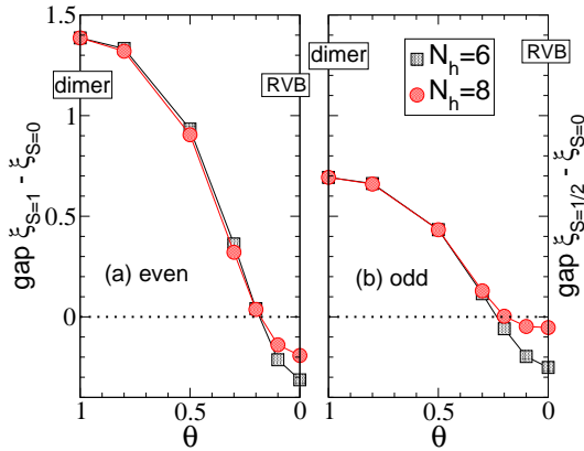
FIG. 16. Gap between the lowest S = 1 and S = 0 state (left) and S = \frac{1}{2} and S = 0 state (right) of the entanglement Hamiltonian for the dimer-RVB interpolation for N_h = 6, 8 .
