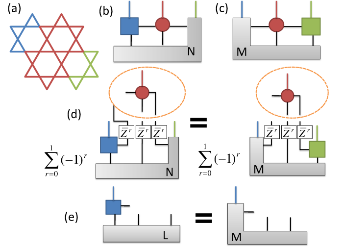
FIG. 22. Graphical proof of the intersection property for the case h_1 + h_2 where h_1 acts on the 3 stars colored in blue-red in (a) and h_2 acts on those colored in red-green. It is easy to see that, by separating the common part (2 red stars) and the rest, with the convention that the common part has all outgoing indices of type P , \ker h_1 \otimes \mathcal{H}_{\text{green}} is given by figure (b), where N is an arbitrary tensor, whereas \mathcal{H}_{\text{blue}} \otimes \ker h_2 is given by figure (c), where M is arbitrary. Here \mathcal{H}_{\text{green}} and \mathcal{H}_{\text{blue}} represent the Hilbert spaces associated to the physical indices in the green and blue regions, respectively. As before, we have gathered together all virtual (as well as the physical) indices within each type of tensor. Given a state |\psi\rangle in the intersection of both kernels, there exist N and M such that |\psi\rangle can be expressed both in the form (b) and (c). In the equality (b)=(c) we invert the circle tensor, obtaining the equality given in figure (d). After that, we apply an auxiliary extra circle tensor, then the inverse of the red-green tensors (3 stars), which is also \mathbb{Z}_2 -injective by the previous section, and then trace the extra virtual system. Since one can assume wlog that both M and N have the symmetry \otimes \bar{Z} , we can also eliminate the sums. After all that we arrive at figure (e) for some tensor L . Substituting (e) in (c) gives the desired form for |\psi\rangle and hence the result.
