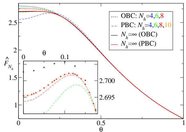
FIG. 13. The overlap change \hat{F}_{N_h} , Eq. (14), as a function of \theta for both open boundary conditions ( N_h = 4, 6, 8 ) and periodic boundary conditions ( N_h = 4, 6, 8, 10 ). The solid black and red line give the extrapolated data for N_h = \infty for open and periodic boundaries. The inset shows a zoom of the N_h = \infty data for \theta \leq 0.18 , where the black (red) crosses correspond to open (periodic) boundaries. The details of the scaling analysis are given in Fig. 14.
