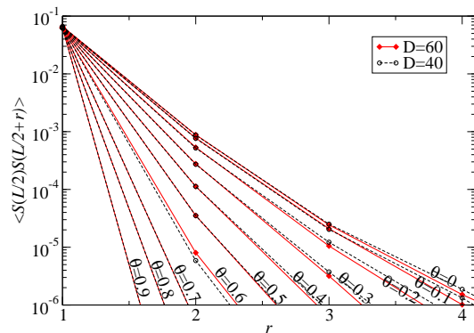
FIG. 11. Two-point correlations as a function of the distance for different values of \theta . The plot shows data for an infinite system where in the PEPS contraction, 14 the bond dimension has been truncated at D = 40 and D = 60 , respectively.
