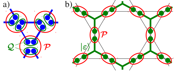
FIG. 18. Simplified PEPS construction for the RVB and dimer state. a) Start from the representation Fig. 17 and rewrite \mathcal{P}_4 in two layers, \mathcal{P}_4 = \mathcal{P}(\mathcal{Q} \otimes \mathcal{Q}) , Eq. (A4). The \mathcal{Q} act as indicated by the green circles, and make sure at most one singlet degree of freedom is kept; they thus return one qutrit each. \mathcal{P}_2 makes sure exactly one singlet is kept, which can come from either of the two \mathcal{Q} 's. b) The simplified PEPS construction: Applying three \mathcal{Q} 's to three bonds around a loop results in a state |\epsilon\rangle which holds at most one singlet, Eq. (A5), and which is placed across every triangle. Subsequently, \mathcal{P} is applied to pick one of the singlets at each vertex.
