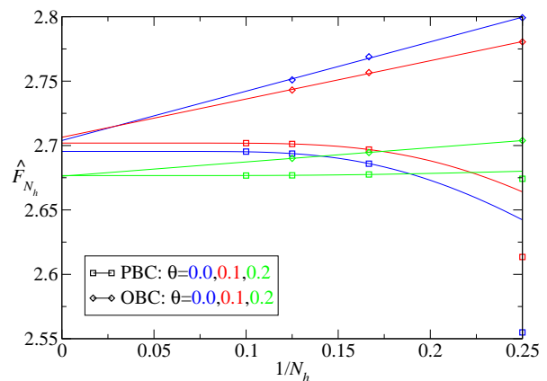
FIG. 14. Finite size scaling analysis for \hat{F}_{N_h} . The plot shows OBC and PBC data for \hat{F}_{N_h} . Due to the absence of boundary effects, the PBC data converges very quickly to the N_h = \infty value once N_h is beyond the correlation length. We have fitted the PBC data for N_h = 6, 8, 10 with a + b \exp(-cN_h) . The OBC data, on the other hand, has a 1/N_h leading term from the boundary; we have fitted the data for N_h = 4, 6, 8 with a + b/N_h . Note that the correction for the data points for OBC would most likely be concave, suggesting that the true N_h = \infty value is closer to the PBC data.
