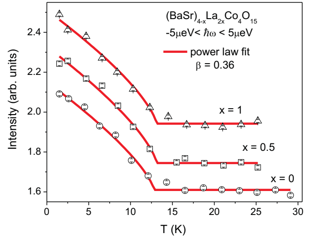
FIG. 6: Temperature dependence of the elastic scattering, from all three samples, integrated over the Q range 0.25 - 2\text{\AA}^{-1} . The solid line represents a power-law fit to the data.
