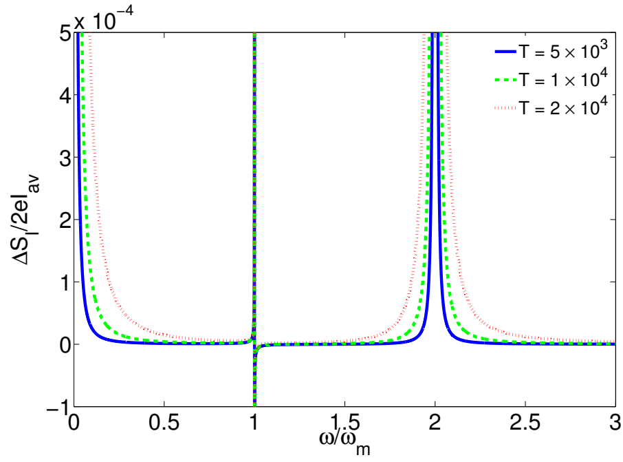
FIG. 5. (Color online) Dimensionless non-Poissonian current noise spectrum for \tilde{T} = 5 \times 10^3 , 1 \times 10^4 and 2 \times 10^4 . The remaining parameters are t_0 = 0.2 , \tilde{V} = 2 \times 10^4 , \tilde{\lambda} = 1 \times 10^{-3} , and \tilde{\Gamma}_0 = 5 \times 10^{-6} .
