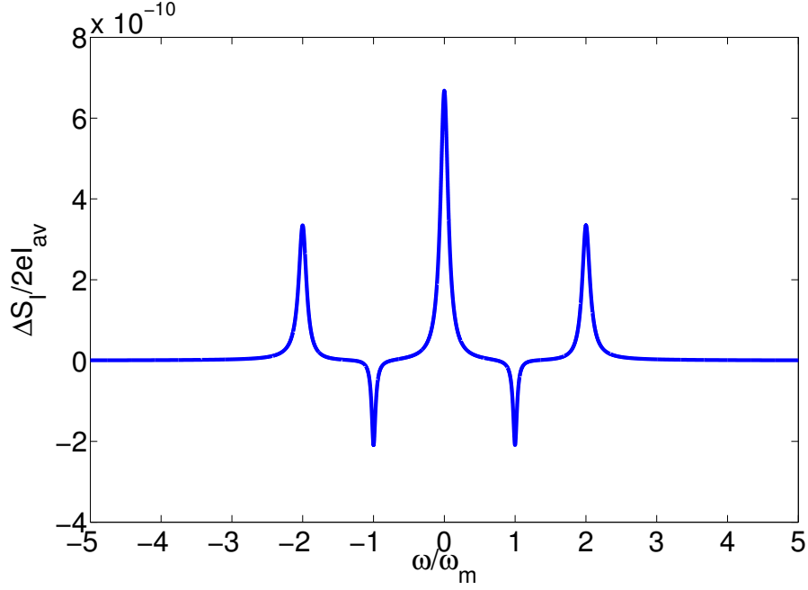
FIG. 12. (Color online) Dimensionless non-Poissonian current noise spectrum for the parameter values used for sample A in the experiment of Ref. [13]: t_0 = 0.71 , \tilde{V} = 1 \times 10^4 , \tilde{\lambda} = 7.2 \times 10^{-6} , \tilde{T} = 1.6 \times 10^3 , and \tilde{\Gamma}_0 = 3.3 \times 10^{-2} .
