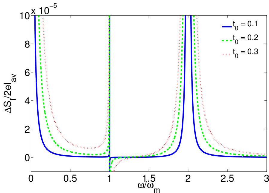
FIG. 2. (Color online) Dimensionless non-Poissonian current noise spectrum for t_0 = 0.1, 0.2 and 0.3 . The remaining parameters are \tilde{V} = 2 \times 10^4 , \tilde{\lambda} = 1 \times 10^{-3} , \tilde{\Gamma}_0 = 5 \times 10^{-6} , and \tilde{T} = 1 \times 10^4 .
