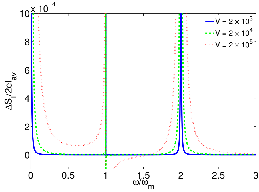
FIG. 3. (Color online) Dimensionless non-Poissonian current noise spectrum for \tilde{V} = 2 \times 10^3 , 2 \times 10^4 and 2 \times 10^5 . The remaining parameters are t_0 = 0.2 , \tilde{\lambda} = 1 \times 10^{-3} , \tilde{\Gamma}_0 = 5 \times 10^{-6} , and \tilde{T} = 1 \times 10^4 .
