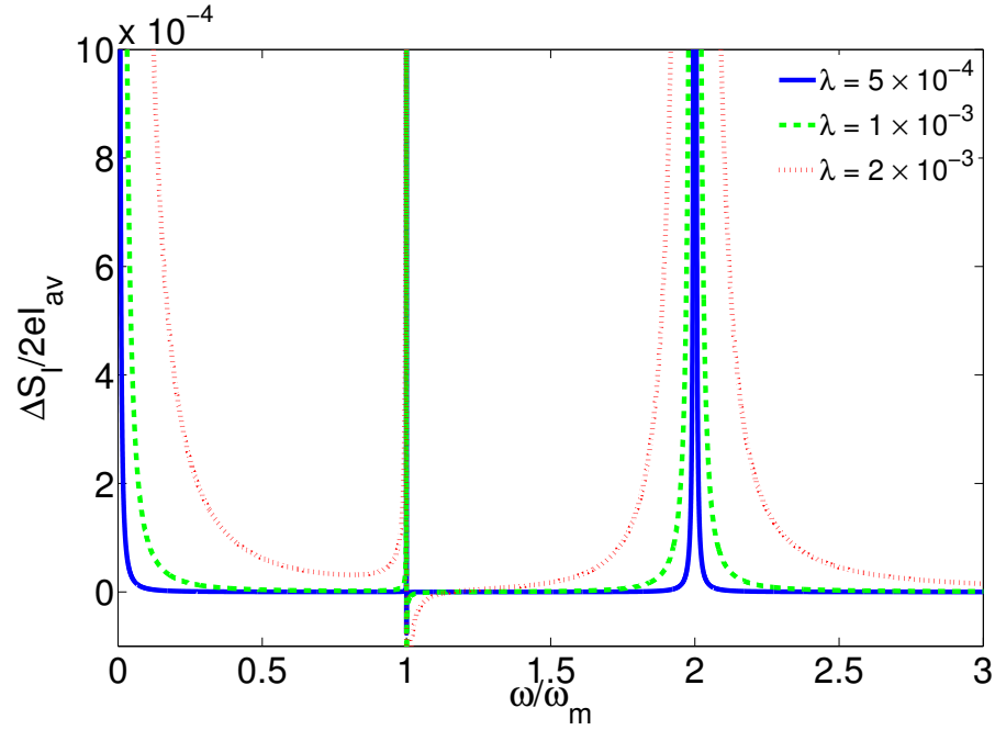
FIG. 4. (Color online) Dimensionless non-Poissonian current noise spectrum for \tilde{\lambda} = 5 \times 10^{-4} , 1 \times 10^{-3} and 2 \times 10^{-3} . The remaining parameters are t_0 = 0.2 , \tilde{V} = 2 \times 10^4 , \tilde{\Gamma}_0 = 5 \times 10^{-6} , and \tilde{T} = 1 \times 10^4 .
