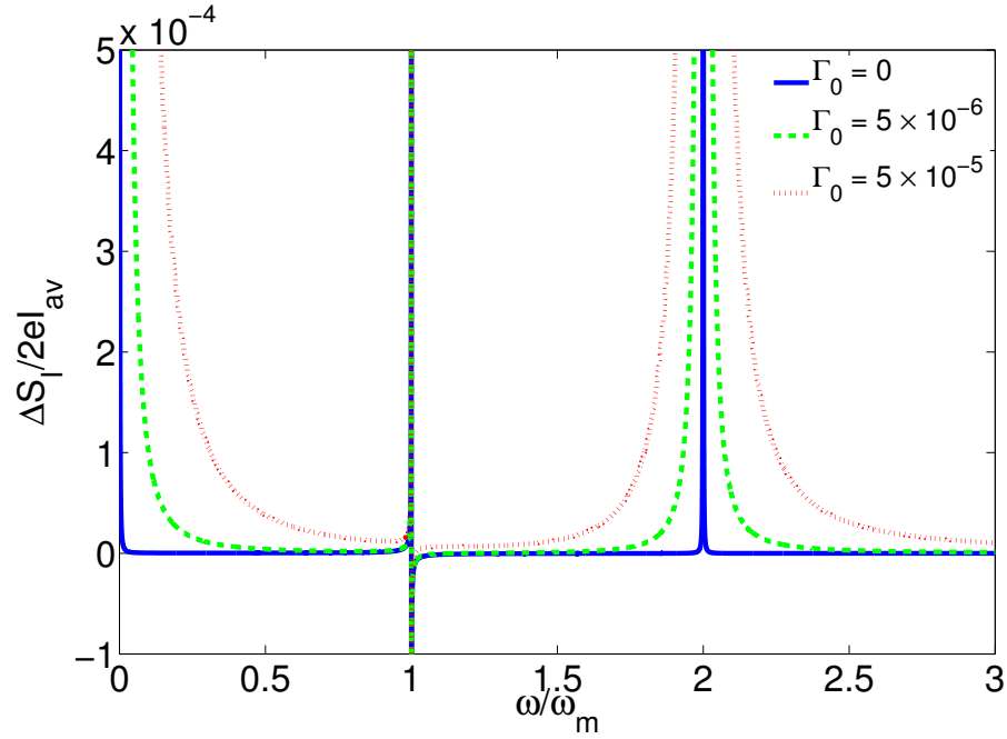
FIG. 6. (Color online) Dimensionless non-Poissonian current noise spectrum for \tilde{\Gamma}_0 = 0 , 5 \times 10^{-6} and 5 \times 10^{-5} . The remaining parameters are t_0 = 0.2 , \tilde{V} = 2 \times 10^4 , \tilde{\lambda} = 1 \times 10^{-3} , and \tilde{T} = 1 \times 10^4 .
