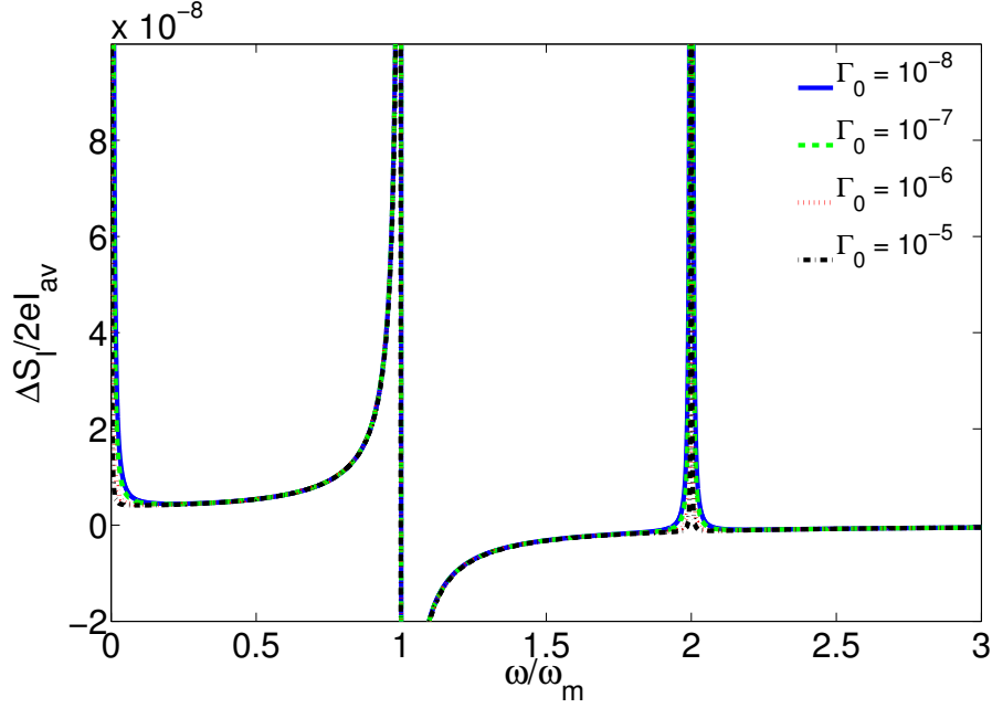
FIG. 11. (Color online) Dimensionless non-Poissonian current noise spectrum for \tilde{\Gamma}_0 = 10^{-8}, 10^{-7}, 10^{-6} and 10^{-5} . The remaining parameters are t_0 = 0.1 , \tilde{V} = 100 , \tilde{\lambda} = 0.01 , and \tilde{T} = 0.01 .
