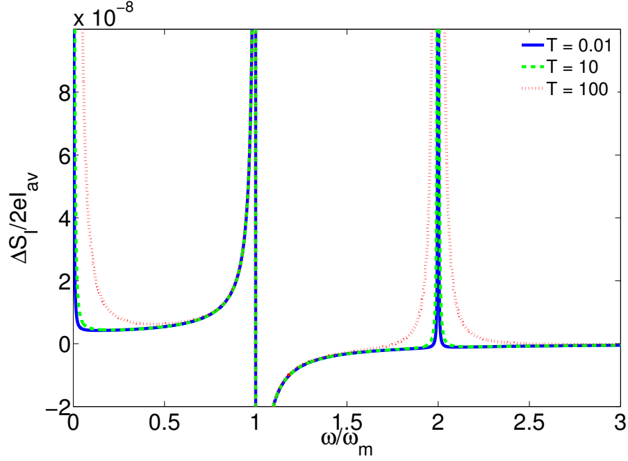
FIG. 10. (Color online) Dimensionless non-Poissonian current noise spectrum for \tilde{T} = 0.01, 10 and 100 . The remaining parameters are t_0 = 0.1 , \tilde{V} = 100 , \tilde{\lambda} = 0.01 , and \tilde{\Gamma}_0 = 10^{-6} .
