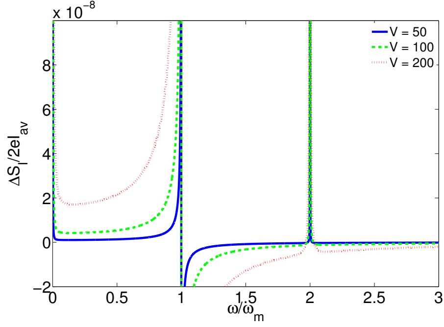
FIG. 8. (Color online) Dimensionless non-Poissonian current noise spectrum for \tilde{V} = 50, 100 and 200 . The remaining parameters are t_0 = 0.1 , \tilde{\lambda} = 0.01 , \tilde{T} = 0.01 and \tilde{\Gamma}_0 = 10^{-6} .
