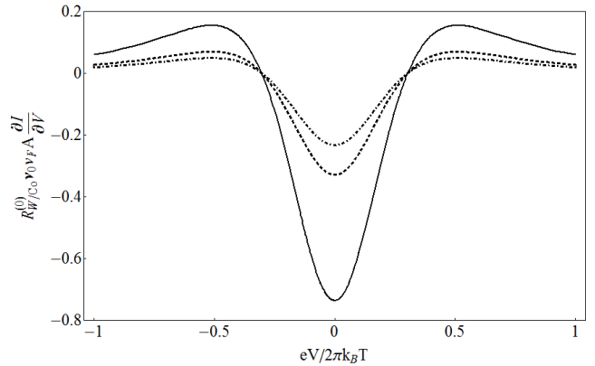
FIG. 5: Correction to the differential conductance from superconducting fluctuations as a function of dimensionless voltage eV/2\pi T (see (64)). The three curves correspond to different temperatures: t := (T - T_c)\tau = 0.01 for the solid line; t = 0.05 for the dashed line; and t = 0.1 for the dotted line.
