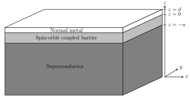
FIG. 3: The proximity tunnel junction considered. The ferromagnetic normal metal, the tunnel barrier with spin-orbit coupling and the superconductor occupy 0 \leq z \leq d , -a < z < 0 and z \leq -a , respectively.
