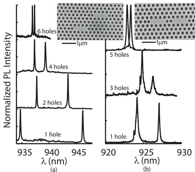
FIG. 2: Photoluminescence spectra of the coupled cavities for different hole spacings between two cavities: (a) the cavities are separated at an angle of 30^\circ (see the inset for a scanning electron micrograph (SEM)); (b) the cavities are laterally separated (see the inset for SEM). A decrease in the wavelength separation between two cavity modes is observed with increasing spatial separation between the cavities (i.e., with increasing number of holes inserted in between the two cavities). A much larger separation is observed in (a) when the cavities are coupled at an angle compared to the lateral coupling (b).
