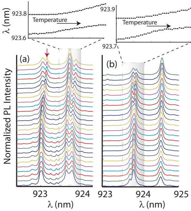
FIG. 3: (color online) Normalized PL intensity plotted when we tune the QD across the cavity resonance by temperature: (a) before nitrogen deposition (i.e., the QD is temperature tuned across the longer wavelength resonance), and (b) after nitrogen deposition (which red-shifts the cavity resonances and allows us to temperature tune the QD across the shorter wavelength resonance). Clear anti-crossings between the QD and the cavity are observed for both super-modes. In both cases, the temperature is increased from bottom to top (the plots are vertically offset for clarity). In the inset the resonances of the two anti-crossing peaks (as extracted from curve-fitting) are plotted. Clear anti-crossing is observed in both cases.
