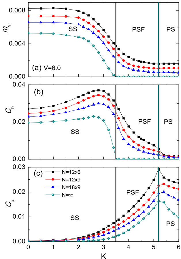
FIG. 4: (color online) (a) The density structure factor order parameter m_s , (b) atomic condensate density C_b at momentum k_1 = (4\pi/3, 0) , and (c) pair condensate density C_p at momentum k_0 = (0, 0) , as functions of K at V = 6.0 and filling \rho = 1/6 , respectively, with system size N = 12 \times 6 , 12 \times 9 , 18 \times 9 , and the corresponding extrapolations in the thermodynamic limit.
