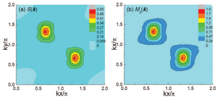
FIG. 3: (Color online) Examples of the contour plot of the boson density structure factor S(\mathbf{k}) and boson momentum distribution M_b(\mathbf{k}) as a function of \mathbf{k} , at V = 6.0 and K = 1.0 for system N = 12 \times 6 .
