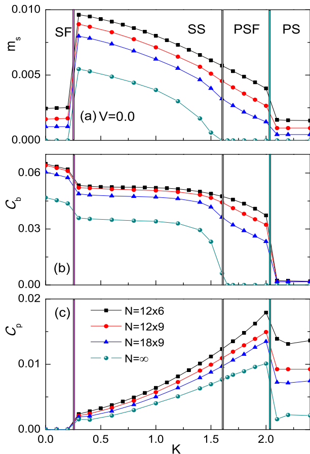
FIG. 6: (color online) (a) The density structure factor order parameter m_s , (b) atomic condensate density C_b at momentum k_1 = (4\pi/3, 0) , and (c) the pair condensate density C_p at momentum k_0 = (0, 0) , as functions of K at V = 0.0 and filling \rho = 1/6 , respectively, with system size N = 12 \times 6 , 12 \times 9 and 18 \times 9 , as well as the corresponding extrapolations in the thermodynamic limit.
