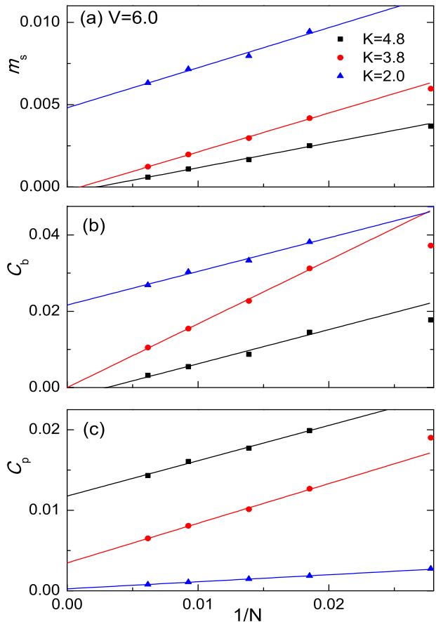
FIG. 5: (color online) Examples of finite-size scaling of (a) the density structure factor order parameter m_s and (b) atomic condensate density C_b at momentum k_1 = (4\pi/3, 0) , as well as (c) the pair condensate density C_p at momentum k_0 = (0, 0) , for different K at V = 6.0 and filling \rho = 1/6 , with system size up to 18 \times 9 .
