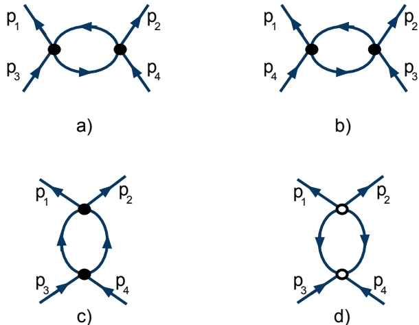
FIG. 1: One-loop contributions to the four-point function \Gamma^4(p_1, p_2; p_3, p_4) = \langle \Phi(p_1)\Phi(p_2)\Phi^*(p_3)\Phi^*(p_4) \rangle determining the flow of u in the theory (42). A solid dot denotes a u -vertex and a hollow dot - a v -vertex.
