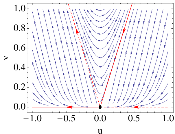
FIG. 3: RG flow of coupling constants u and v in the theory (42). Solid and dashed red lines mark separatrices and attractor lines, respectively.
