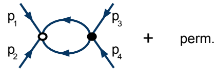
FIG. 2: One-loop contributions to the four-point function \bar{\Gamma}^4(p_1, p_2, p_3, p_4) = \langle \Phi^*(p_1)\Phi^*(p_2)\Phi^*(p_3)\Phi^*(p_4) \rangle determining the flow of v in the theory (42). There are a total of 6 distinct diagrams obtained by permuting the external momenta p_1, p_2, p_3, p_4 .
