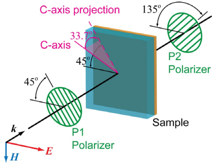
Figure 5(Color online): Measurement setup for chiral metamaterials. One THz wire-grid polarizer was installed ahead and one behind the sample, each oriented either 45^\circ or 135^\circ with respect to the horizontal. The THz electromagnetic wave was polarized horizontally and was incident from the substrate (sapphire) side (blue region (light gray)) of the samples.
