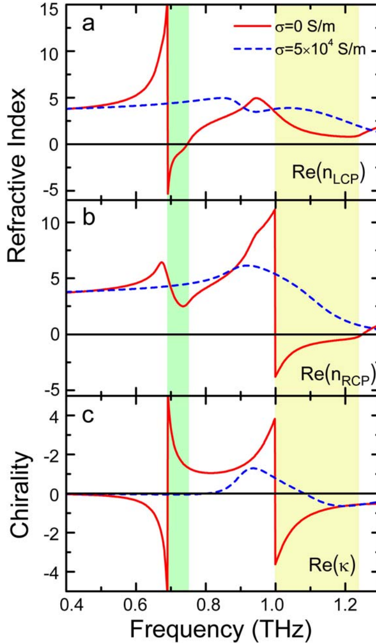
Figure 3(Color online): Refractive index for LCP (a) and RCP (b) obtained from numerical simulations with silicon island conductivity \sigma = 0 (red solid) and 5 \times 10^4 S/m (blue dash), which corresponds to laser fluence of 0 and 40 \mu\text{J}/\text{mm}^2 in experiments. Green and yellow shaded regions highlight negative values of refractive index, n_{LCP} and n_{RCP} , respectively. (c) Real part of the chirality parameter \kappa .
