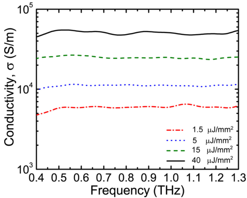
Figure 6(Color online): Measured conductivity of the silicon layer on the sapphire substrate for laser fluences of 1.5, 5, 15 and 40 \mu\text{J}/\text{mm}^2 .
