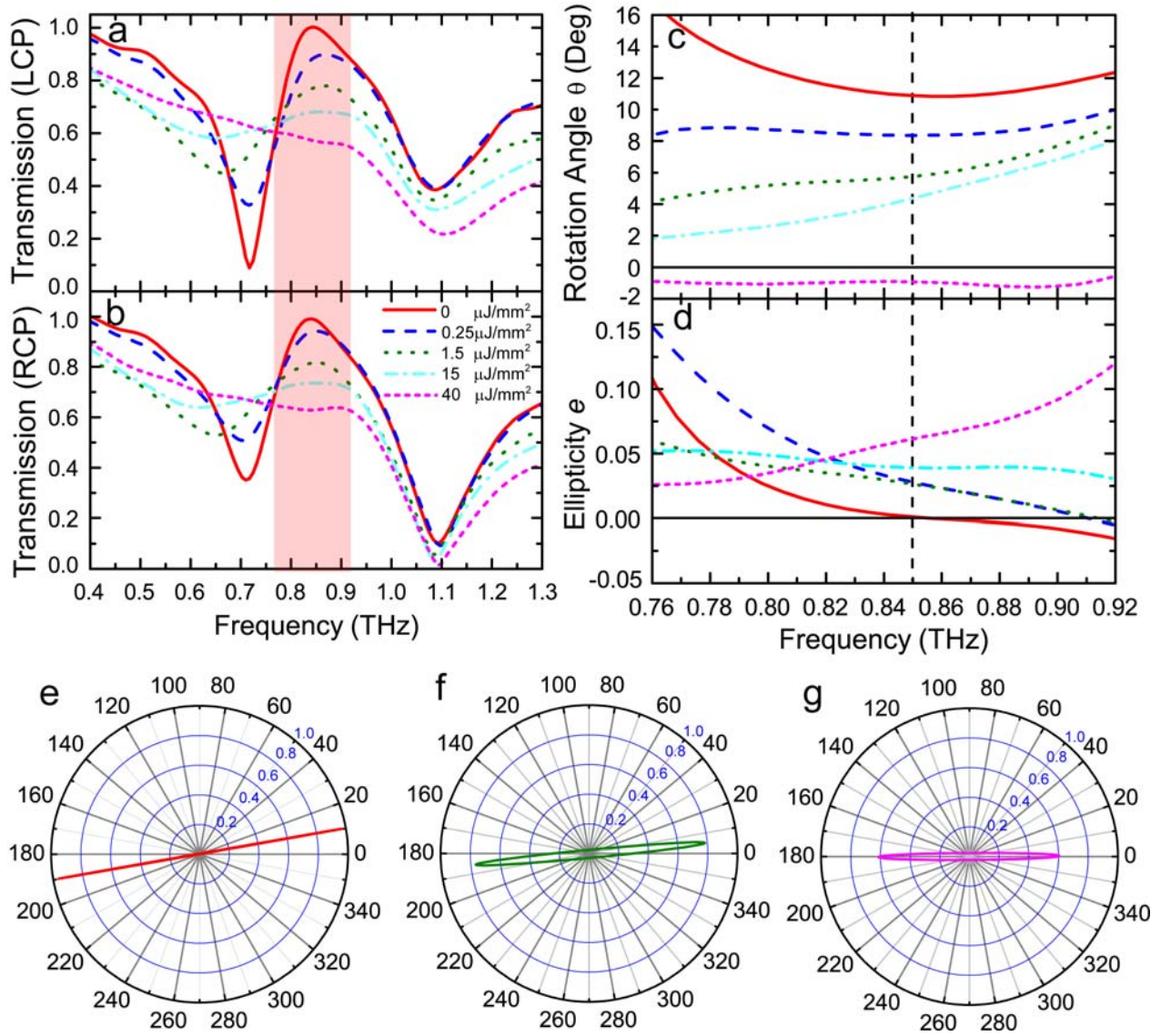
Figure 2(Color online): Measured transmission coefficients of left (a) and right (b) handed circular polarizations (LCP and RCP) under normal incidence at different fluence levels of near-infrared photoexcitation. The shaded region indicates the operation frequency range (off-resonance) with simultaneously high transmission and significant chirality. With linearly polarized incident THz radiation, the rotation angle (c) and ellipticity (d) of the transmission are calculated from the experimental data in (a) and (b). At 0.85 THz, the polar plots show the polarization state of the transmitted wave with photoexcitation fluences of 0 (e), 1.5 (f) and 40 (g) \mu\text{J}/\text{mm}^2 .
