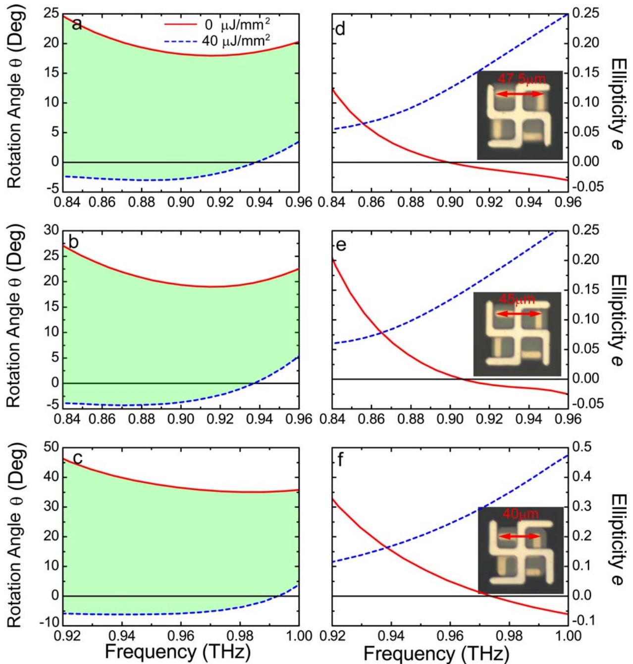
Figure 4(Color online): Measured rotation angle (a,b,c) and ellipticity (d,e,f) for dynamic chiral metamaterials with bottom-layer resonator dimensions of 47.5 \mu\text{m} , 45 \mu\text{m} and 40 \mu\text{m} , respectively, with the unit cell microscopic images shown in the insets. Size of top layer resonator is 60 \mu\text{m} for all three designs. Red (solid) and blue (dash) curves show measured rotation angle and ellipticity with the laser fluences of 0 and 40 \mu\text{J}/\text{mm}^2 , respectively. Green shaded regions (a,b,c) show increased tuning range as bottom-layer resonator size decreases.
