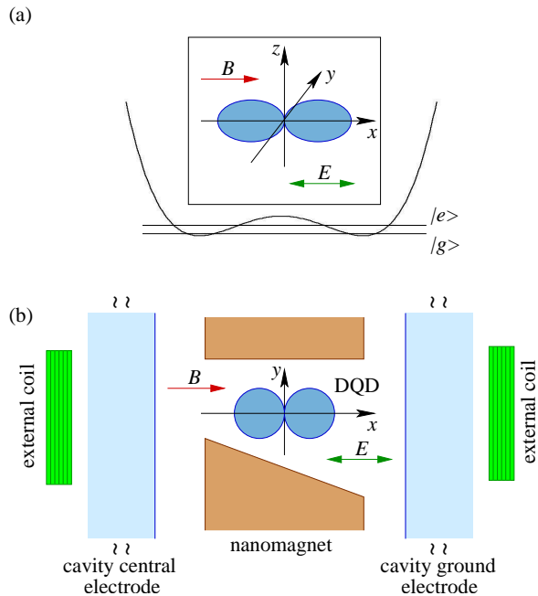
FIG. 1: (Color online) Schematics of the two-dimensional double dot in a cavity. Panel (a) shows that both the cavity electric field and the external magnetic field are along the interdot axis ( x -axis). Panel (b) shows the top view of the combined DQD-nanomagnet-cavity system for the case of a DQD in an inhomogeneous magnetic field. External coils are used to produce the uniform magnetic field, while close-by nanomagnets provide the transverse inhomogeneous field.
