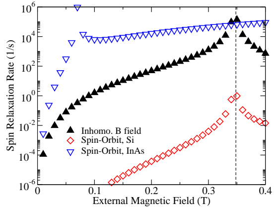
FIG. 2: (Color online) Single-spin relaxation rate in a Si or InAs DQD as a function of the applied field. Here the tunnel splitting of the double dot orbital state is \epsilon_0 = 40 \mu\text{eV} (the vertical line represents the resonant condition when 2\epsilon_Z = \epsilon_0 for Si, with a corresponding magnetic field of 0.345 T), and the interdot distance is 100 nm for Si and 50 nm for InAs. The black filled triangles represent the spin relaxation due to spin mixing from the inhomogeneous magnetic field along the interdot ( x ) direction, while the red unfilled diamond (for InAs) and blue unfilled triangles (for Si) are due to Rashba spin-orbit coupling. The spin relaxation rate for InAs peaked at a different magnetic field because of the very different g -factor (we used g = 10 here).
