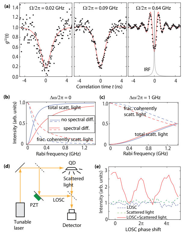
FIG. 4: (Color online) (a) Photon statistics of scattered light for three different Rabi frequencies. When \Omega > \kappa , Rabi oscillations appear. (b) Plot of the total scattered light intensity (solid red trace) and the fraction of coherently scattered light intensity (dashed red trace), using the same parameters as those used in Fig. 3. For comparison the same are plotted in blue when not including spectral diffusion. (c) Same as in (b) but with a laser detuned by \Delta\omega/2\pi = 1 GHz. (d) Measurement of mutual phase coherence between the coherently scattered light and a local oscillator (LOSC) by interferometry. (e) Intensity of light at the output of the beam splitter in (d) as a function of LOSC phase.
