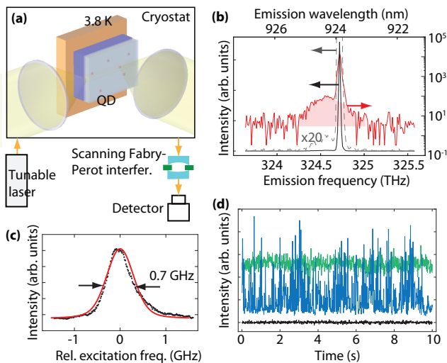
FIG. 1: (Color online) (a) Schematic of experimental setup. (b) QD emission spectrum, recorded with a grating spectrometer under resonant laser excitation as is (black solid trace), 20 \times magnified (dashed gray trace) and on a logarithmic scale (solid red trace) to visualize the phonon broadband. (c) QD excitation spectrum. (d) Spectrally integrated intensity of scattered light as a function of time showing flickering (dark blue trace) that is inhibited when an additional weak auxiliary laser is added (light green trace). The black trace was recorded with the auxiliary laser only.
