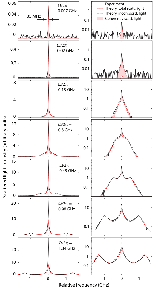
FIG. 3: (Color online) Power spectrum of light scattered by the QD at exact resonance ( \Delta\omega = 0 ) represented on a linear (left) and logarithmic (right) ordinate scale, for a range of Rabi frequencies. Each spectrum was recorded in 60 s. The theoretical curve (red dashed line) was obtained by numerical evaluation of Eq. (2). The light red shaded area corresponds to coherently scattered light which dominates whenever \Omega \lesssim \kappa . If pure dephasing had a significant role in the scattering process, a broader feature would always be visible, even when \Omega \ll \kappa .
