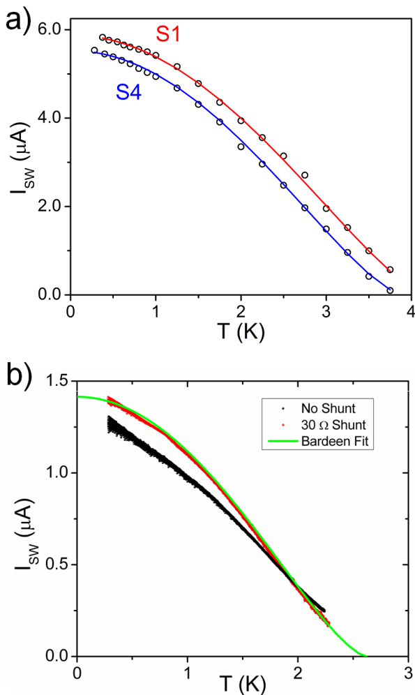
FIG. 5: (a) Mean I_{sw} vs. T for samples S1 and S4 shunted with 5\ \Omega and 10\ \Omega respectively. The solid lines are fits to the Bardeen’s prediction (Eq.3.4) for the temperature dependence of the depairing current, I_c . The fitting parameters used are: I_{c0} = 5.88, 5.53\ \mu\text{A} and T_c = 4.2, 3.9\ \text{K} for samples S1 and S4, respectively. (b) Distribution of I_{sw} vs. T for sample S5 unshunted (red) and shunted with 30\ \Omega (black). Each curve contains approximately 20,000 points. The corresponding fit to the Bardeen prediction (green) is presented for the shunted wire. Here I_{c0} = 1.415\ \mu\text{A} and T_c = 2.62\ \text{K} .
