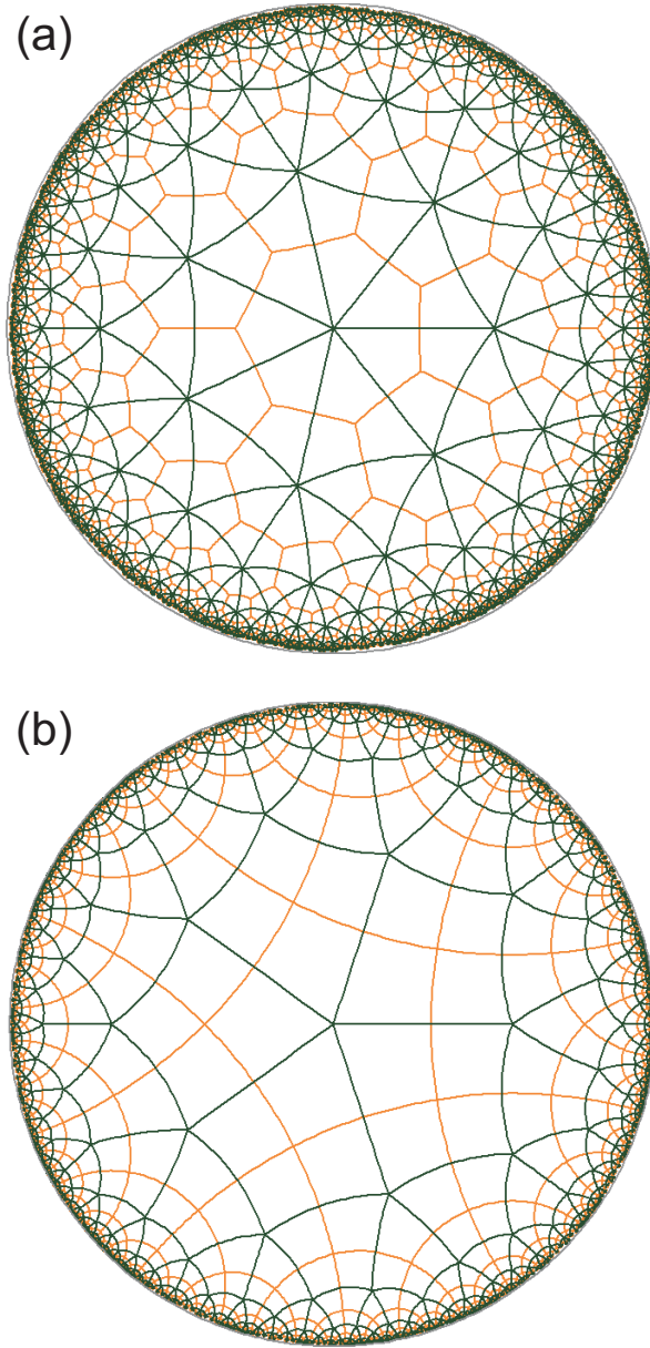
FIG. 1: (Color online) Hyperbolic tessellations in a Poincaré disk. The Schläfli symbols \{p, q\} describe tessellations where q regular p -gons meet at each vertex: \{3, 7\} (a) and \{4, 5\} (b) (shown by dark green/black lines). The corresponding dual tessellations \{7, 3\} (a) and \{5, 4\} (b) are shown by orange (grey in black and white) lines.
