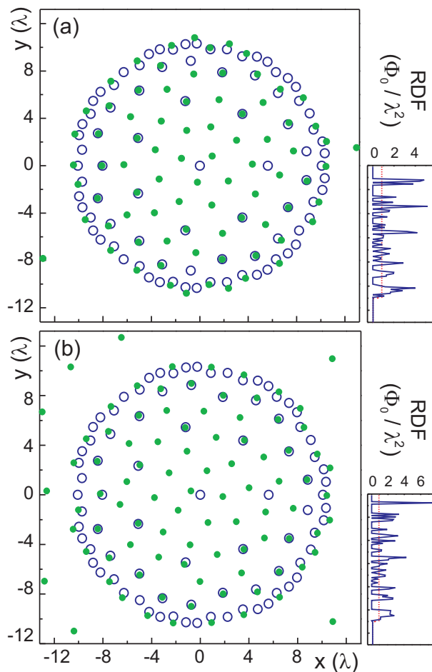
FIG. 4: (Color online) Accumulation of the magnetic flux in a HT APS and its expulsion: vortex patterns for N_v = 81 (a), and 93 (b). The right-hand side panels show the corresponding RDF for the magnetic flux inside ( r/\lambda \lesssim 11 ) and outside ( r/\lambda \gtrsim 11 ) the HT [solid dark blue (black) line] and the average magnetic flux inside the HT [dashed red (grey) line].
