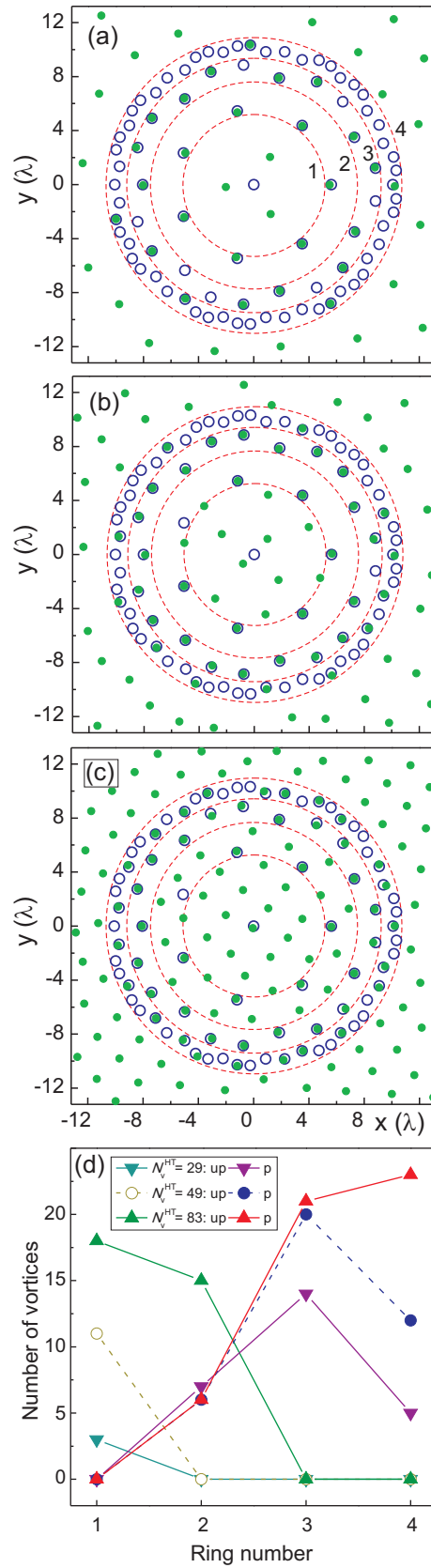
FIG. 2: (Color online) Vortex configurations in a \{3, 7\} hyperbolic tessellation (HT) APS for varying number of vortices per simulation cell (inside the HT): N_v = 49 ( N_v^{\text{HT}} = 29 ) (a), N_v = 81 ( N_v^{\text{HT}} = 49 ) (b), and N_v = 144 ( N_v^{\text{HT}} = 83 ) (c). Pinning sites are shown by dark blue (black) open circles, vortices by green (grey) dots. Red (grey) dashed lines show the boundaries of concentric rings [numbered 1 to 4 (a)] of the same area containing 1, 7, 21, and 56 pins. (d) Number of pinned (p) and unpinned (up) vortices in the rings, corresponding to N_v^{\text{HT}} in (a) to (c), shown by symbols (lines connecting the symbols are guides for eye).
