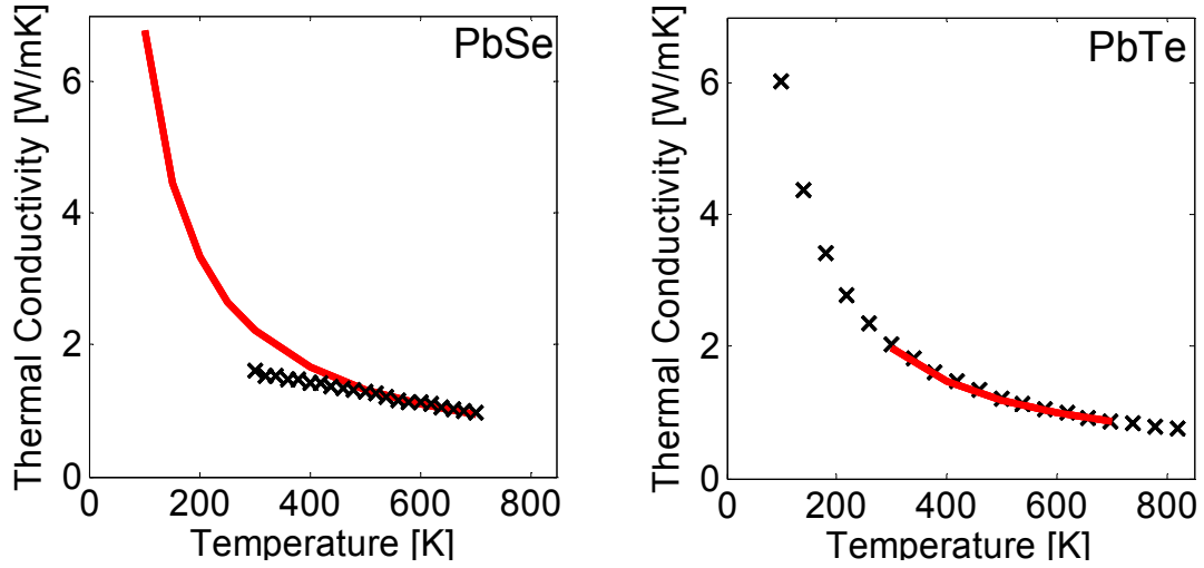
Fig. 2 Temperature dependent lattice thermal conductivity of PbSe and PbTe, red lines: calculated results; black crosses: experimental data [29, 30].
