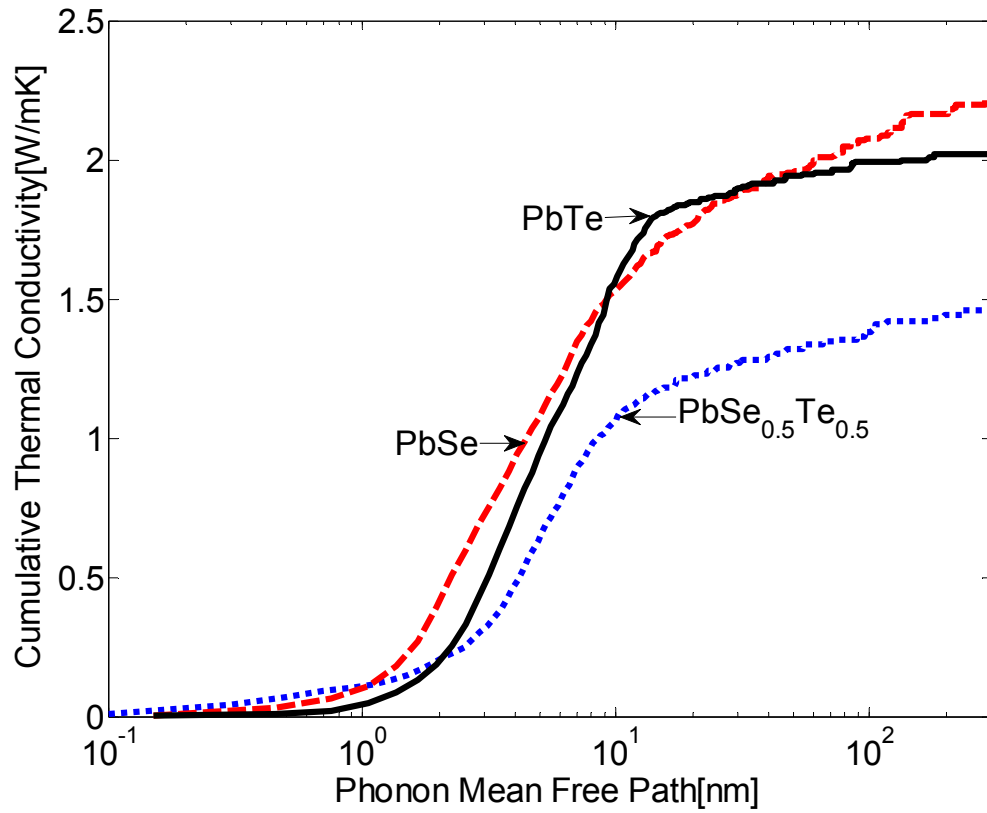
Fig. 7 Cumulative thermal conductivity with respect to phonon mean free path at 300 K for PbSe (red dashed line), PbTe (black solid line) and \text{PbTe}_{0.5}\text{Se}_{0.5} (blue dotted line)
