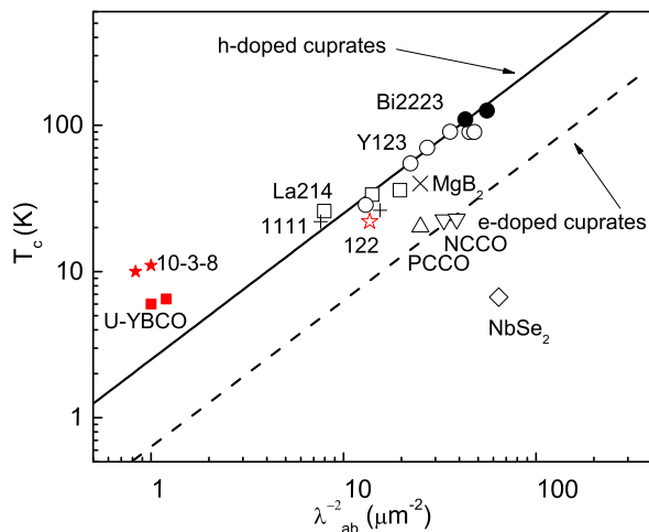
FIG. 3: (Color online) Uemura plot for high T_c cuprates. The data for the cuprates and points for the 1111 system are taken from Ref. 25. The data for \text{MgB}_2 and \text{NbSe}_2 are taken from Ref. 26 and Ref. 27, respectively. The red filled squares show highly underdoped YBCO superconductors taken from Ref. 28. The red filled stars represent the data for 10-3-8 obtained in this work.
