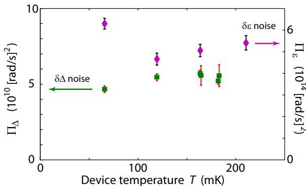
FIG. 4: (color online) Temperature dependencies of the total noise powers \Pi_\lambda(T) = (2\pi)^2 \kappa_\lambda^2 \int_{F_\lambda} df S_\lambda(f; T) in the frequency intervals F_\varepsilon = 0.02 - 50 Hz and F_\Delta = 0.02 - 2 Hz, cf. Fig. 2(b). It is possible to measure the \delta\varepsilon noise up to somewhat higher temperatures and frequencies than the \delta\Delta noise. Note that the \Pi_\lambda values depend on the integration limits although the choice of F_\lambda does not make any significant difference in the trends. (The double data points for the 165- and 180-mK \delta\Delta noise were measured with different pulse spacings \tau_0 .) We estimated the device temperature from switching-current measurements on the SQUID, which suggest saturation at dilution-refrigerator temperatures below about 65 mK. The error bars are derived only from the fit error of the read-out visibility a(\tau_0, T) , included in the p_{\text{sw-to-}\delta\lambda} conversion factor \eta_\lambda(\tau_0, T) , see Fig. 1(f).
