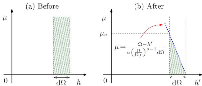
Figure 2: (Color online) Schematic of the possible transverse-field decimations in the h vs. \mu plane. (a) Before the integration of the fast oscillators, the hatched area represents all the potential fields to be decimated. (b) After integrating out the oscillators, some of these fields have been shifted below \Omega - d\Omega and are not eligible to be decimated anymore, only those in the triangular shaded area still are. The dashed line h = \Omega maps into the dotted line \mu = (\Omega - h')/(\alpha(\Omega/\Omega_I)^{s-1}d\Omega) after the adiabatic-renormalization step (11).
