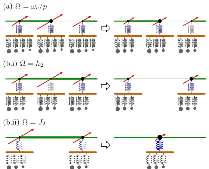
Figure 1: (Color online) Decimation scheme. The magnitude of the transverse fields, interactions and magnetic moments are depicted by the length of the arrows, the thickness of the lines and the size of the dots, respectively. The bosonic bath are depicted by the array of springs and oscillators in which lighter (small) oscillators are faster. Finally, the magnitude of the coupling to the bath (or the local dissipation strength) is depicted by the thickness of the spring connecting the spin to the bath. (a) global adiabatic renormalization of the fast oscillators, (b.i) decimation of a strong local transverse field, and (b.ii) decimation of a strong local interaction.
