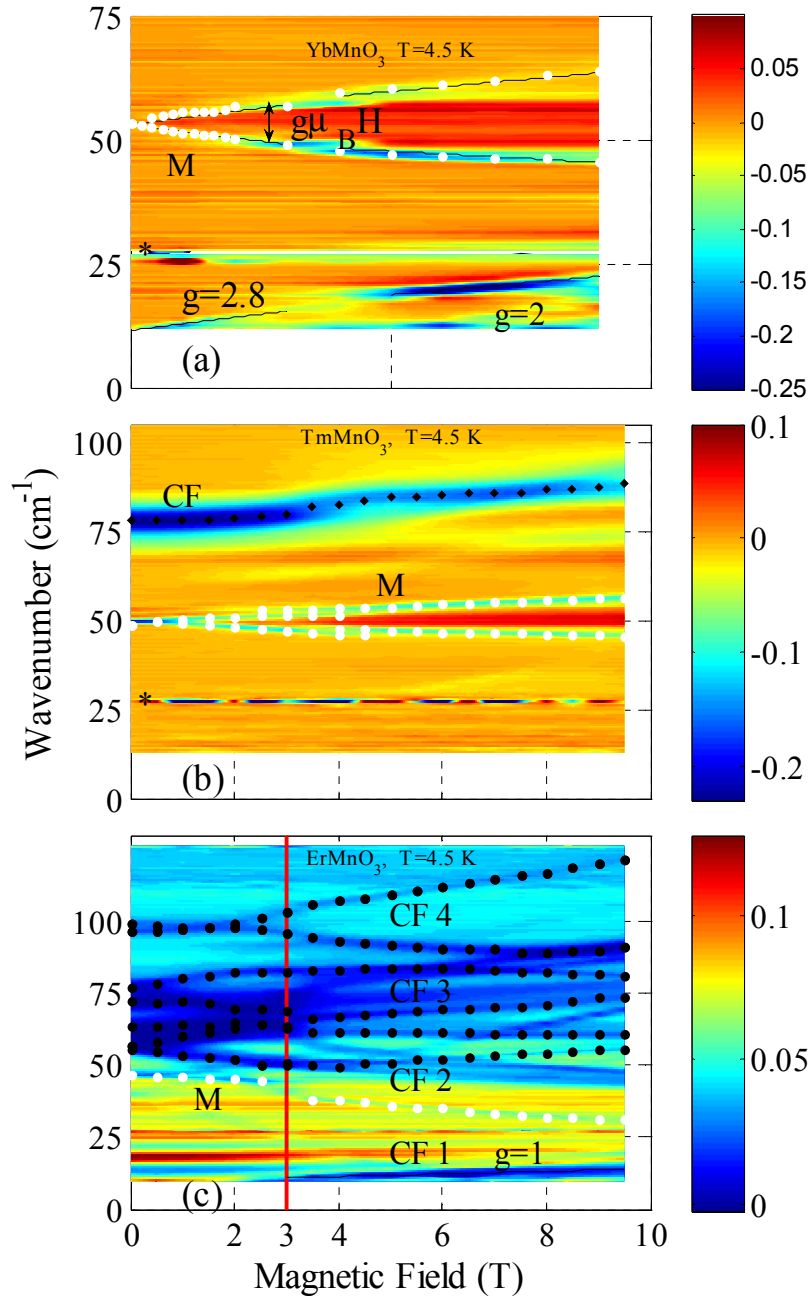
FIG. 8 (color online) Normalized transmission maps vs. magnetic field and light frequency for \text{YbMnO}_3 in (a), \text{TmMnO}_3 in (b), and \text{ErMnO}_3 in (c) measured at T = 4.5 K. The blue (dark) color corresponds to stronger absorption and red (light) color indicates high transmission. The transmission intensity scale is shown with the vertical bars. The black dots represent the fit results for the CF transitions. The magnons M are shown with white circles. Note the changes of the magnon g -factor for \text{YbMnO}_3 at the critical field H_C \approx 4 T in (a). The critical field for \text{ErMnO}_3 , H_C = 2.8 T, is marked with the vertical red line. Noise in (a) and (b) maps at \sim 27 \text{ cm}^{-1} , which is marked with (*) is an artifact of the experimental setup.
