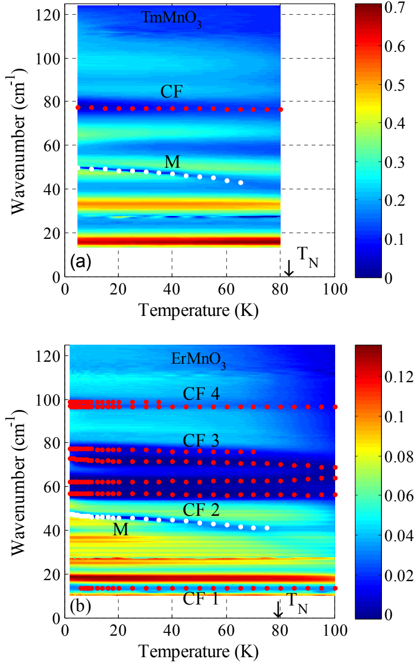
FIG. 3 (color online) Transmission maps vs. temperature and light frequency for \text{TmMnO}_3 (a) and \text{ErMnO}_3 (b). The blue (dark) color corresponds to stronger absorption and red (light) color indicates high transmission. The transmission intensity scale is shown with the vertical bars. Black arrows indicate the AFM transition temperatures T_N . Frequencies of the CF transitions are shown with red dots and the magnon frequencies are shown with white dots. Noise in the map (a) at \sim 27 \text{ cm}^{-1} is an artifact of the experimental setup.
