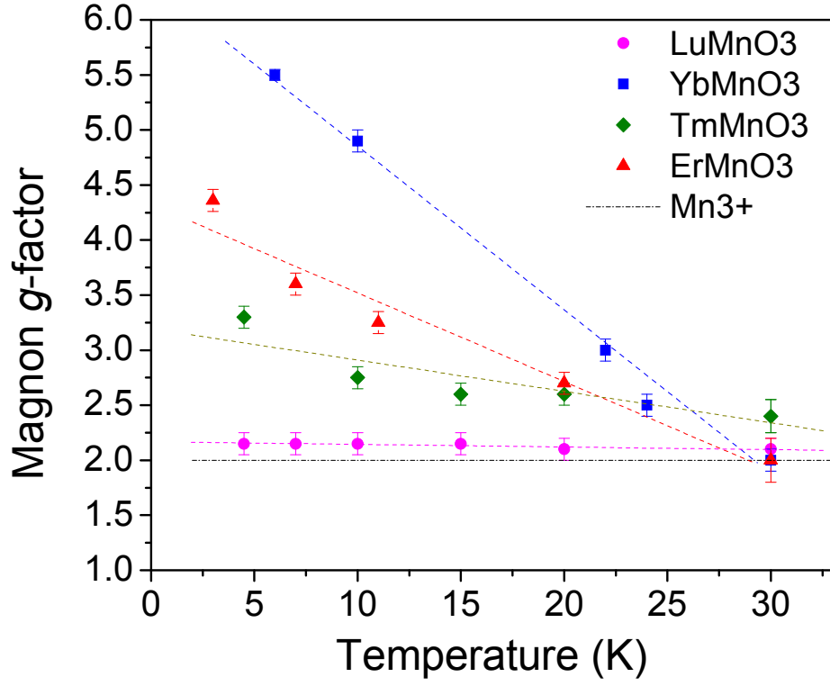
FIG. 6. (color online) Temperature dependence of the magnon g -factor for REMnO_3 ( RE=Lu, Yb, Tm , and Er ). Dashed lines guide the eye. The horizontal line corresponds to the theoretical expectation for g -factor of Mn^{3+} : g_{Mn}=2 . At higher temperatures above T \approx 32 \pm 5 K, the magnon g -factors approach g_{Mn}=2 in all REMnO_3 .
