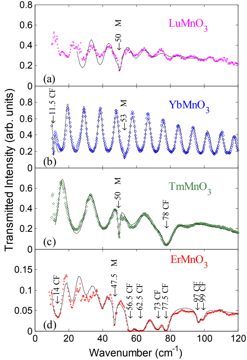
FIG. 1 (color online) Transmission spectra of REMnO_3 samples measured for the light propagation along the c -axis at T \approx 4.5 K and at zero magnetic field. The magnon absorption lines are marked with M. The crystal field transitions are marked with CF. Black solid curves represent the fit results using the multi-oscillator dielectric model [see Eq.(1)]. The magnon and CF frequencies are rounded up to 0.5 \text{ cm}^{-1} .
