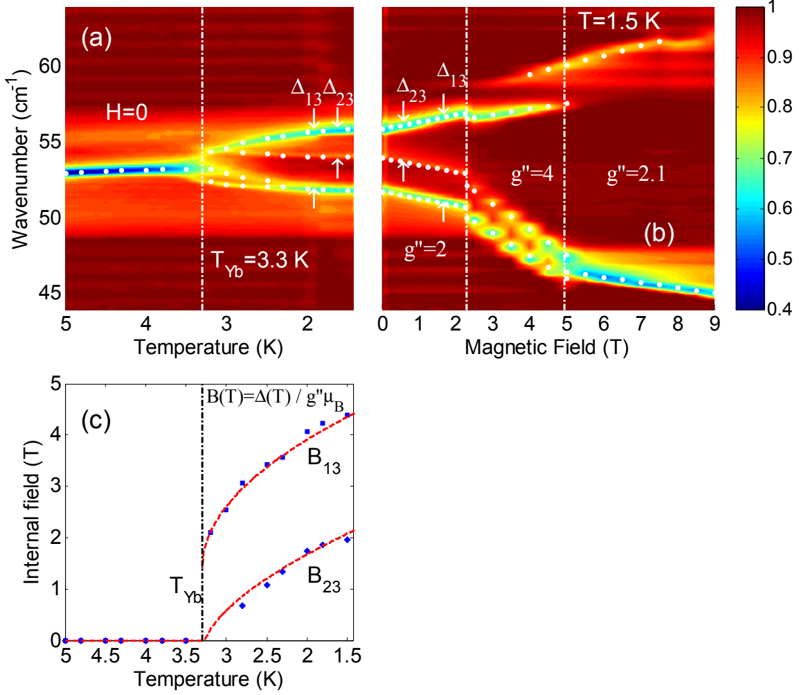
FIG. 7. (color online) (a) Temperature dependence of the transmission intensity in YbMnO 3 measured at zero magnetic field. The magnon lines are marked with white dots. Below T_{Yb} = 3.3 K the major splitting of the magnon is marked with \Delta_{13} . Two additional weak absorption lines can be seen with a smaller splitting \Delta_{23} between the top two modes. (b) Magnetic field dependence of the transmission intensity measured at T = 1.45 K, which corresponds to the right edge of the map in (a). The vertical frequency scale and the intensity scale are the same for the maps in (a) and (b). Below H = 2.3 T, the major magnon doublet splits in external field as \Delta_{13}(T, H) = g'' \mu_B [B(T) + H] with g'' = 2 . Between H = 2.3 T and H = 5 T, the magnon g -factor is g'' = 4 . g'' = 2.1 for H > 5 T. (c) Temperature dependence of the two internal fields B_{13} and B_{23} , which correspond to \Delta_{13} and \Delta_{23} splittings in (a) calculated as B(T) = \Delta(T) / (g'' \mu_B) with g'' = 2 . Note that the reversed scale for temperature in (c) matches that in (a).
