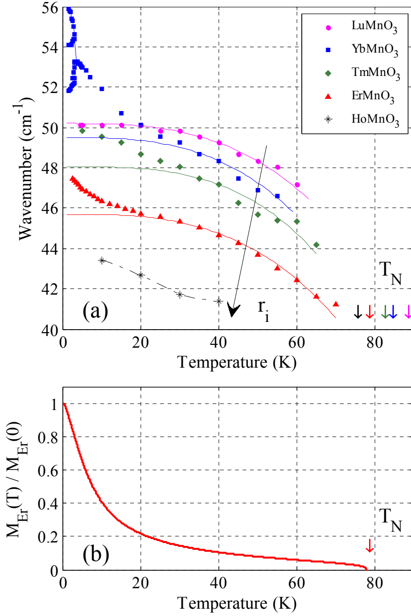
FIG. 2 (color online) (a) Temperature dependence of the magnon frequency for five REMnO_3 samples at zero magnetic field. Black stars correspond to HoMnO 3 (courtesy of D. Talbayev). At low temperatures, a single magnon in YbMnO 3 splits into several distinct absorption lines due to ordering of Yb spins at T_{yb} = 3.3 K. Solid curves for Lu, Yb, Tm, and Er samples show the fit results using \Omega_M(0) - \Omega_M(T) \sim T^3 . Dashed curve for HoMnO 3 guide the eye. The AFM transition temperatures T_N for Mn^{3+} are shown with arrows. The arrow labeled r_i indicates the increase of the RE ionic radius and the corresponding decrease of both, magnon frequency and T_N . (b) Calculation for the relative change of paramagnetic magnetization of Er^{3+} .
