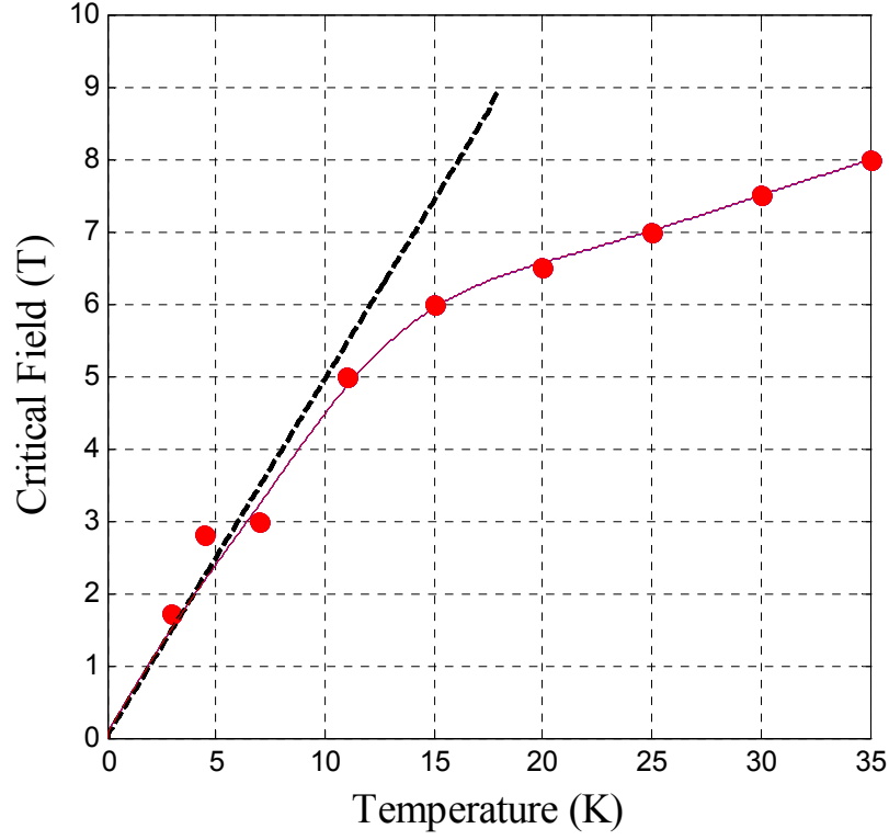
FIG. 9 (color online) Temperature dependence of the critical external magnetic field H_C in \text{ErMnO}_3 . Experimental points were determined from the 2D transmission intensity maps measured at different temperatures [similar to that is shown in Figure 8(c)]. Straight dotted line corresponds to g_{Er}\mu_B H_C = k_B T calculated with g_{Er} = 3 . Red curve guides the eye.
