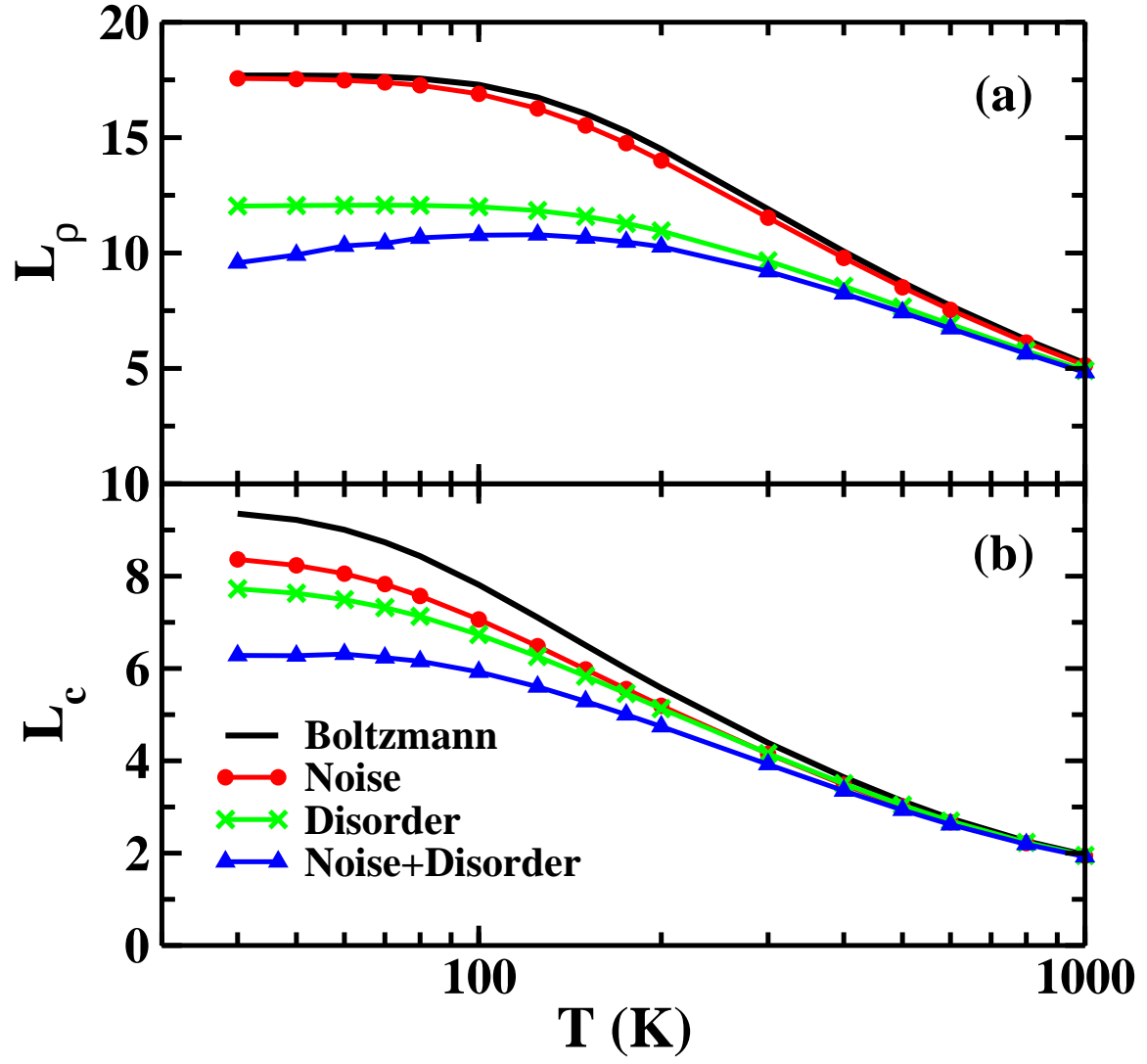
FIG. 8: (color online) The coherence lengths, L_\rho (a), and L_c (b), calculated for LH2 as a function of temperature. The solid (black) line is obtained from the Boltzmann populations without noise or disorder. The (red) line with dots is obtained from calculations with noise only using the spectral density of Eq. 19, the (green) line with crosses is obtained from calculations with static disorder only with a width of 200 \text{ cm}^{-1} , and the (blue) line with triangles is from calculations with both noise and disorder.
