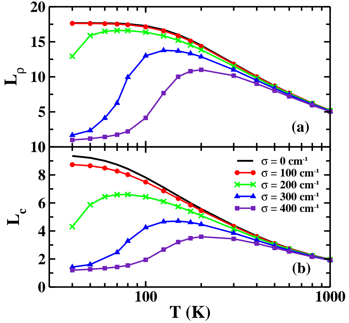
FIG. 10: (color online) The coherence lengths L_\rho (a), and L_c (b), calculated for LH2 as a function of temperature for increasing strength of the annealed disorder. The solid (black) line is obtained from the Boltzmann populations without any disorder. The widths of the annealed disorder distribution of 100, 200, 300, and 400 \text{cm}^{-1} are indicated by the (red) line with dots, (green) line with crosses, (blue) line with triangles, and (purple) line with squares, respectively.
