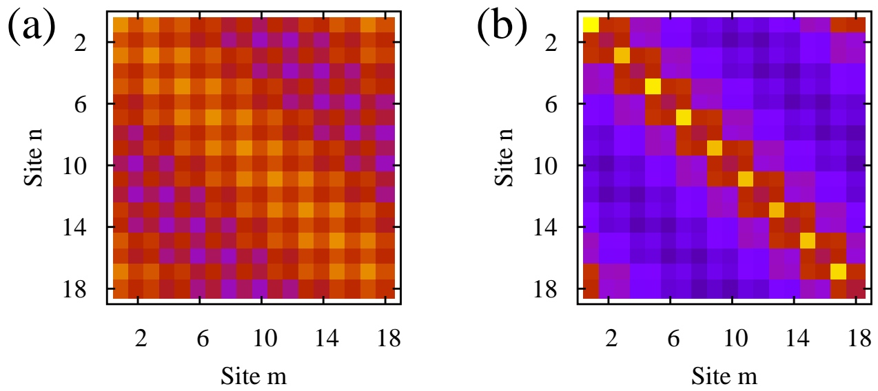
FIG. 4: (color online) The absolute value of the density matrix elements |\rho_{nm}| for LH2 at a temperature of 100 K. The left is the Boltzmann distribution and the right is the exact reduced density matrix calculated at a reorganization energy of 600 \text{ cm}^{-1} .
