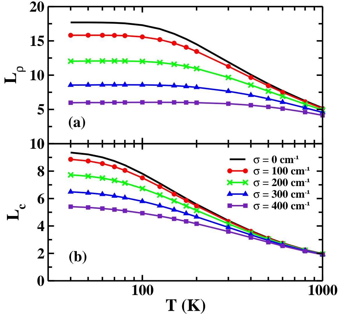
FIG. 7: (color online) The coherence lengths, L_\rho (a), and, L_c (b), calculated for LH2 as a function of temperature for increasing static disorder. The solid (black) line is obtained from the Boltzmann populations without any static disorder. The widths of the static disorder distribution of 100, 200, 300, and 400 \text{cm}^{-1} are indicated by the (red) line with dots, (green) line with crosses, (blue) line with triangles, and (purple) line with squares, respectively. Note the increasing persistence of the plateau with increasing disorder.
