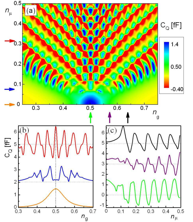
FIG. 7: (Color online) LZS interferometry probed via a quantum capacitance. (a) The quantum capacitance C_Q of the qubit versus the energy bias ( n_g ) and the driving amplitude ( n_\mu ). Arrows show the values of n_\mu and n_g at which the graphs (b) and (c) are plotted as functions of n_g and n_\mu , respectively. The upper curves were shifted for clarity.
