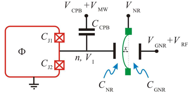
FIG. 2: (Color online) Schematic diagram of a split-junction charge qubit coupled to a nanomechanical resonator. The charge qubit (shown in red) is biased by the magnetic flux \Phi and the dc+ \mu w voltage V_{\text{CPB}} + V_{\text{MW}} , to which it is coupled through the capacitance C_{\text{CPB}} . The qubit is coupled to the NR (shown in green) through the capacitance C_{\text{NR}} . The NR is biased by a large dc voltage V_{\text{NR}} ; its state is controlled and measured by applying the dc and rf voltages between the gate and the NR, V_{\text{GNR}} and V_{\text{RF}} , through the capacitance C_{\text{GNR}} . The NR's motion is described by the displacement at the midpoint x . Capacitances form the island (Cooper-pair box) with the total capacitance C_{\Sigma} , voltage V_I and charge -2en .
