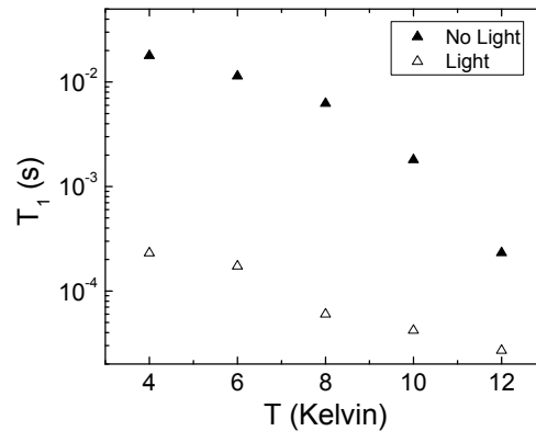
FIG. 4: The spin lifetime, T_1^e , of phosphorus donor electrons measured with an inversion recovery sequence at a resonance frequency of 240GHz with conventional pulsed electron spin resonance. The measurements are performed both in the dark (closed data points), and whilst shining light onto the sample (open data points).
