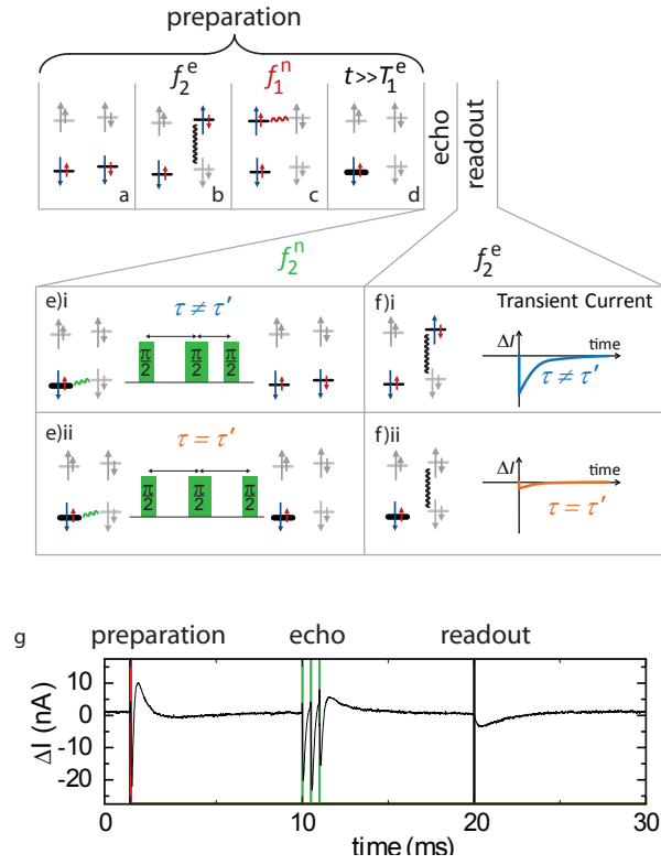
FIG. 2: Pulse sequence for observing nuclear spin echoes. (a-d) Preparation of a polarized nuclear spin population is obtained by mapping the large electron spin polarization to the nuclear spins with a two pulse sequence. (e) The nuclear spin echo is performed on the electron spin down manifold. (f) Readout of the resulting nuclear spin population is achieved by selectively exciting the electron spins corresponding to nuclear spin down, and monitoring the current change through the sample after the excitation. (g) The change in current through the sample during an entire pulse sequence, with \tau = 0.5 ms. (Grey spins represent nominally unpopulated states.)
