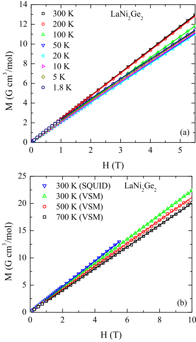
FIG. 21: (Color online) applied applied field H isotherms (symbols) at the listed temperatures for \text{LaNi}_2\text{Ge}_2 (a) using a SQUID magnetometer and (b) using a VSM magnetometer. The solid curves of the corresponding colors are fits by Eq. (19).
